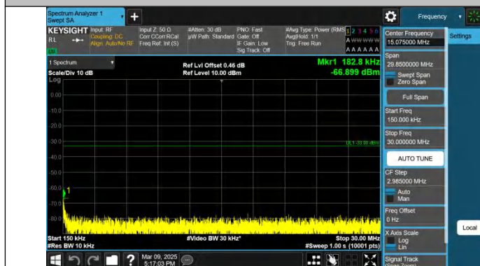
Band4-3MHz-QPSK-19965-1RB#14-0.15~30-PASS
