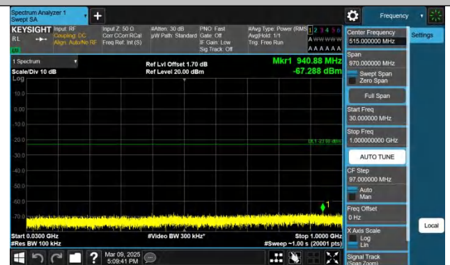
Band4-1.4MHz-QPSK-20393-1RB#5-30~1000-PASS
