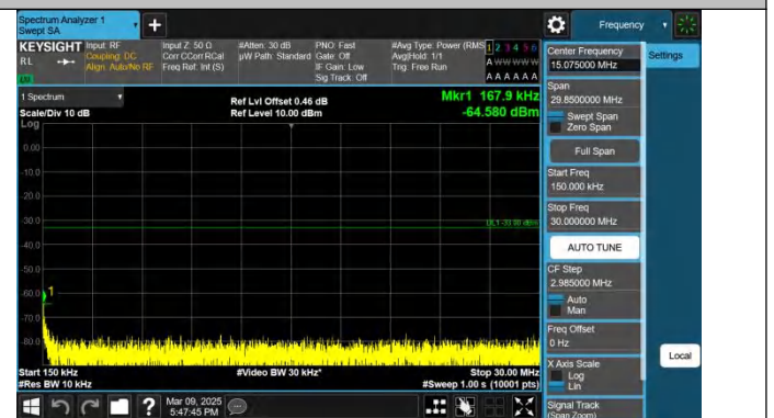
Band4-15MHz-QPSK-20175-1RB#0-0.15~30-PASS
