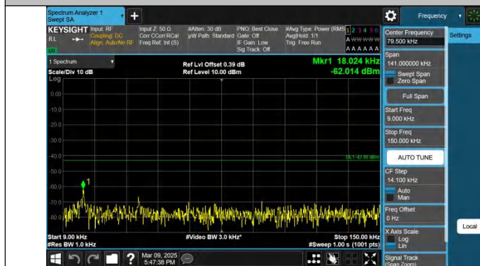
Band4-15MHz-QPSK-20175-1RB#0-0.009~0.15-PASS
