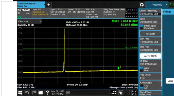
Band4-15MHz-QPSK-20025-1RB#74-1000~3000-PASS
