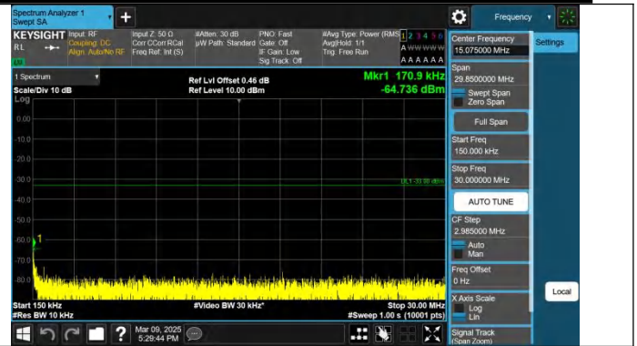
Band4-5MHz-QPSK-20375-1RB#0-0.15~30-PASS
