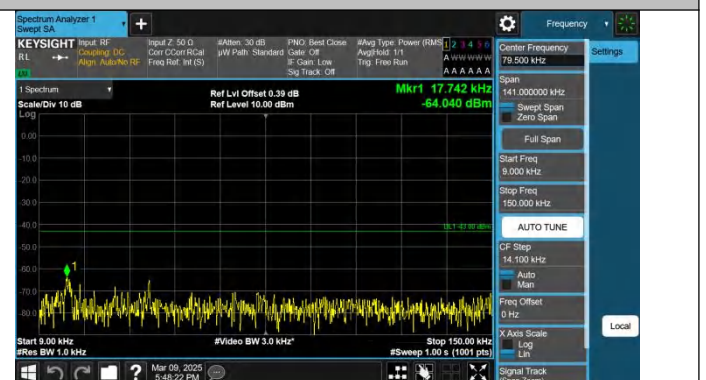
Band4-15MHz-QPSK-20175-1RB#74-0.009~0.15-PASS
