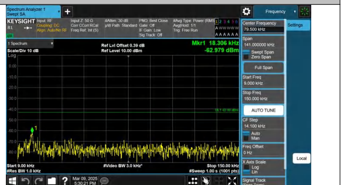
Band4-5MHz-QPSK-20375-1RB#24-0.009~0.15-PASS
