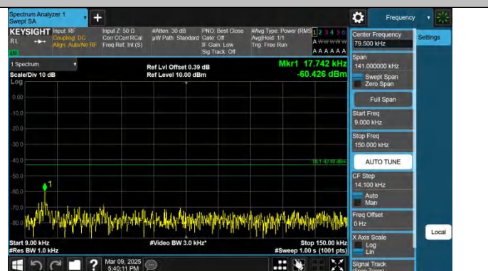
Band4-10MHz-QPSK-20350-1RB#49-0.009~0.15-PASS
