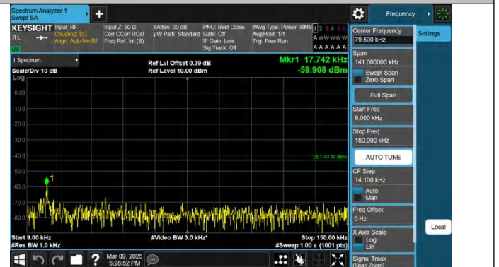
Band4-5MHz-QPSK-20175-1RB#24-0.009~0.15-PASS
