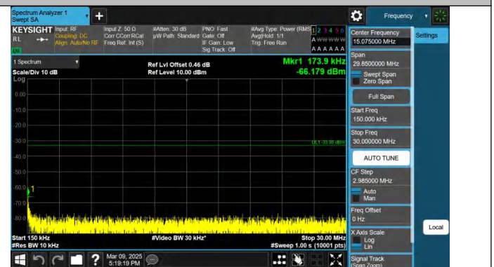
Band4-3MHz-QPSK-20385-1RB#0-0.15~30-PASS
