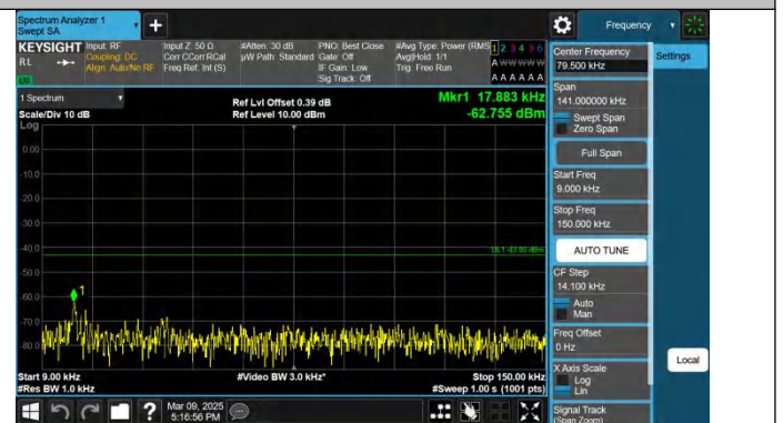
Band4-3MHz-QPSK-19965-1RB#14-0.009~0.15-PASS
