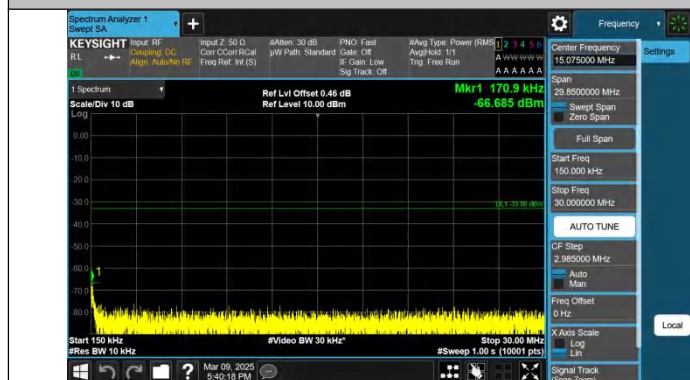
Band4-10MHz-QPSK-20350-1RB#49-0.15~30-PASS
