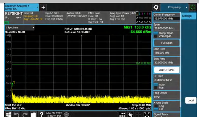
Band4-3MHz-QPSK-19965-1RB#0-0.15~30-PASS
