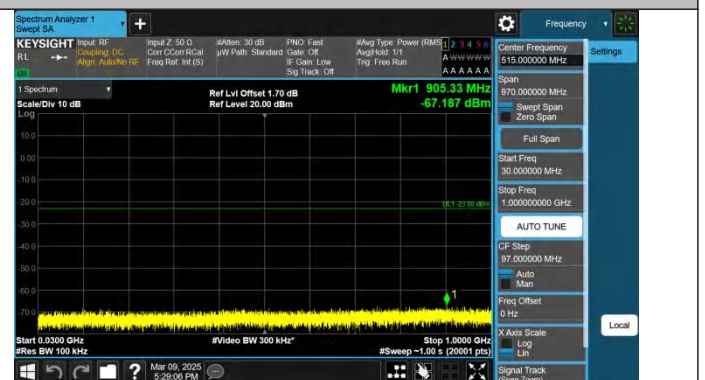
Band4-5MHz-QPSK-20175-1RB#24-30~1000-PASS
