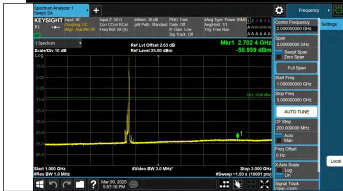
Band4-20MHz-QPSK-20175-1RB#99-1000~3000-PASS
