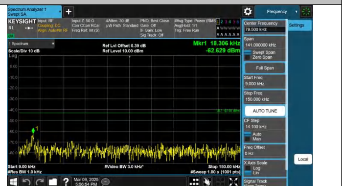
Band4-20MHz-QPSK-20175-1RB#99-0.009~0.15-PASS
