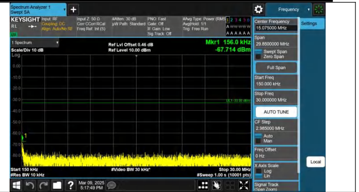
Band4-3MHz-QPSK-20175-1RB#0-0.15~30-PASS
