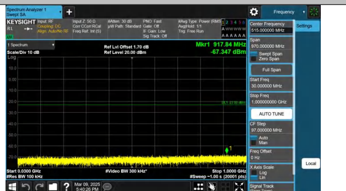
Band4-10MHz-QPSK-20350-1RB#49-30~1000-PASS
