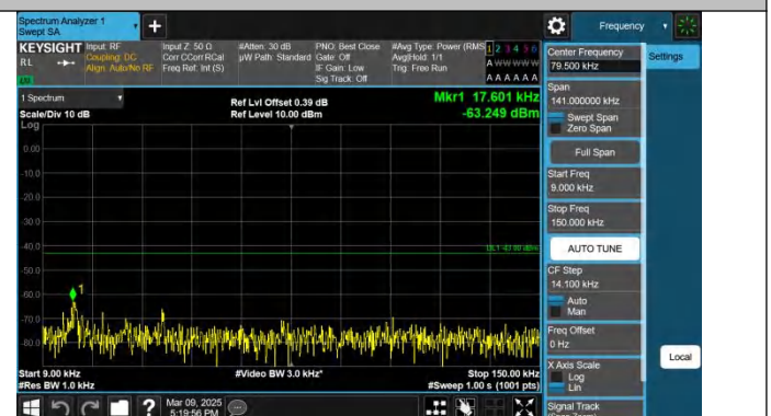
Band4-3MHz-QPSK-20385-1RB#14-0.009~0.15-PASS
