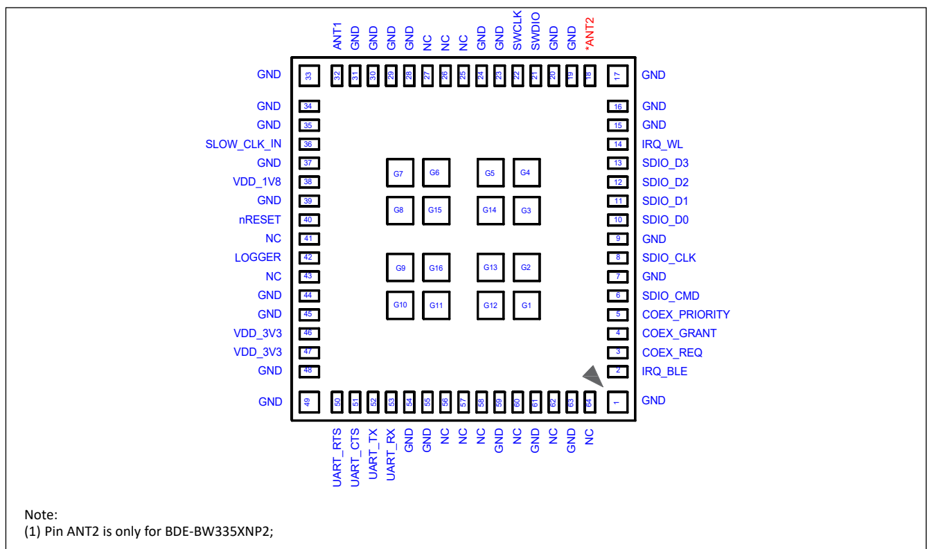
Figure 5. Pin Diagram of BDE-BW335XNP1 and BDE-BW335XNP2 (Top View)
