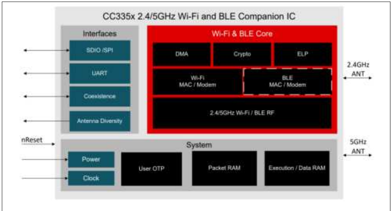
Figure 4. The block diagram of CC3351 (Adopted from CC3351 Datasheet)
