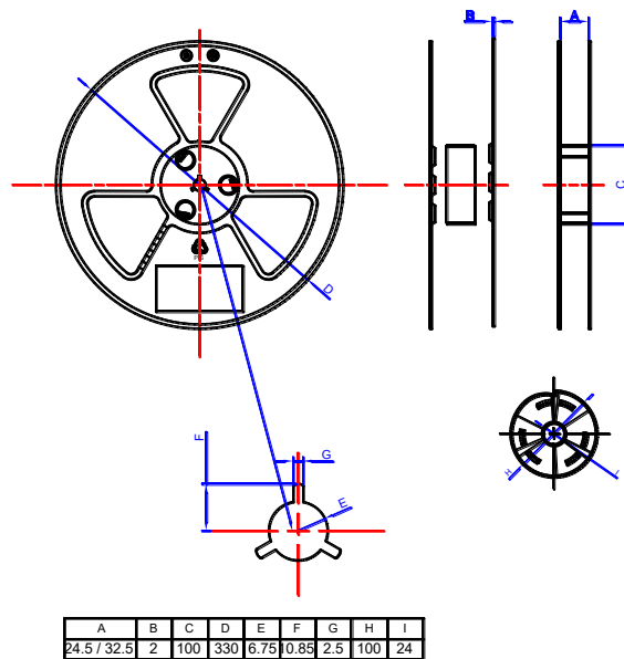
Figure 20. Carrier Tape Drawing for BDE-BW335XUPX and BDE-BW335XAP1 variants
