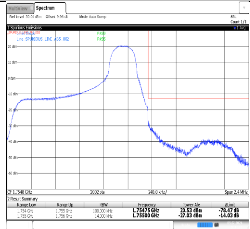
Band4-1.4MHz-16QAM-20393-1RB#5-PASS
