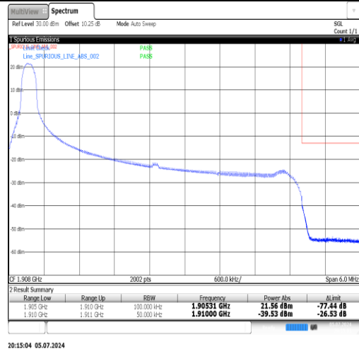
Band2-5MHz-QPSK-19175-1RB#24-PASS
