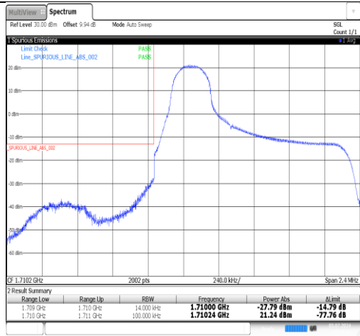
Band4-1.4MHz-16QAM-19957-1RB#5-PASS
