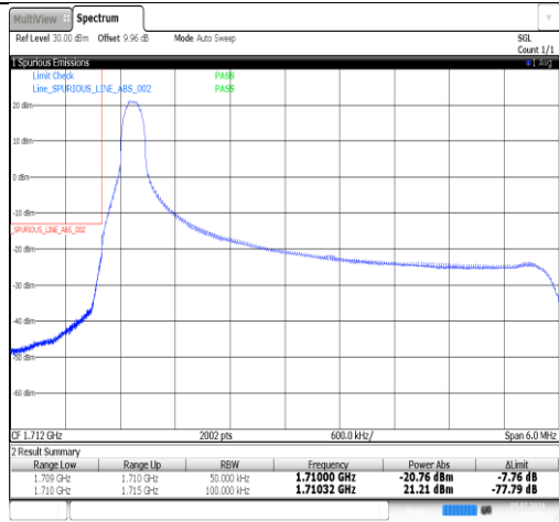
Band4-5MHz-QPSK-19975-1RB#24-PASS
