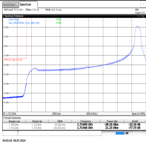
Band4-5MHz-QPSK-20375-25RB#0-PASS
