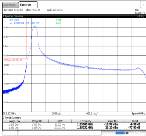
Band2-5MHz-16QAM-18625-1RB#24-PASS
