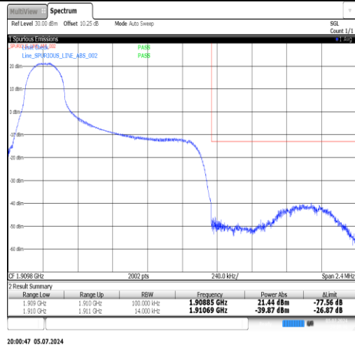
Band2-1.4MHz-16QAM-19193-1RB#5-PASS
