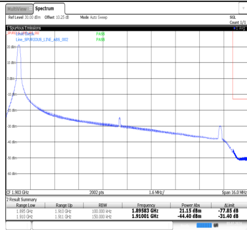
Band2-15MHz-QPSK-19125-1RB#74-PASS
