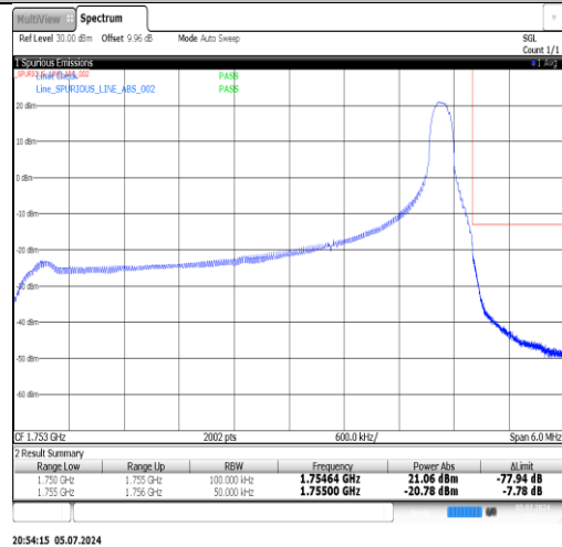
Band4-5MHz-16QAM-19975-25RB#0-PASS
