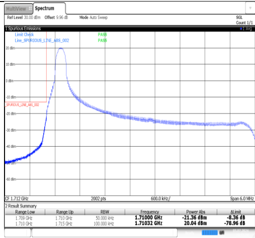
Band4-5MHz-16QAM-19975-1RB#24-PASS
