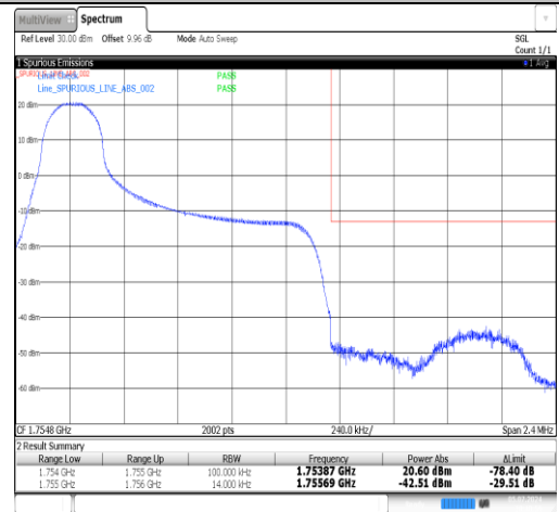
Band4-1.4MHz-16QAM-20393-1RB#0-PASS
