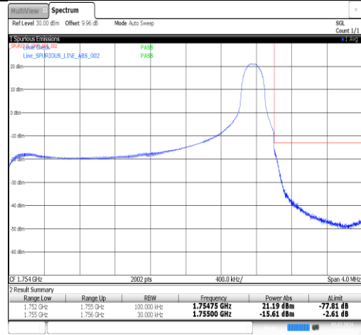
Band4-3MHz-QPSK-20385-1RB#14-PASS
