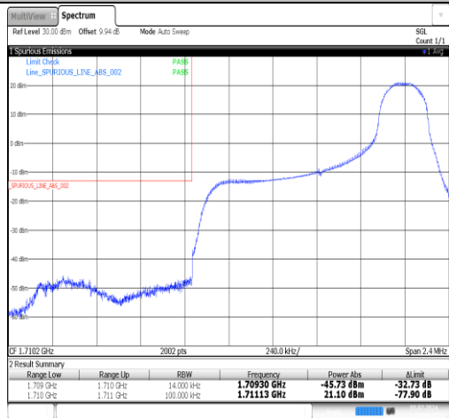
Band4-1.4MHz-16QAM-19957-1RB#5-PASS
