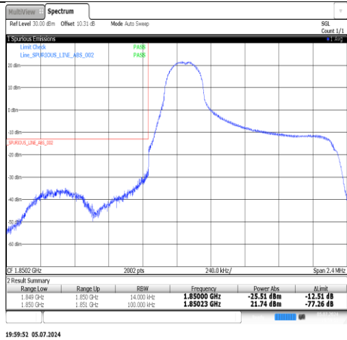
Band2-1.4MHz-16QAM-18607-1RB#5-PASS
