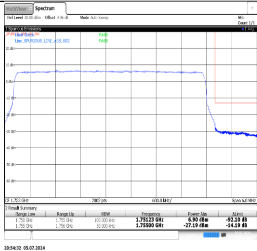
Band4-5MHz-16QAM-19975-1RB#0-PASS
