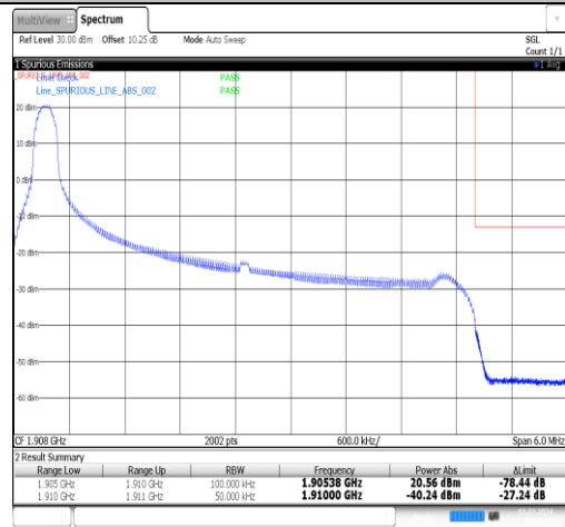
Band2-5MHz-16QAM-19175-1RB#24-PASS
