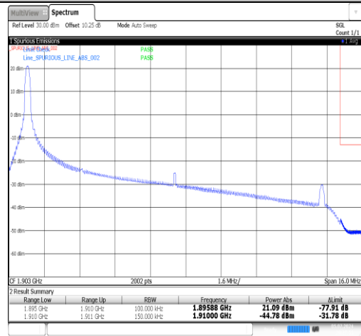
Band2-15MHz-16QAM-19125-1RB#74-PASS
