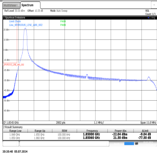
Band2-10MHz-16QAM-18650-1RB#49-PASS
