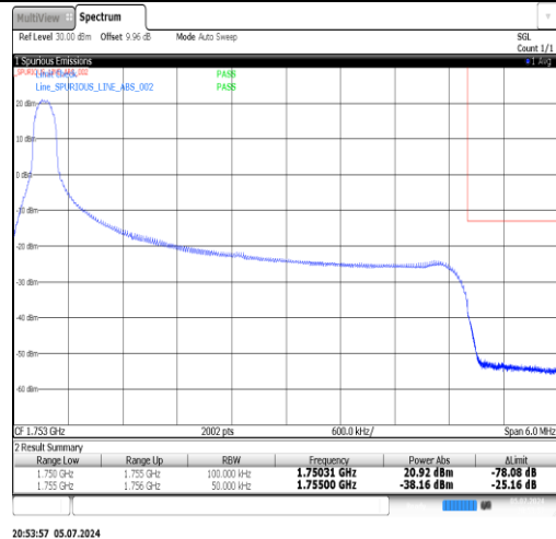
Band4-5MHz-QPSK-20375-1RB#24-PASS
