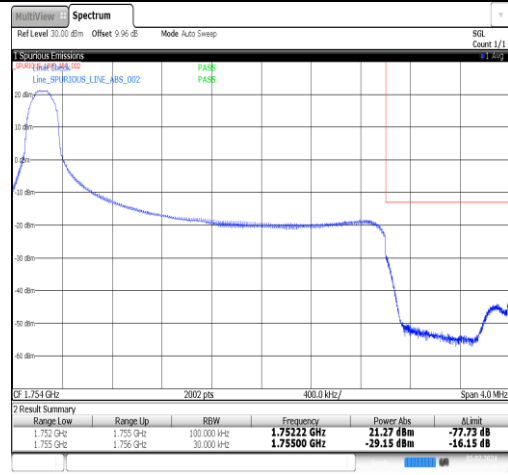
Band4-3MHz-QPSK-20385-1RB#14-PASS
