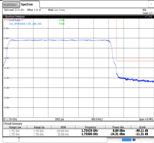
Band4-3MHz-QPSK-20385-15RB#0-PASS
