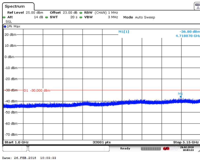
Figure 293 Spurious Emissions (1 GHz – 5.15 GHz) – 64QAM (5200.0/ 5220.0/ 5240.0 MHz) (3 X 20MHz Channel BW)
