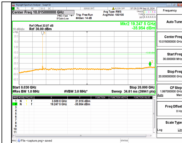
n77(3450-3550MHz) (30MHz-20GHz) 60M DFT-s-OFDM QPSK Inner_1RB_Right Low
