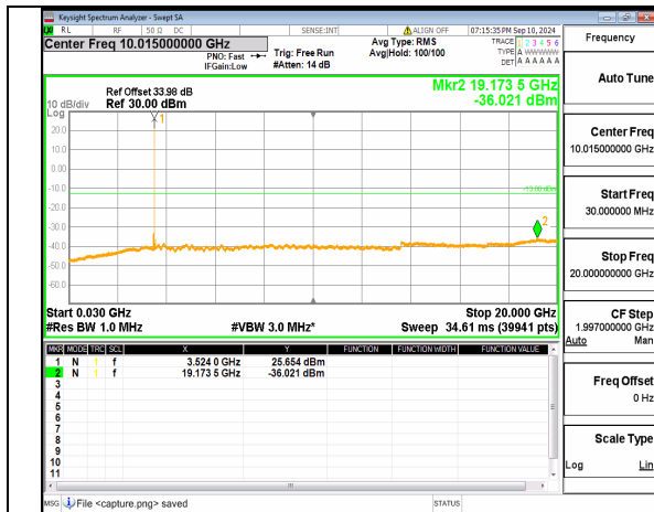
n77(3450-3550MHz) (30MHz-20GHz) 50M DFT-s-OFDM BPSK Inner_1RB_Right Mid
