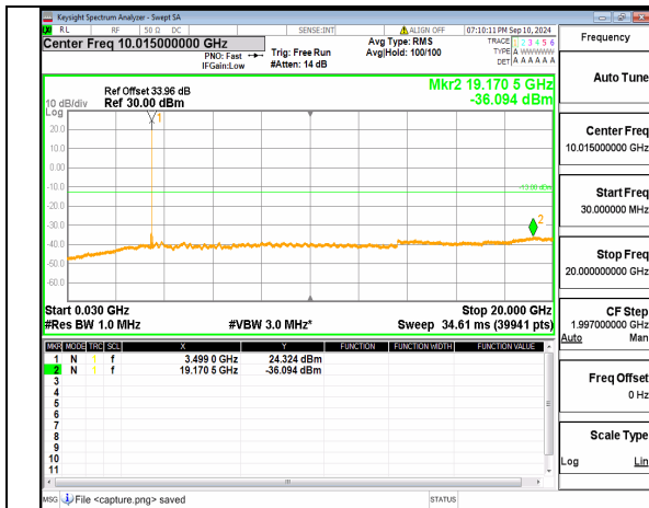
n77(3450-3550MHz) (30MHz-20GHz) 50M DFT-s-OFDM BPSK Inner_1RB_Right Low
