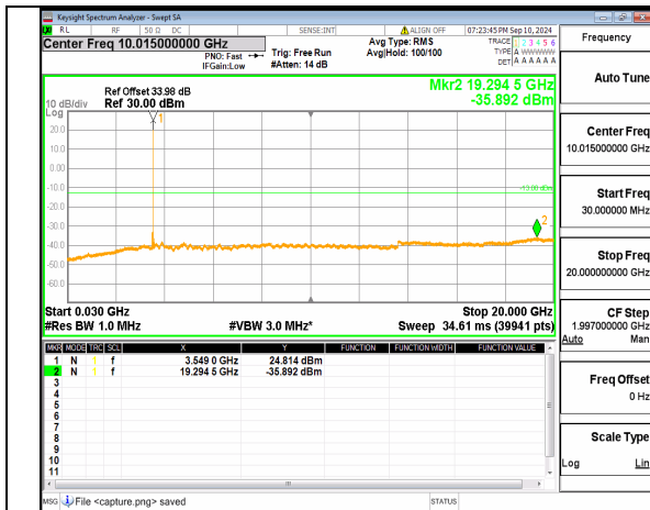
n77(3450-3550MHz) (30MHz-20GHz) 50M DFT-s-OFDM QPSK Inner_1RB_Right_High
