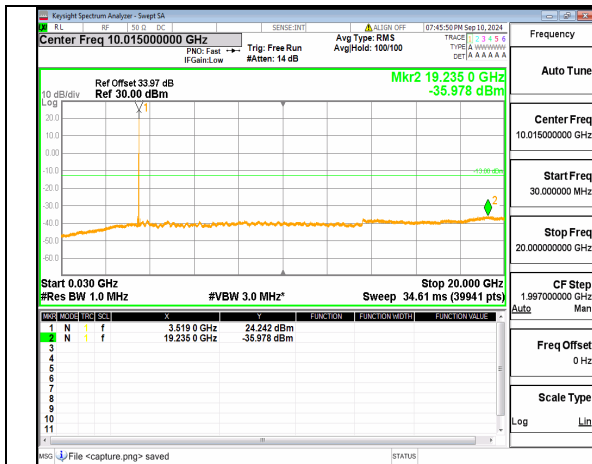
n77(3450-3550MHz) (30MHz-20GHz) 70M DFT-s-OFDM QPSK Inner_1RB_Right Low
