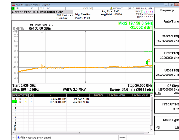
n77(3450-3550MHz) (30MHz-20GHz) 50M DFT-s-OFDM QPSK Inner_1RB_Right Mid
