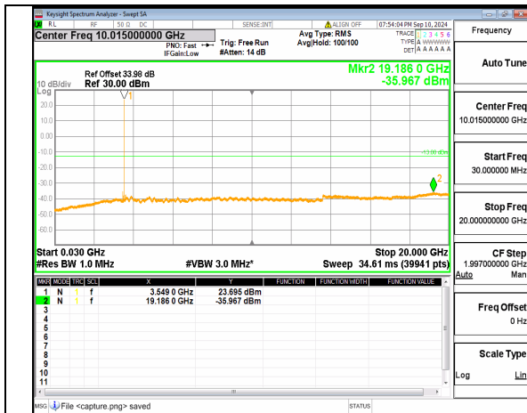
n77(3450-3550MHz) (30MHz-20GHz) 70M DFT-s-OFDM BPSK Inner_1RB_Right High
