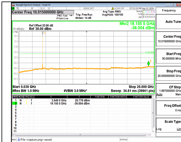
n77(3450-3550MHz) (30MHz-20GHz) 50M DFT-s-OFDM BPSK Inner_1RB_Right High
