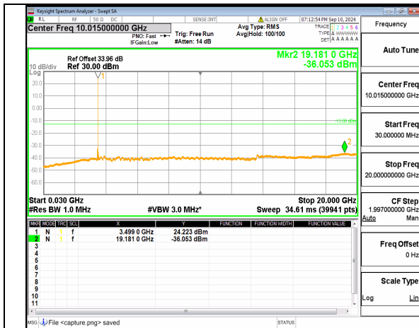
n77(3450-3550MHz) (30MHz-20GHz) 50M DFT-s-OFDM QPSK Inner_1RB_Right Low
