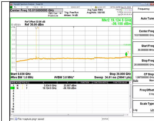
n77(3450-3550MHz) (30MHz-20GHz) 70M DFT-s-OFDM QPSK Inner_1RB_Right Mid
