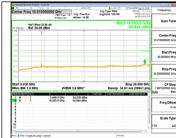
n77(3450-3550MHz) (30MHz-20GHz) 70M DFT-s-OFDM QPSK Inner_1RB_Right_High
