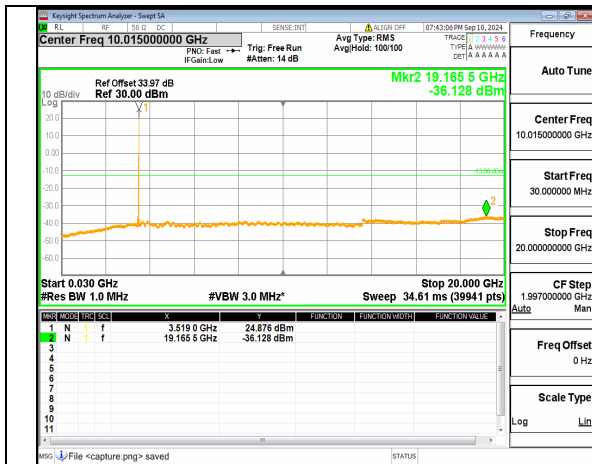
n77(3450-3550MHz) (30MHz-20GHz) 70M DFT-s-OFDM BPSK Inner_1RB_Right Low
