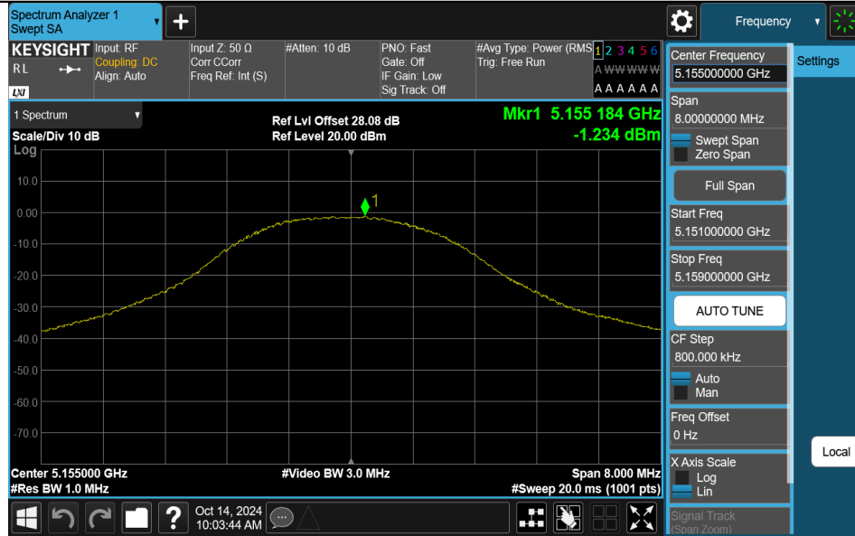
GFSK-Ant2-5155-PASS
