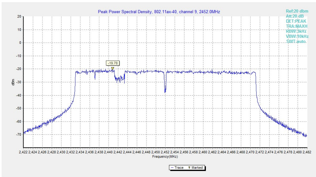
Fig.A.3.36 Power Spectral Density (802.11ax-HE40, Ch 9)
