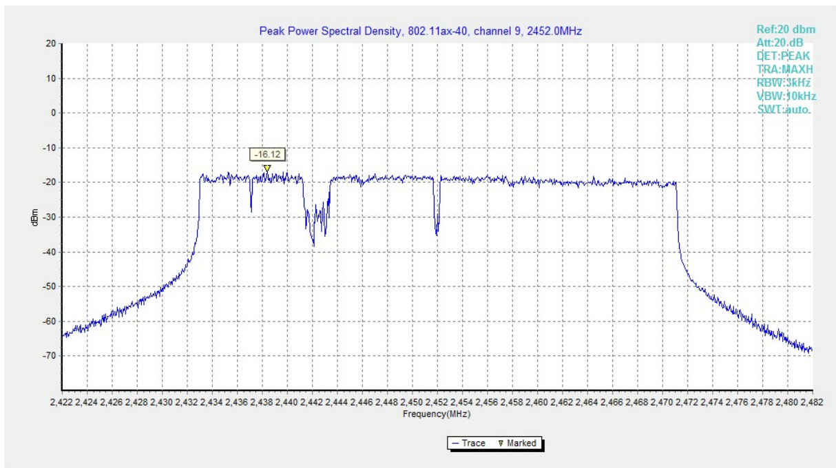
Fig.A.3.18 Power Spectral Density (802.11ax-HE40, Ch 9)
