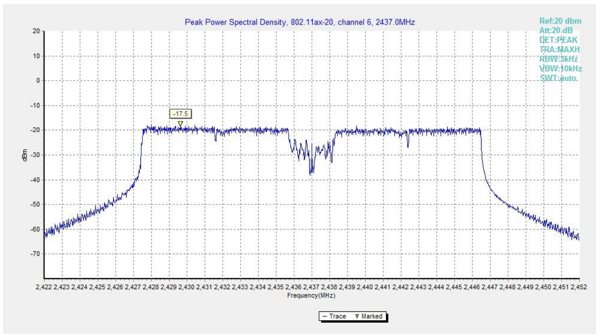
Fig.A.3.50 Power Spectral Density (802.11ax-HE20, Ch 6)
