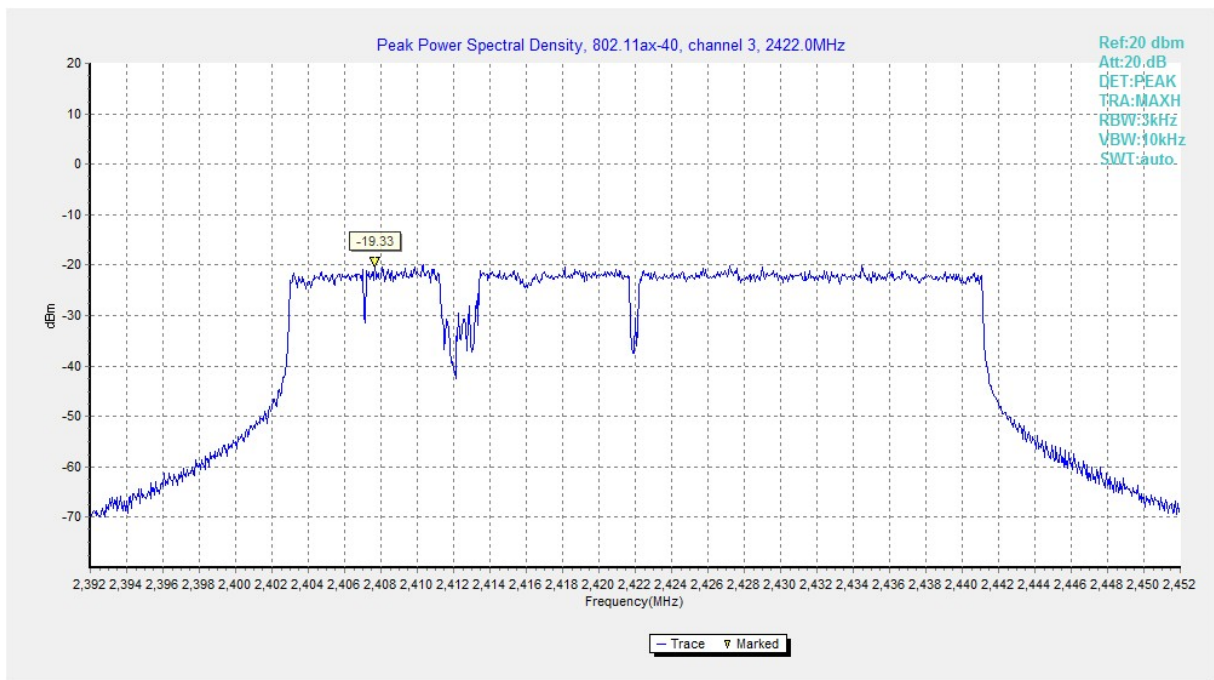
Fig.A.3.34 Power Spectral Density (802.11ax-HE40, Ch 3)
