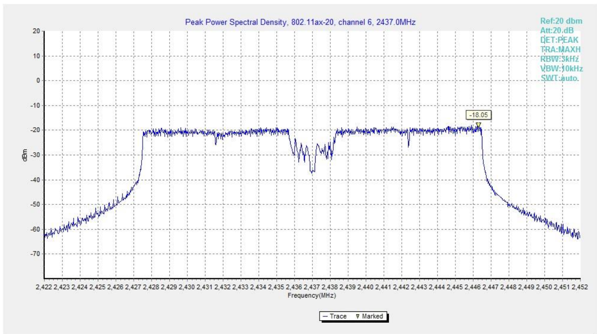
Fig.A.3.32 Power Spectral Density (802.11ax-HE20, Ch 6)
