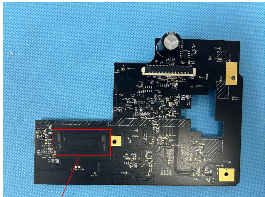
BT 2 Antenna
