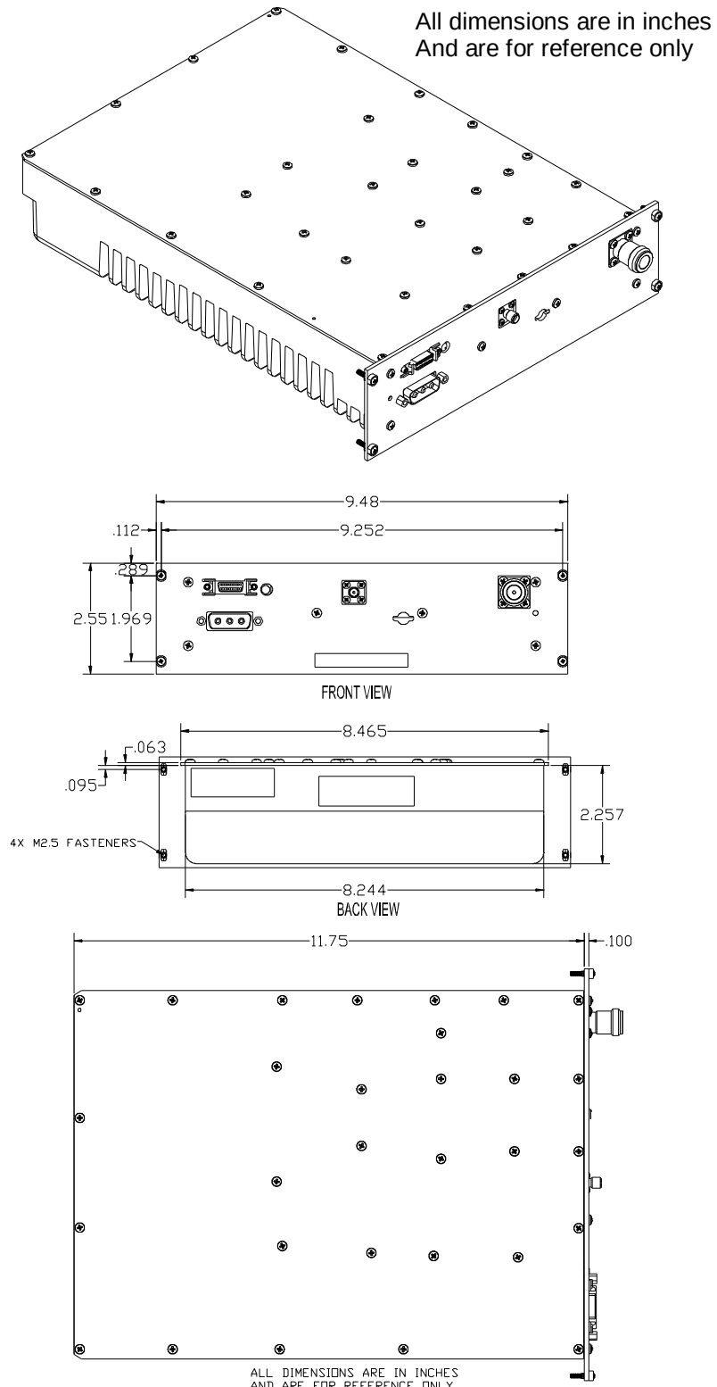
Figure 1-1. SCA 9321-30C Amplifier
