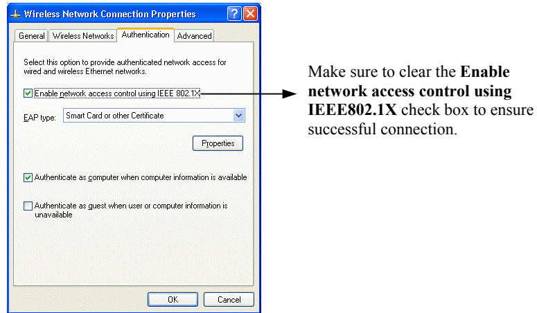
Figure 3-10 Windows XP Connection Properties -Authentication
