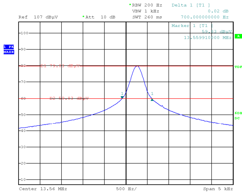
20dB Bandwidth
