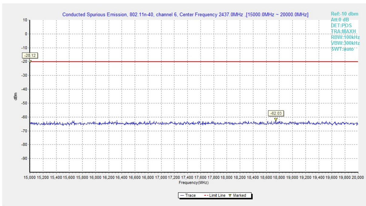
Fig.A.6.1.87 Conducted Spurious Emission (802.11n-HT40, Ch6, 15 GHz-20 GHz)
