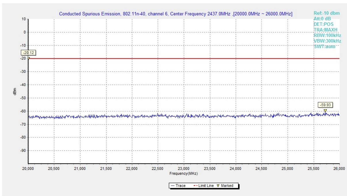
Fig.A.6.1.88 Conducted Spurious Emission (802.11n-HT40, Ch6, 20 GHz-26 GHz)
