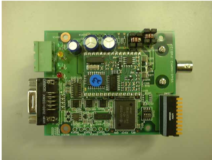
Upper Circuit Board (Front)
