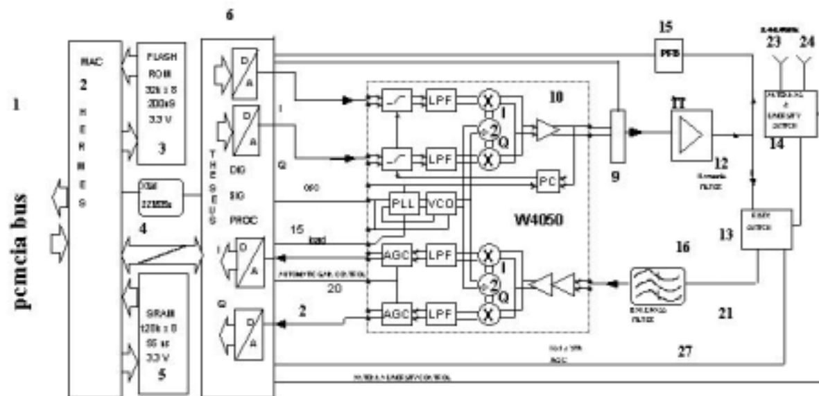
Block diagram Agere 2.4 GHz ORINOCO (WaveLAN)
