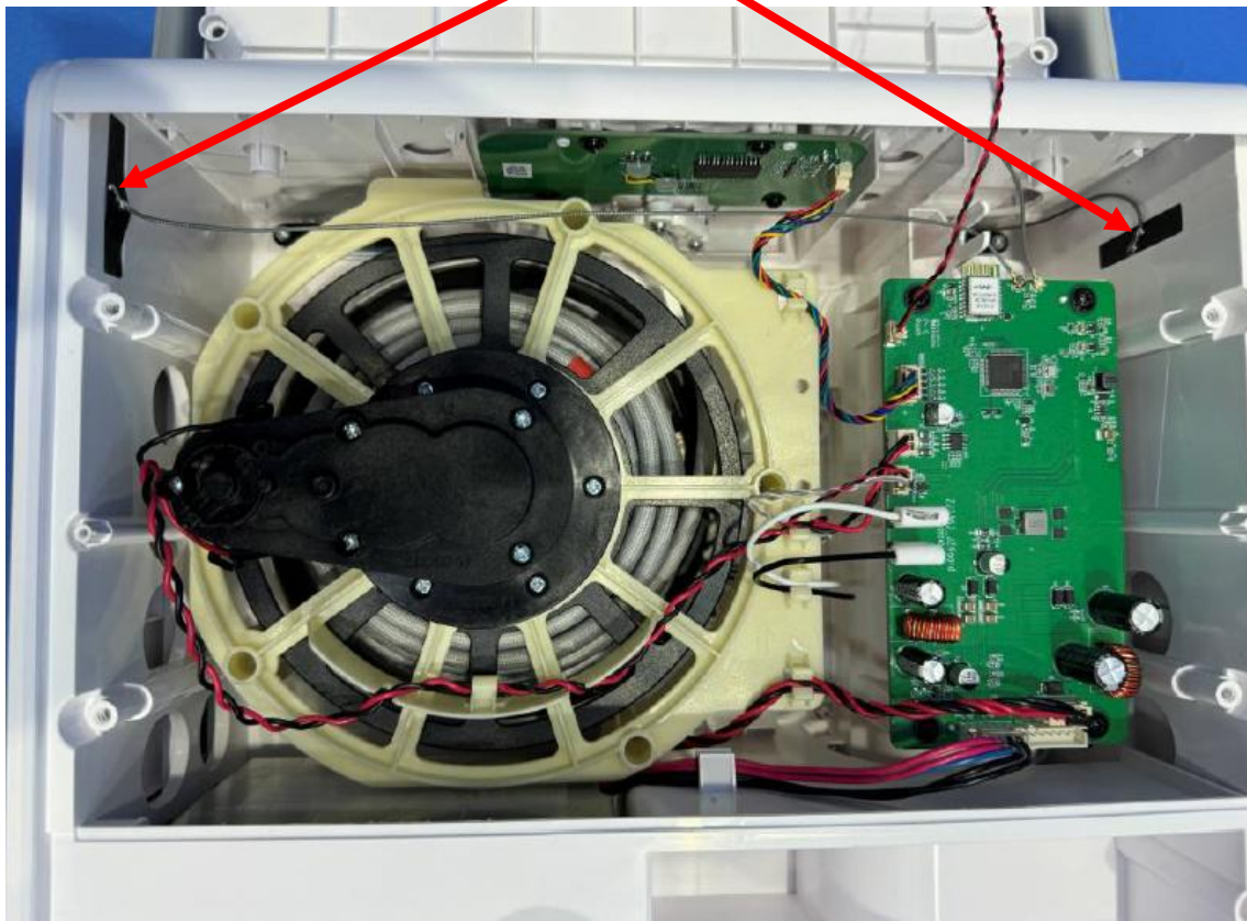
Antenna 1 Antenna 2 of station
