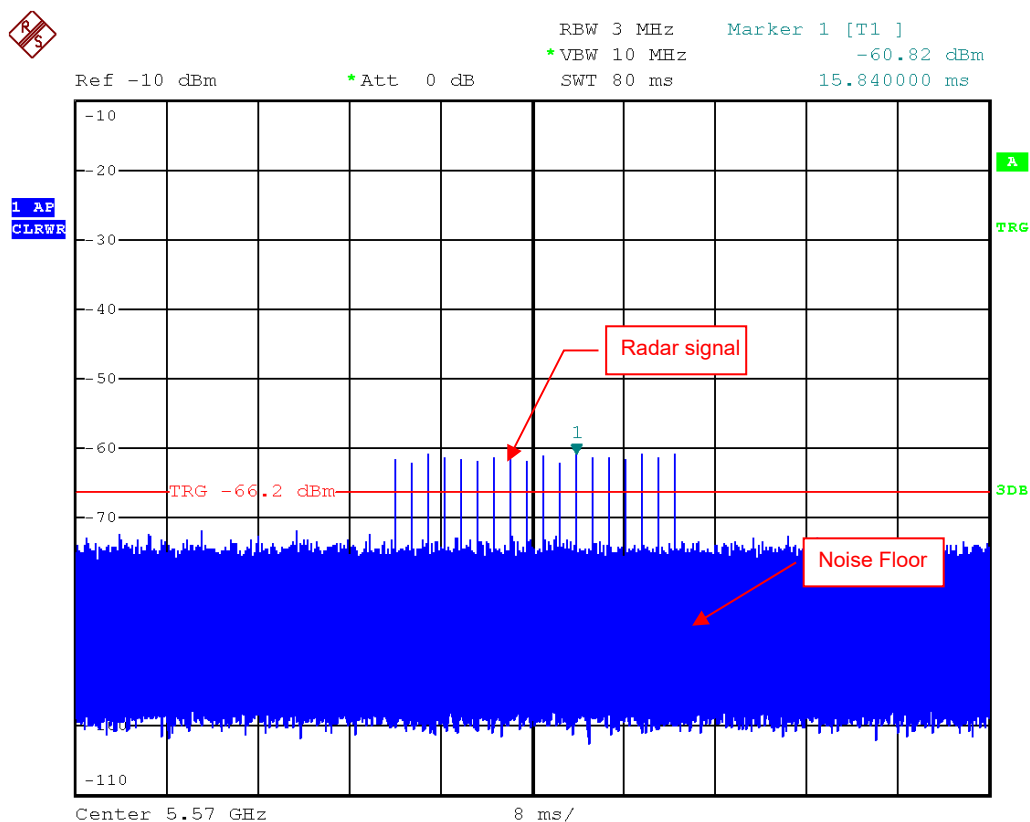
Radar Signal 0
