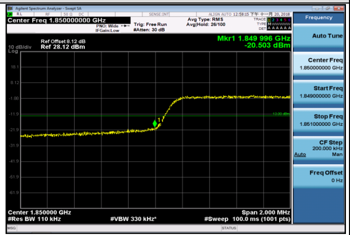
LCH_16QAM_15RB#0
