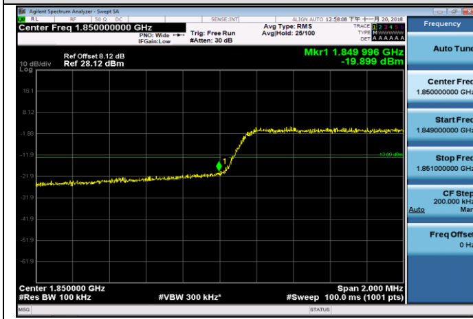
LCH_QPSK_15RB#0
