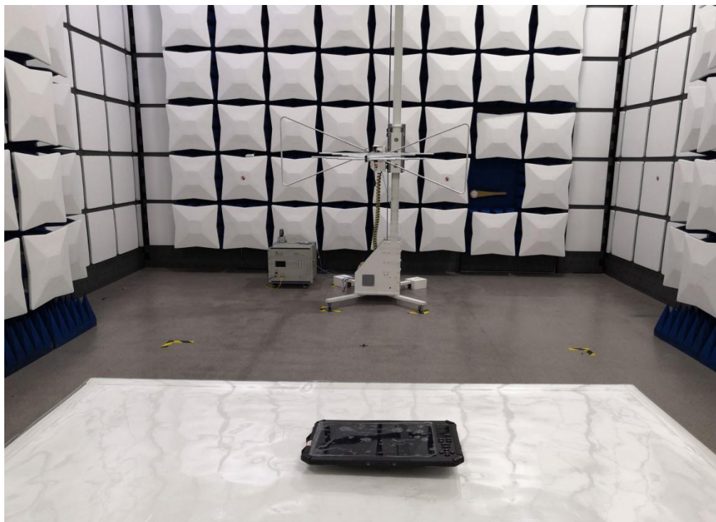
RADIATED SPURIOUS ABOVE 1G EMISSION
