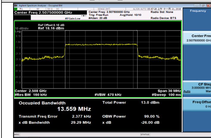
LCH_QPSK_75RB#0
