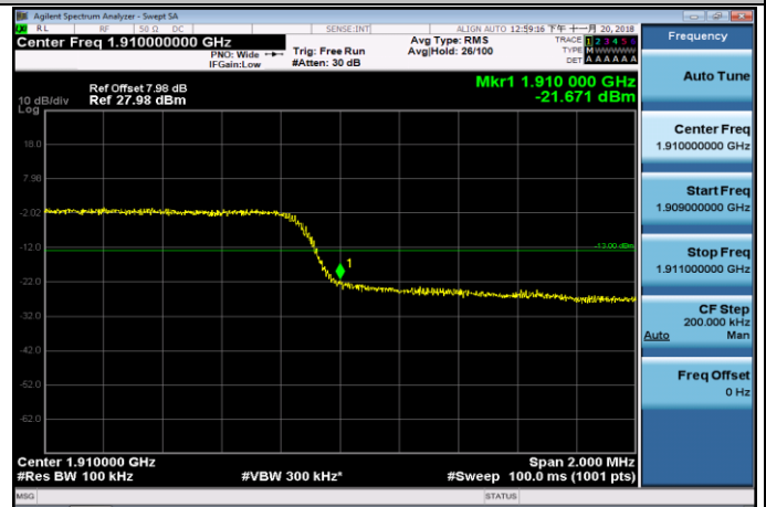
HCH_16QAM_15RB#0
