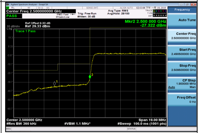
LCH_16QAM_50RB#0
