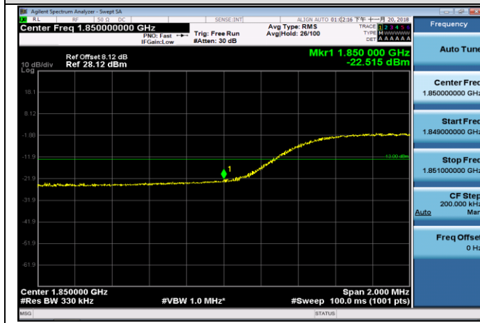
LCH_QPSK_50RB#0
