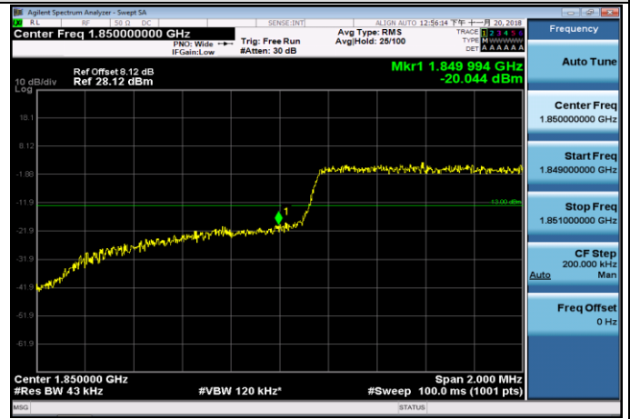
LCH_16QAM_6RB#0
