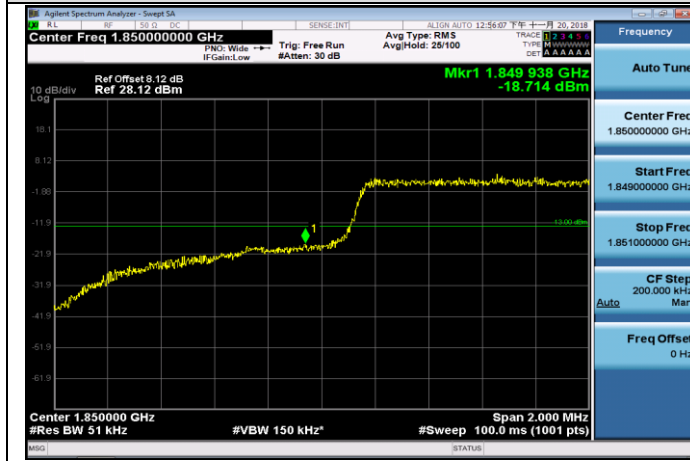
LCH_QPSK_6RB#0
