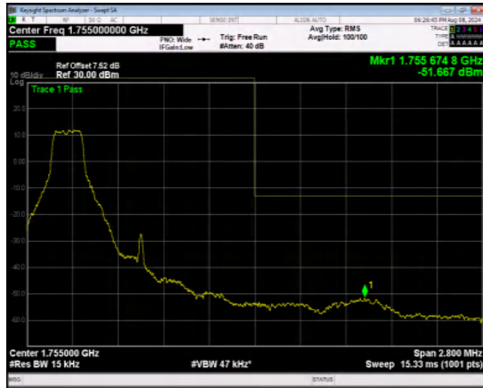
Band4 16QAM BW=1.4MHz Channel=20393 RB Size=1 Position=#Max Extended
