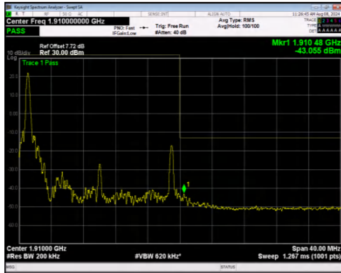
Band2 QPSK BW=20MHz Channel=19100 RB Size=1 Position=#Max Extended
