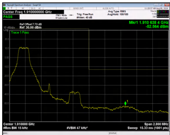
Band2 16QAM BW=1.4MHz Channel=19193 RB Size=1 Position=#Max Extended
