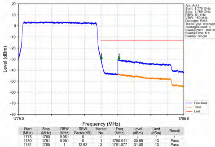
Band66_5MHz_QPSK_HCH_1777.5MHz_RB_25_0_NTNV
