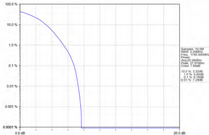
Band66_1.4MHz_64QAM_MCH_1745MHz_RB_6_0_NTNV
