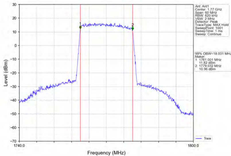
Band66_20MHz_64QAM_HCH_1770MHz_RB_100_0_NTNV
