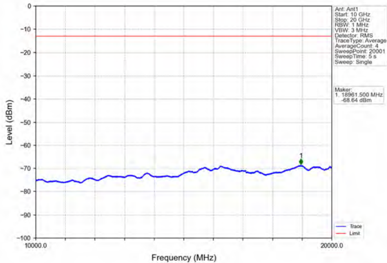
Band66_15MHz_64QAM_LCH_1717.5MHz_RB_75_0_NTNV
