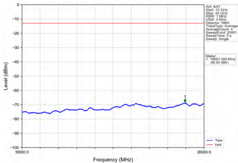
Band66_20MHz_16QAM_MCH_1745MHz_RB_1_0_NTNV
