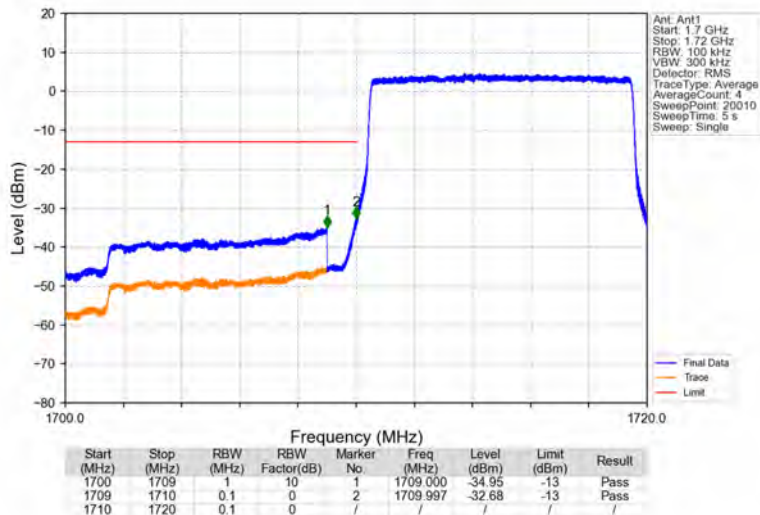
Band66_10MHz_QPSK_LCH_1715MHz_RB_50_0_NTNV
