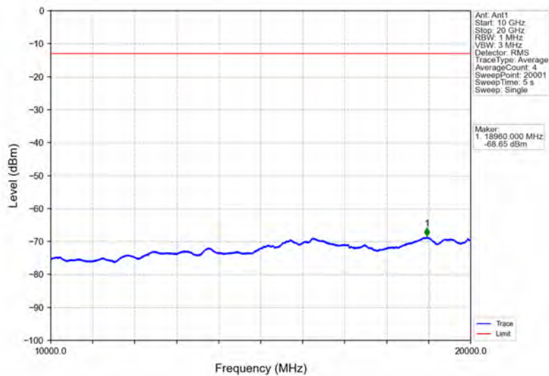
Band66_10MHz_16QAM_HCH_1775MHz_RB_1_0_NTNV
