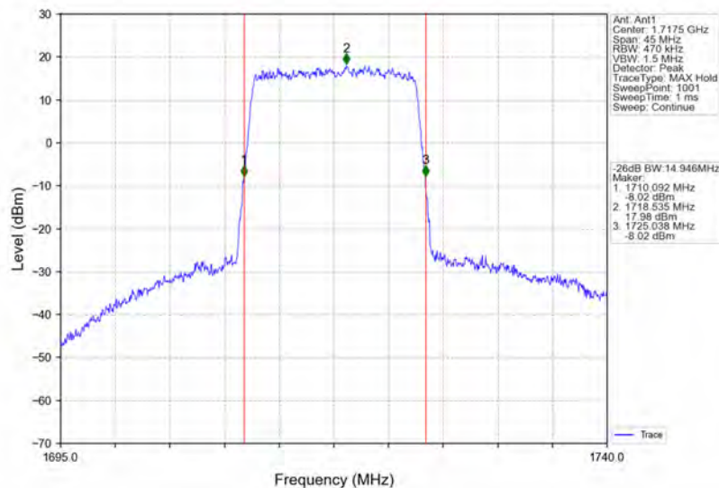
Band66_15MHz_16QAM_LCH_1717.5MHz_RB_75_0_NTNV
