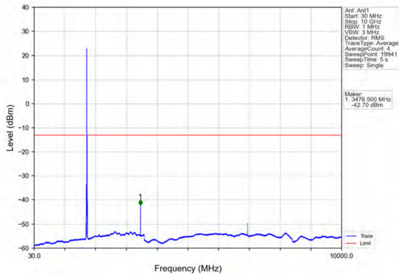
Band66_15MHz_16QAM_MCH_1745MHz_RB_1_0_NTNV
