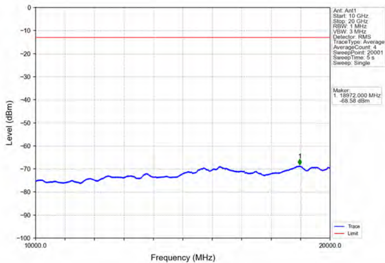
Band66_3MHz_QPSK_MCH_1745MHz_RB_1_0_NTNV
