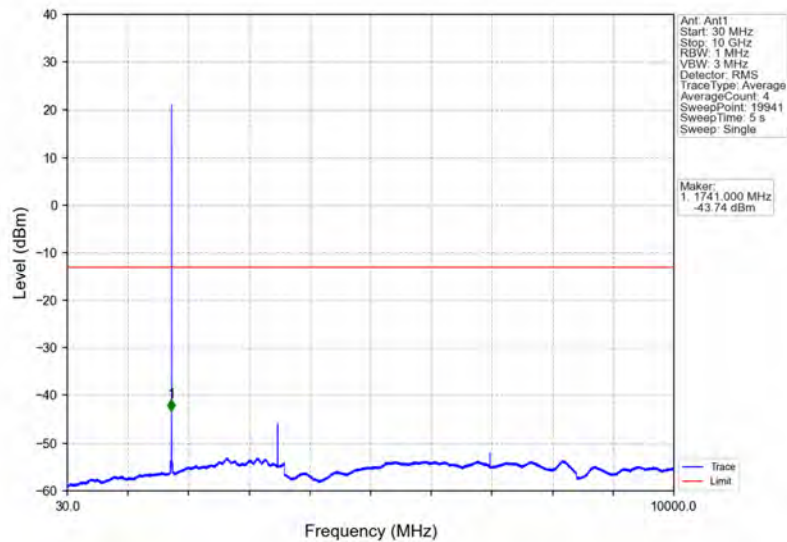
Band66_1.4MHz_64QAM_MCH_1745MHz_RB_1_0_NTNV
