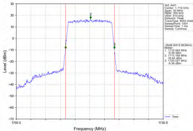
Band66_10MHz_64QAM_LCH_1715MHz_RB_50_0_NTNV
