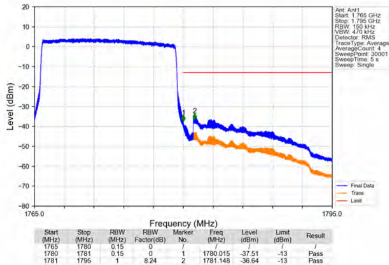
Band66_15MHz_QPSK_HCH_1772.5MHz_RB_75_0_NTNV
