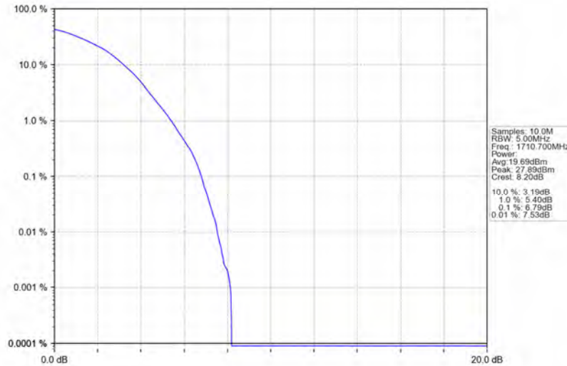
Band66_1.4MHz_64QAM_LCH_1710.7MHz_RB_6_0_NTNV
