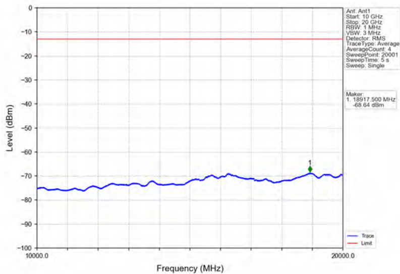
Band66_20MHz_64QAM_HCH_1770MHz_RB_1_0_NTNV
