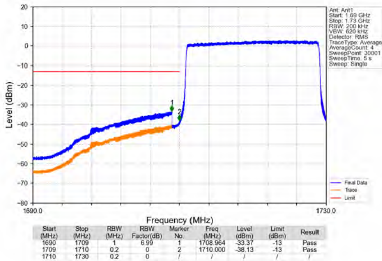
Band66_20MHz_64QAM_LCH_1720MHz_RB_100_0_NTNV
