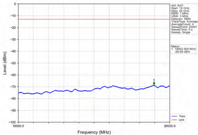
Band66_1.4MHz_16QAM_MCH_1745MHz_RB_1_0_NTNV
