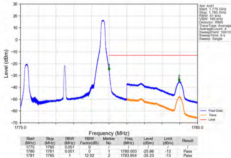
Band66_5MHz_16QAM_HCH_1777.5MHz_RB_1_24_NTNV
