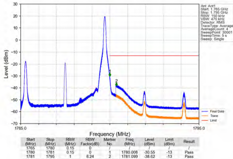
Band66_15MHz_16QAM_HCH_1772.5MHz_RB_1_74_NTNV
