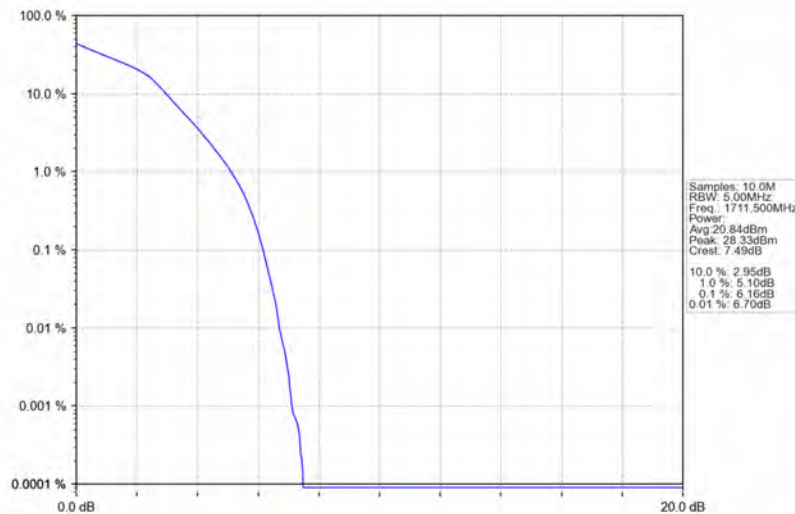
Band66_3MHz_16QAM_LCH_1711.5MHz_RB_15_0_NTNV
