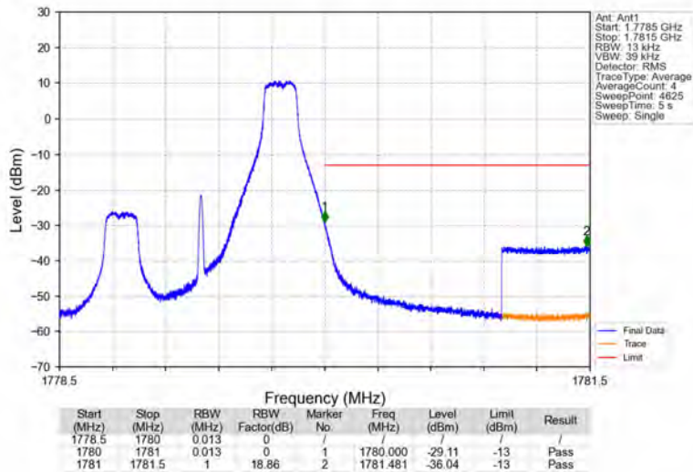
Band66_1.4MHz_64QAM_HCH_1779.3MHz_RB_1_5_NTNV
