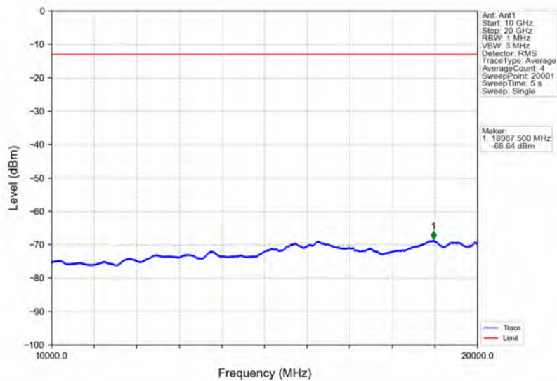
Band66_10MHz_64QAM_HCH_1775MHz_RB_1_0_NTNV
