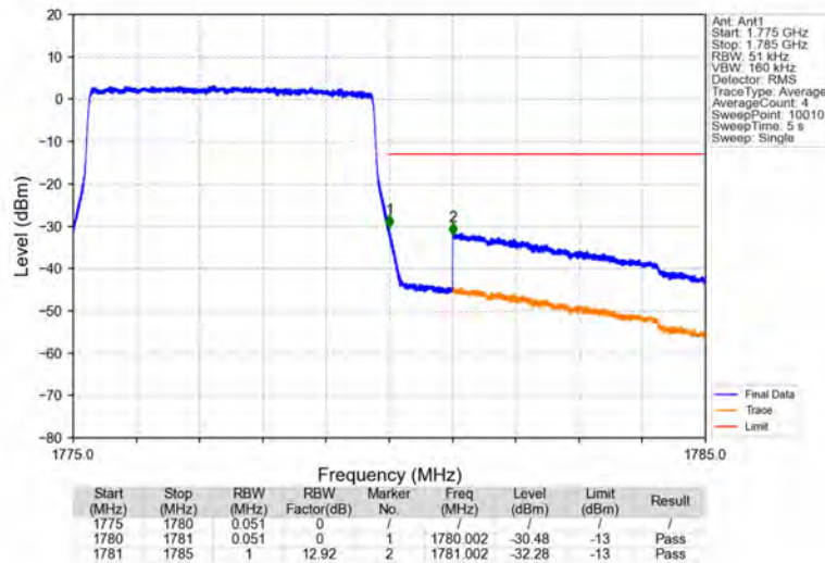
Band66_5MHz_16QAM_HCH_1777.5MHz_RB_25_0_NTNV
