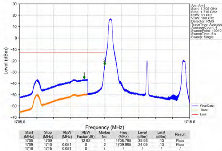
Band66_5MHz_16QAM_LCH_1712.5MHz_RB_1_0_NTNV
