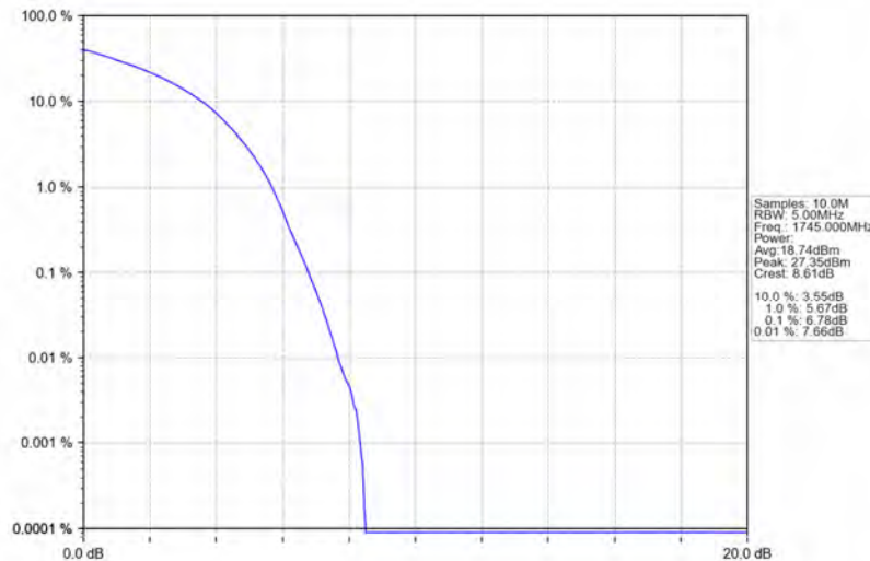
Band66_10MHz_16QAM_MCH_1745MHz_RB_50_0_NTNV
