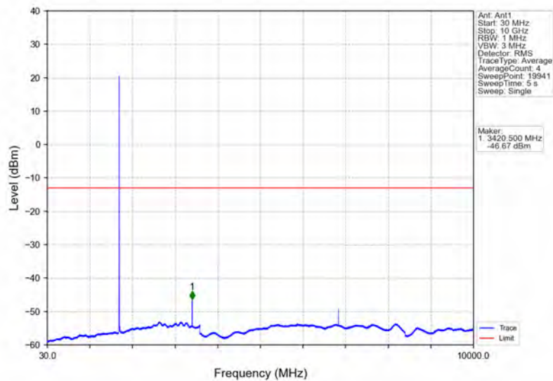
Band66_3MHz_64QAM_LCH_1711.5MHz_RB_1_0_NTNV
