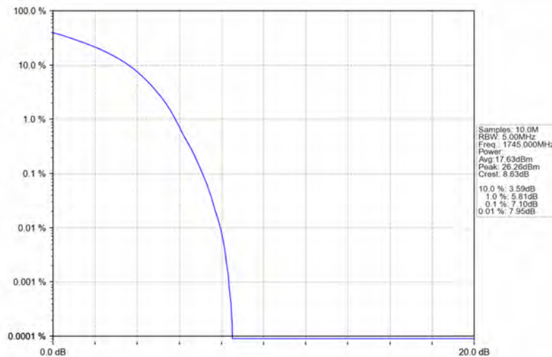
Band66_10MHz_64QAM_MCH_1745MHz_RB_50_0_NTNV
