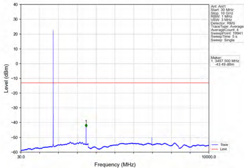
Band66_3MHz_QPSK_MCH_1745MHz_RB_1_0_NTNV
