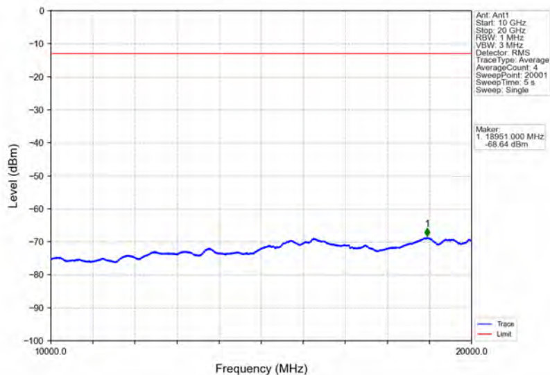
Band66_20MHz_64QAM_MCH_1745MHz_RB_1_0_NTNV
