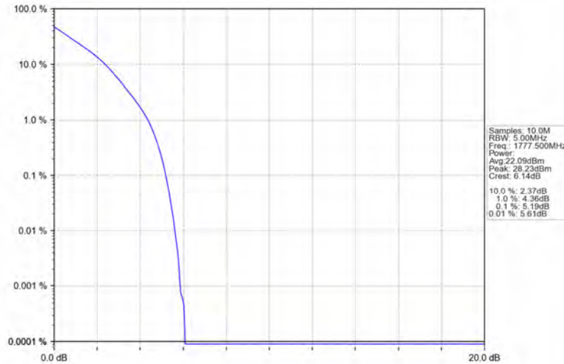
Band66_5MHz_QPSK_HCH_1777.5MHz_RB_25_0_NTNV
