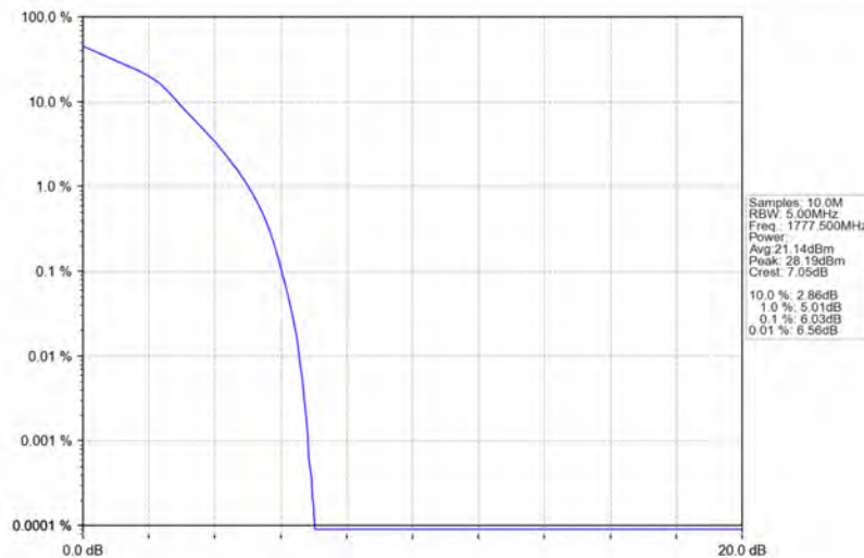
Band66_5MHz_16QAM_HCH_1777.5MHz_RB_25_0_NTNV
