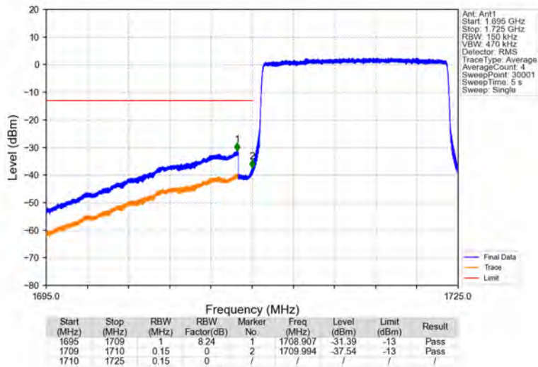
Band66_15MHz_64QAM_LCH_1717.5MHz_RB_75_0_NTNV
