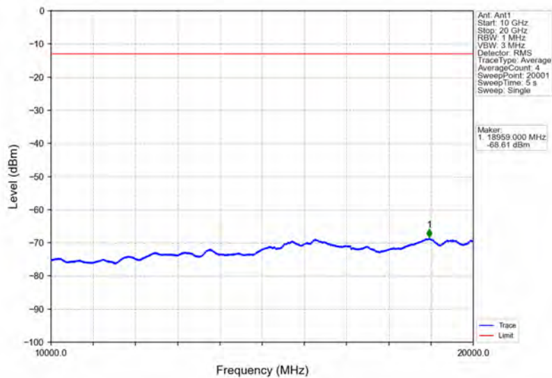
Band66_1.4MHz_16QAM_HCH_1779.3MHz_RB_1_0_NTNV
