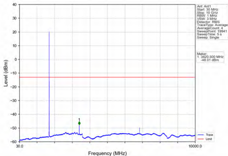
Band66_5MHz_64QAM_LCH_1712.5MHz_RB_1_0_NTNV
