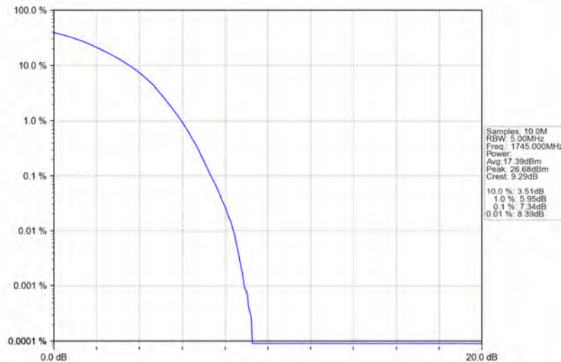
Band66_15MHz_16QAM_MCH_1745MHz_RB_75_0_NTNV
