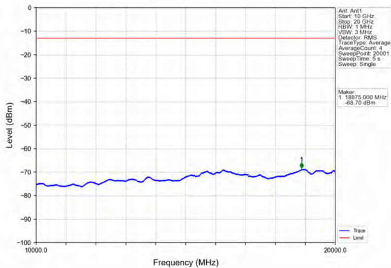
Band66_5MHz_64QAM_MCH_1745MHz_RB_1_0_NTNV
