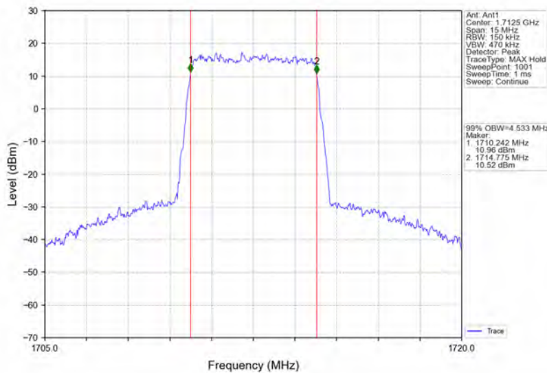
Band66_5MHz_16QAM_LCH_1712.5MHz_RB_25_0_NTNV
