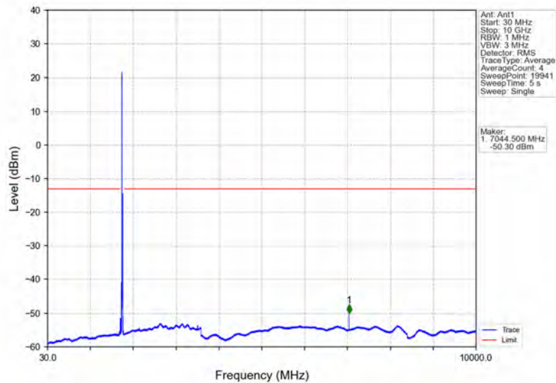
Band66_20MHz_16QAM_HCH_1770MHz_RB_1_0_NTNV
