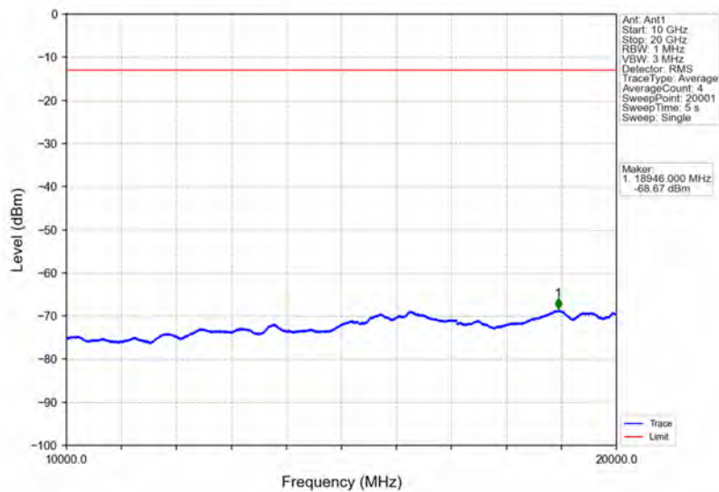
Band66_1.4MHz_64QAM_HCH_1779.3MHz_RB_1_0_NTNV
