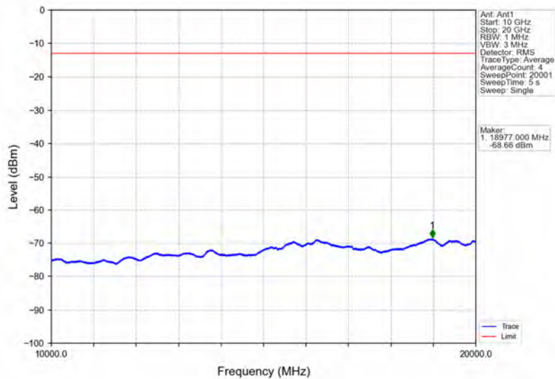
Band66_5MHz_16QAM_LCH_1712.5MHz_RB_25_0_NTNV
