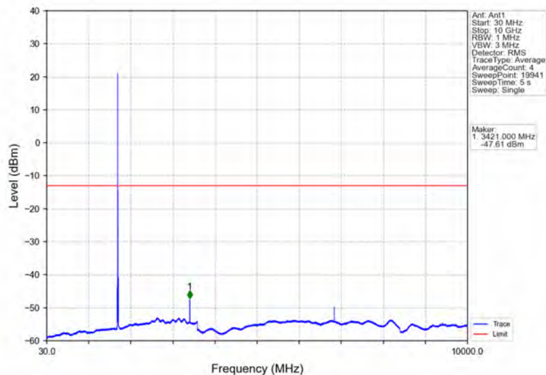
Band66_10MHz_64QAM_LCH_1715MHz_RB_1_0_NTNV
