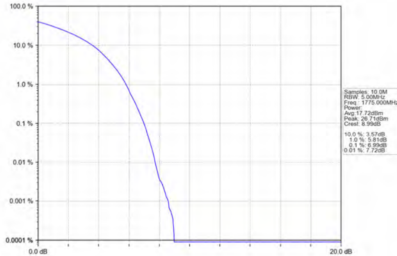
Band66_10MHz_64QAM_HCH_1775MHz_RB_50_0_NTNV
