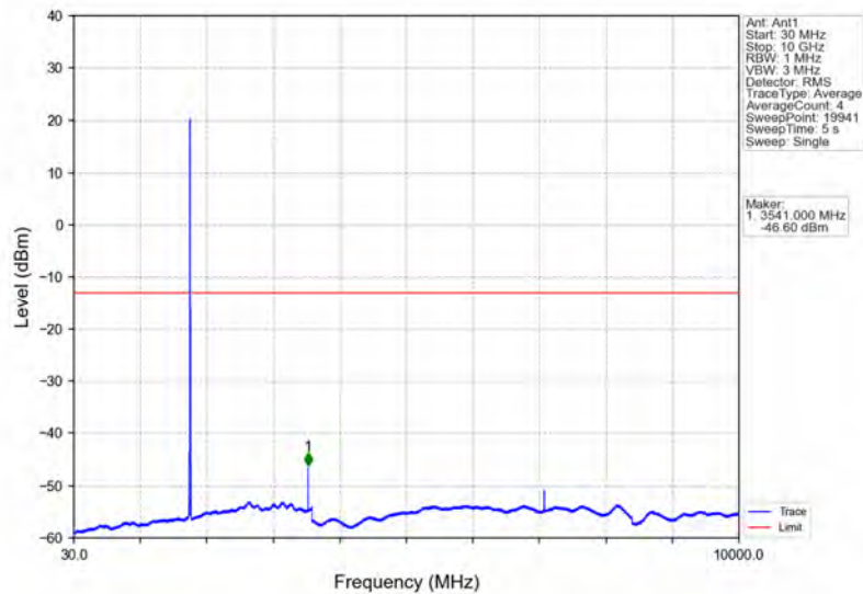
Band66_10MHz_64QAM_HCH_1775MHz_RB_1_0_NTNV
