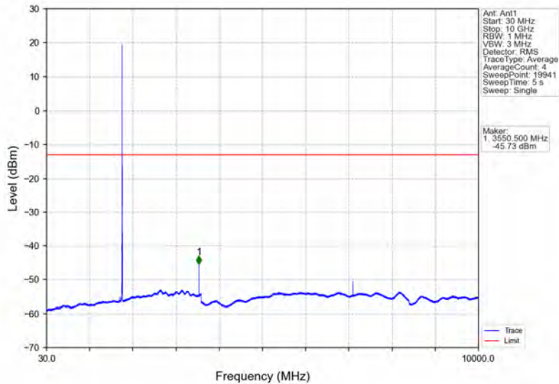
Band66_5MHz_64QAM_HCH_1777.5MHz_RB_1_0_NTNV
