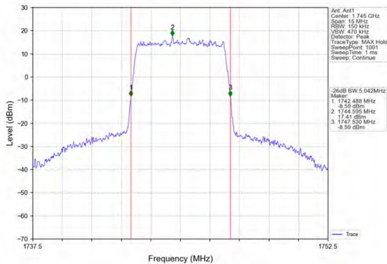
Band66_5MHz_64QAM_MCH_1745MHz_RB_25_0_NTNV
