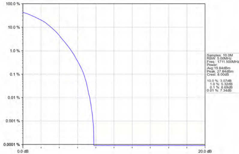
Band66_3MHz_64QAM_LCH_1711.5MHz_RB_15_0_NTNV
