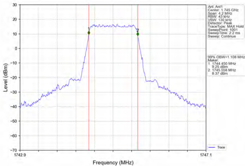
Band66_1.4MHz_64QAM_MCH_1745MHz_RB_6_0_NTNV
