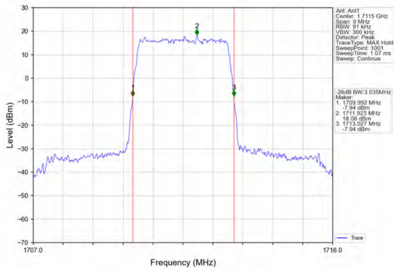
Band66_3MHz_QPSK_LCH_1711.5MHz_RB_15_0_NTNV
