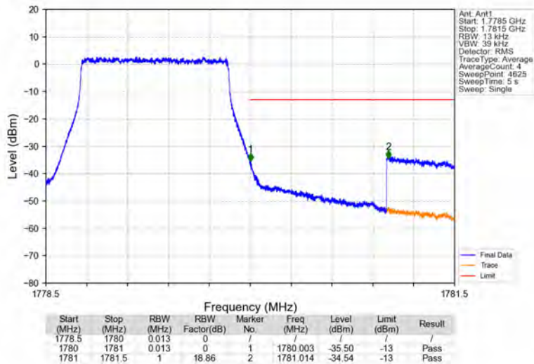
Band66_1.4MHz_64QAM_HCH_1779.3MHz_RB_6_0_NTNV
