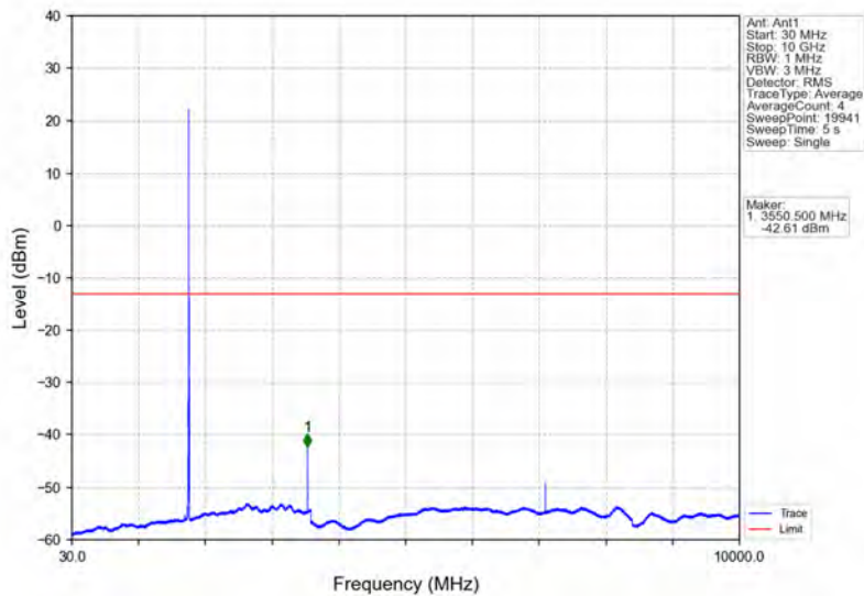
Band66_5MHz_QPSK_HCH_1777.5MHz_RB_1_0_NTNV
