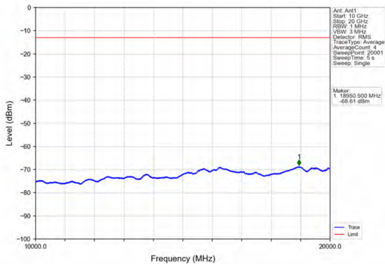
Band66_5MHz_16QAM_MCH_1745MHz_RB_1_0_NTNV
