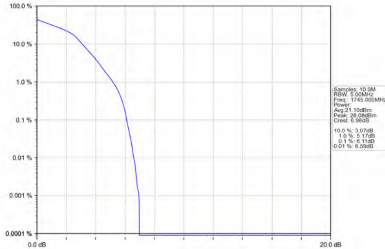
Band66_1.4MHz_16QAM_MCH_1745MHz_RB_6_0_NTNV
