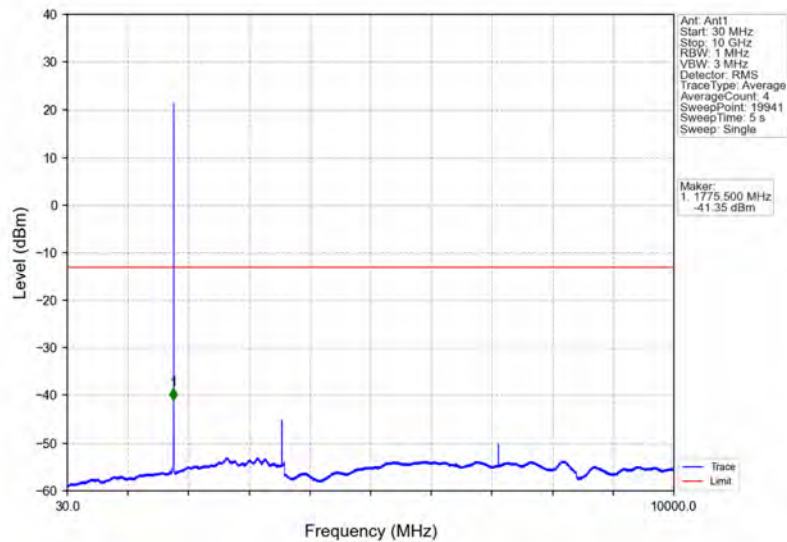
Band66_1.4MHz_16QAM_HCH_1779.3MHz_RB_1_0_NTNV
