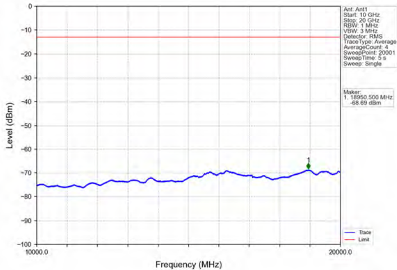
Band66_20MHz_64QAM_LCH_1720MHz_RB_100_0_NTNV
