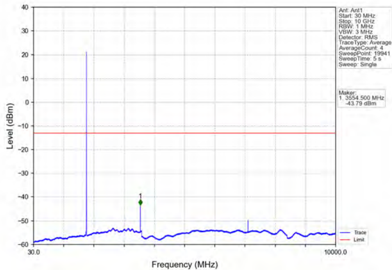
Band66_3MHz_16QAM_HCH_1778.5MHz_RB_1_0_NTNV
