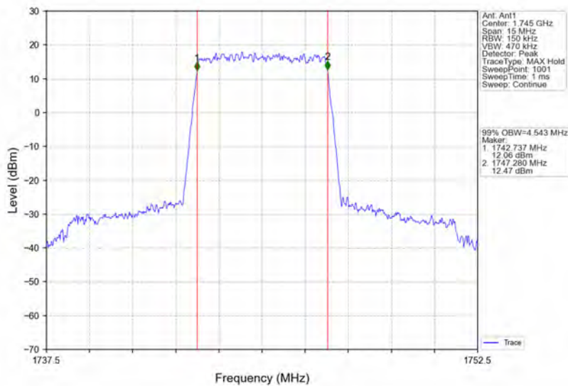
Band66_5MHz_QPSK_MCH_1745MHz_RB_25_0_NTNV
