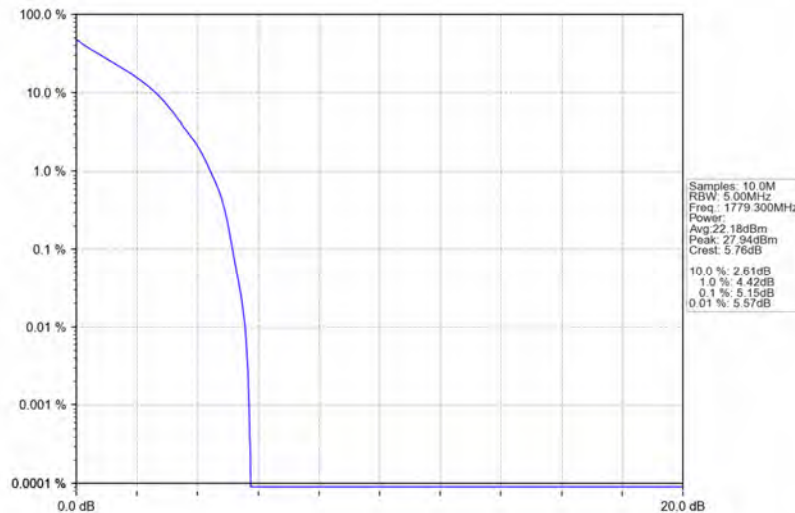
Band66_1.4MHz_QPSK_HCH_1779.3MHz_RB_6_0_NTNV
