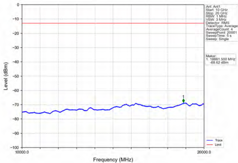
Band66_1.4MHz_QPSK_MCH_1745MHz_RB_1_0_NTNV
