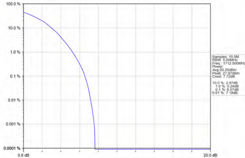
Band66_5MHz_64QAM_LCH_1712.5MHz_RB_25_0_NTNV
