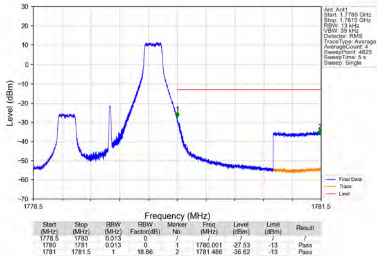
Band66_1.4MHz_16QAM_HCH_1779.3MHz_RB_1_5_NTNV
