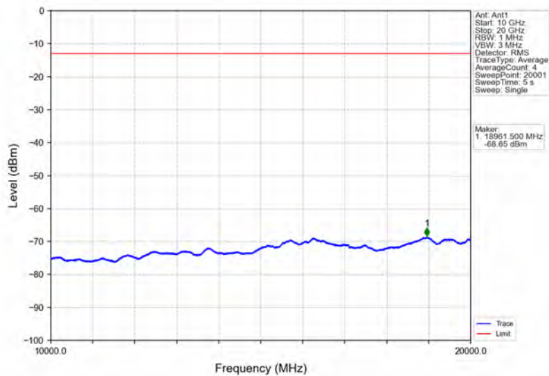
Band66_3MHz_64QAM_HCH_1778.5MHz_RB_1_0_NTNV
