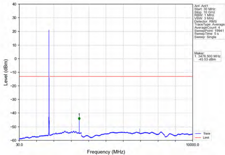
Band66_15MHz_64QAM_MCH_1745MHz_RB_1_0_NTNV
