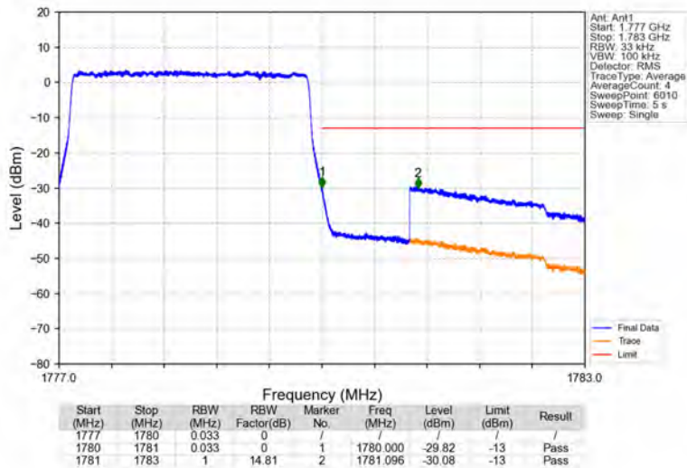
Band66_3MHz_16QAM_HCH_1778.5MHz_RB_15_0_NTNV
