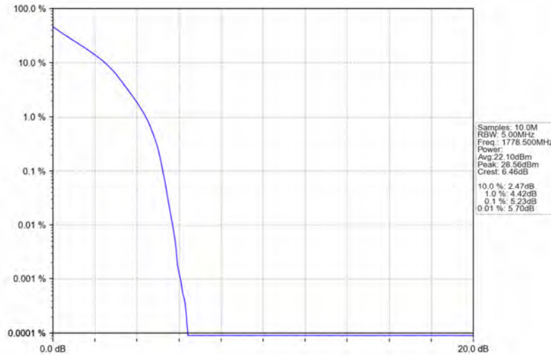
Band66_3MHz_QPSK_HCH_1778.5MHz_RB_15_0_NTNV
