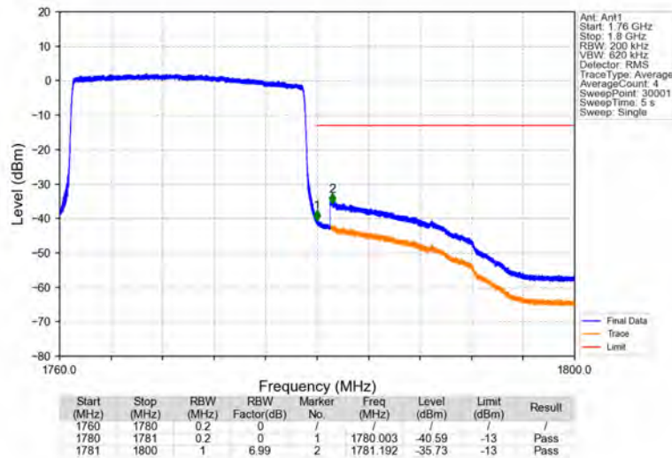
Band66_20MHz_64QAM_HCH_1770MHz_RB_100_0_NTNV
