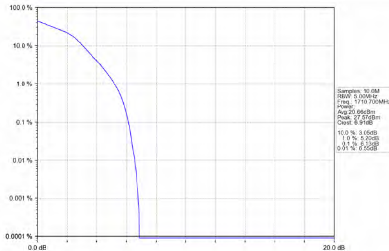
Band66_1.4MHz_16QAM_LCH_1710.7MHz_RB_6_0_NTNV
