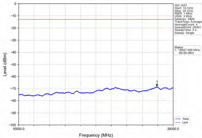
Band66_10MHz_64QAM_LCH_1715MHz_RB_50_0_NTNV
