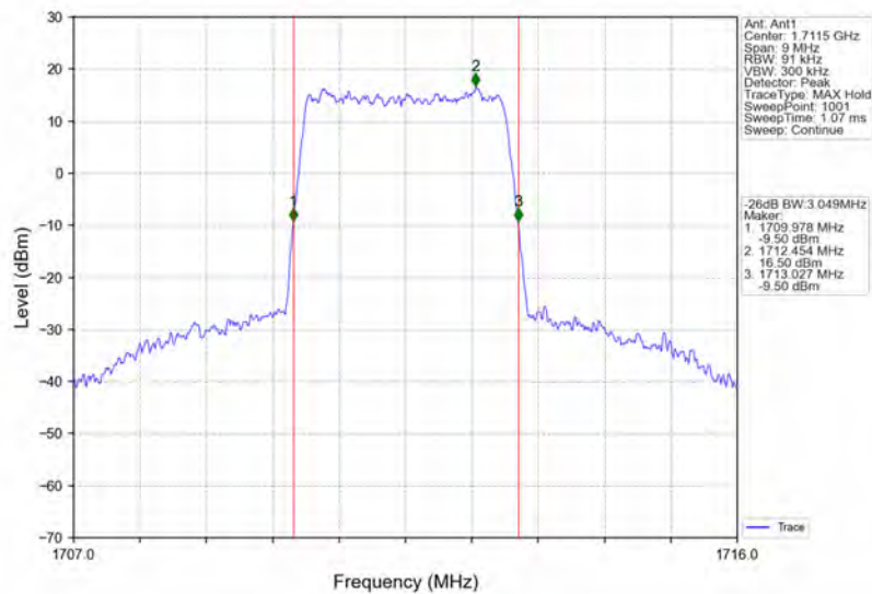
Band66_3MHz_64QAM_LCH_1711.5MHz_RB_15_0_NTNV
