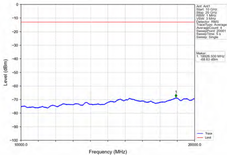
Band66_1.4MHz_64QAM_MCH_1745MHz_RB_1_0_NTNV
