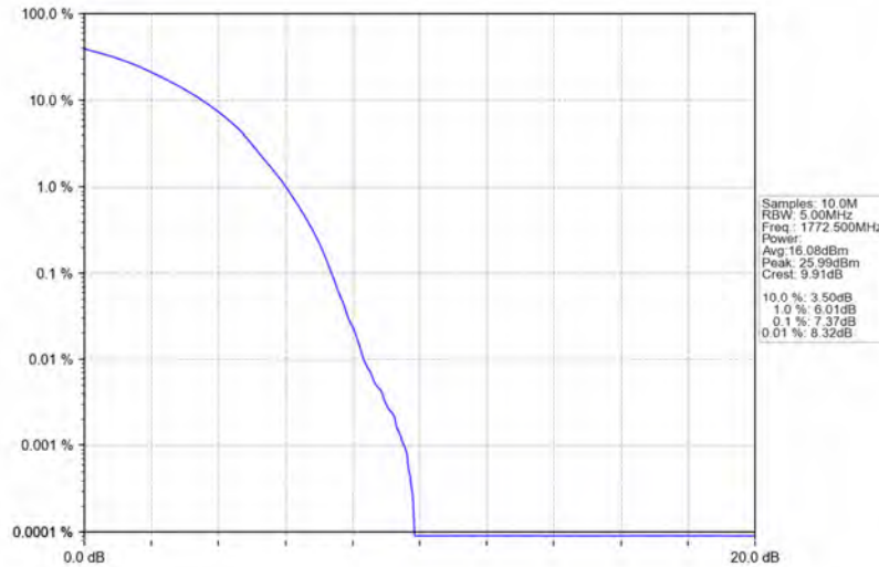
Band66_15MHz_64QAM_HCH_1772.5MHz_RB_75_0_NTNV
