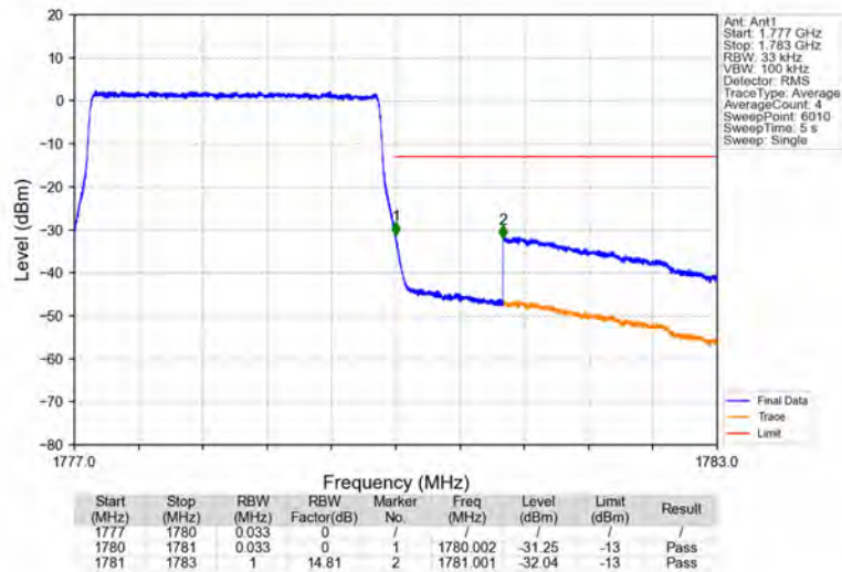
Band66_3MHz_64QAM_HCH_1778.5MHz_RB_15_0_NTNV
