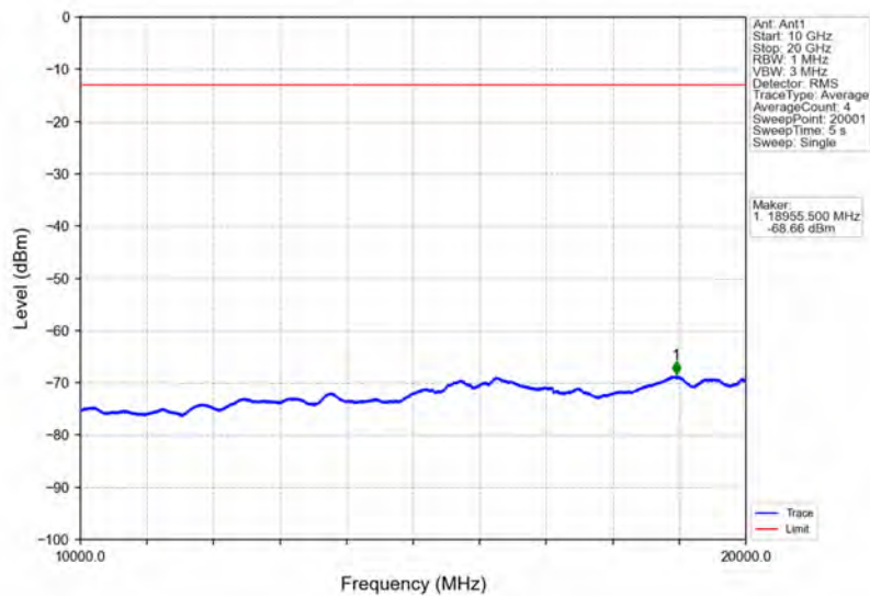
Band66_5MHz_64QAM_HCH_1777.5MHz_RB_1_0_NTNV
