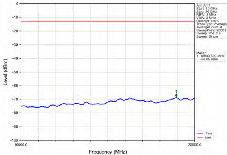
Band66_15MHz_16QAM_LCH_1717.5MHz_RB_75_0_NTNV
