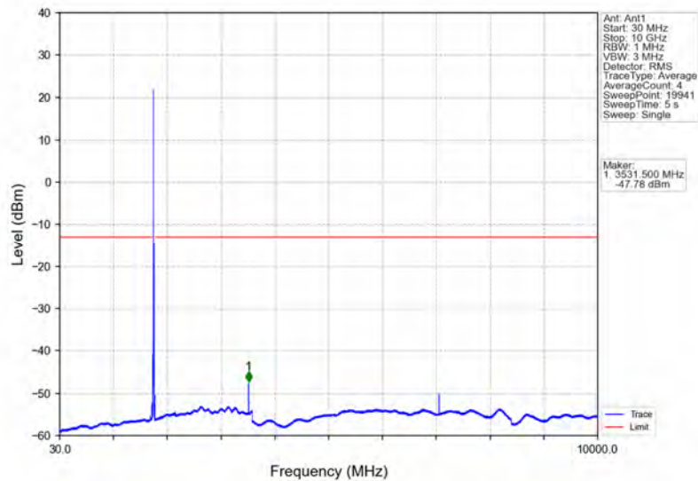
Band66_15MHz_QPSK_HCH_1772.5MHz_RB_1_0_NTNV
