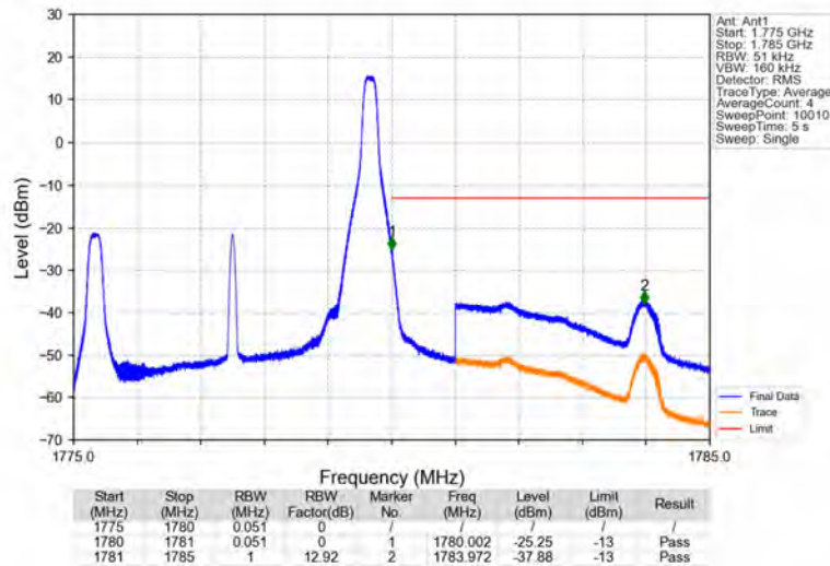
Band66_5MHz_64QAM_HCH_1777.5MHz_RB_1_24_NTNV
