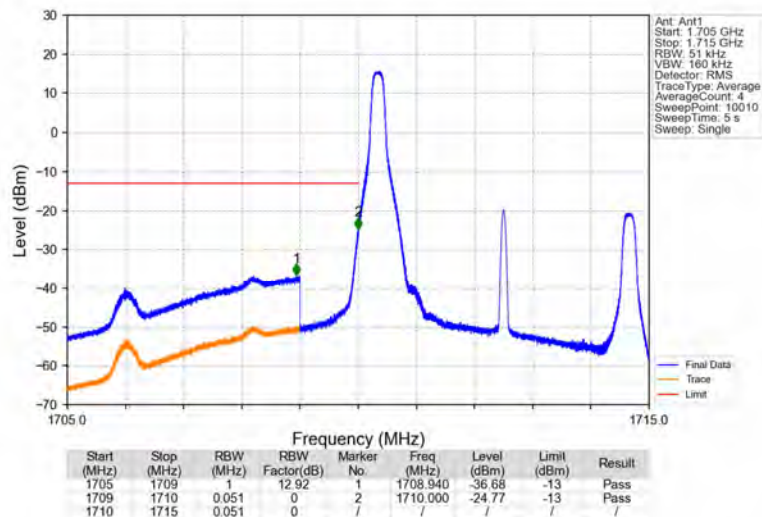
Band66_5MHz_64QAM_LCH_1712.5MHz_RB_1_0_NTNV
