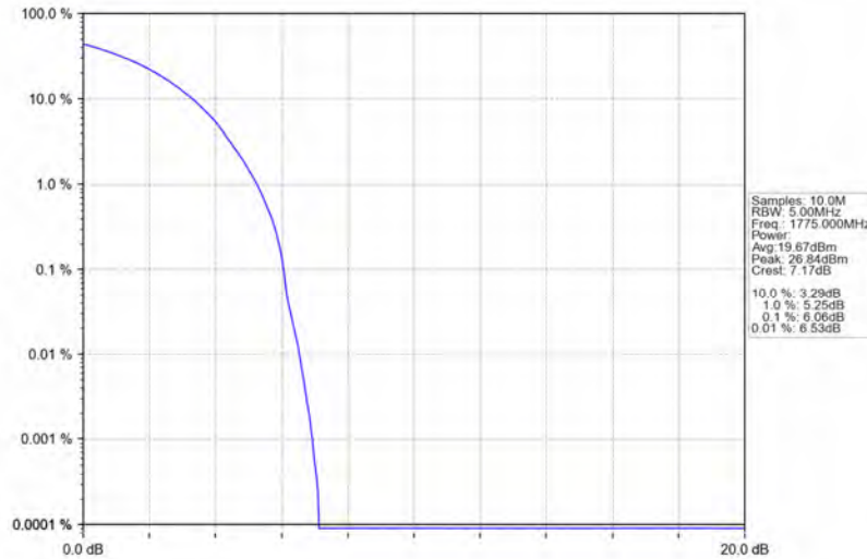
Band66_10MHz_QPSK_HCH_1775MHz_RB_50_0_NTNV
