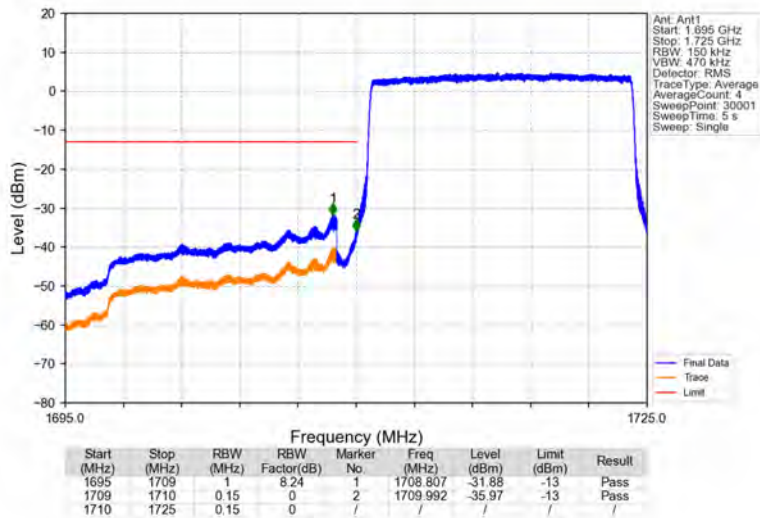
Band66_15MHz_QPSK_LCH_1717.5MHz_RB_75_0_NTNV
