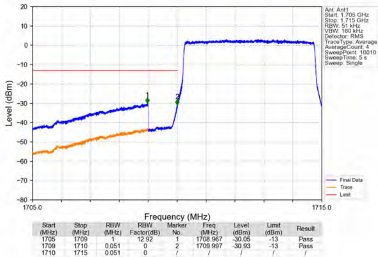
Band66_5MHz_16QAM_LCH_1712.5MHz_RB_25_0_NTNV
