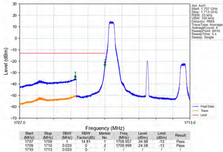
Band66_3MHz_64QAM_LCH_1711.5MHz_RB_1_0_NTNV
