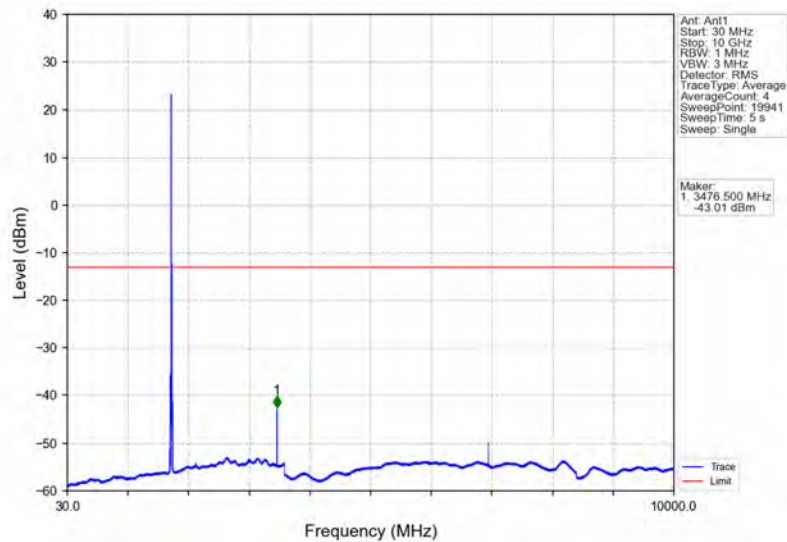
Band66_15MHz_QPSK_MCH_1745MHz_RB_1_0_NTNV
