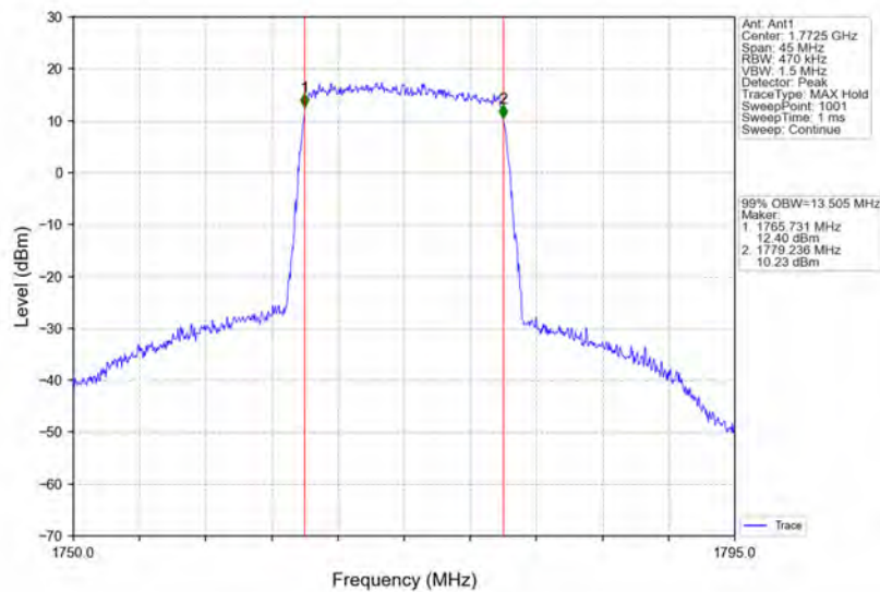
Band66_15MHz_16QAM_HCH_1772.5MHz_RB_75_0_NTNV
