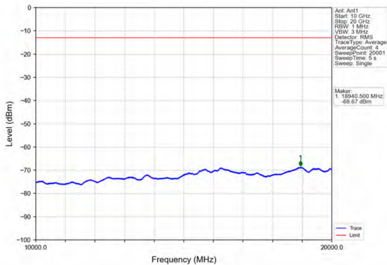
Band66_10MHz_64QAM_MCH_1745MHz_RB_1_0_NTNV
