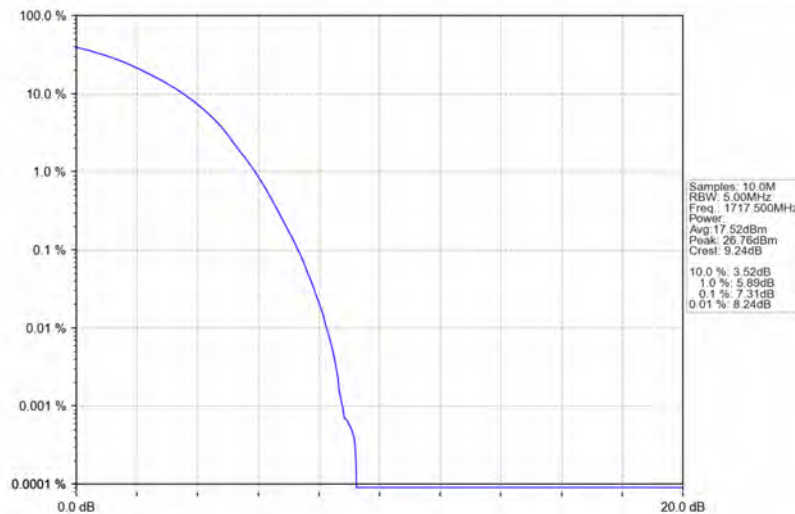
Band66_15MHz_16QAM_LCH_1717.5MHz_RB_75_0_NTNV
