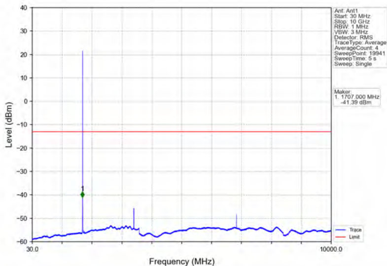
Band66_1.4MHz_16QAM_LCH_1710.7MHz_RB_1_0_NTNV
