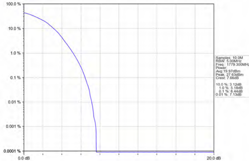
Band66_1.4MHz_64QAM_HCH_1779.3MHz_RB_6_0_NTNV
