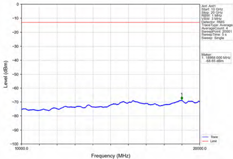
Band66_10MHz_QPSK_LCH_1715MHz_RB_50_0_NTNV
