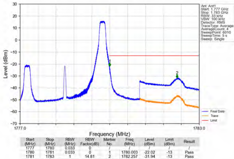
Band66_3MHz_QPSK_HCH_1778.5MHz_RB_1_14_NTNV
