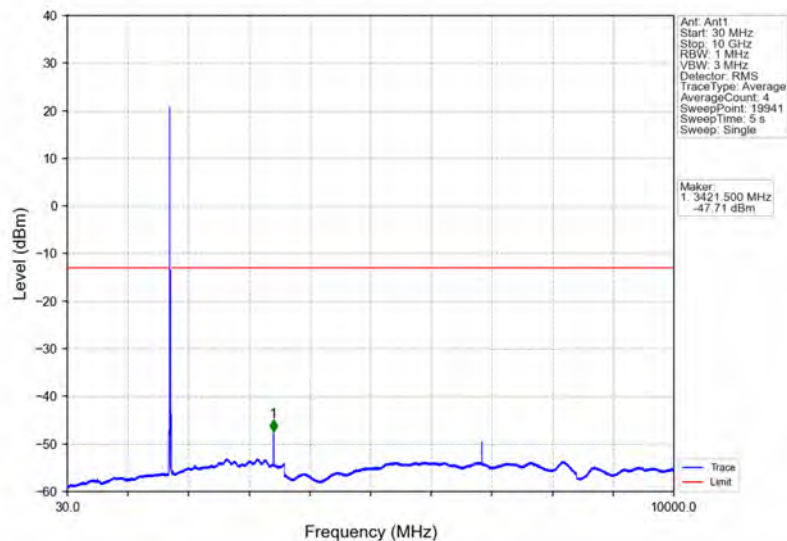
Band66_15MHz_64QAM_LCH_1717.5MHz_RB_1_0_NTNV
