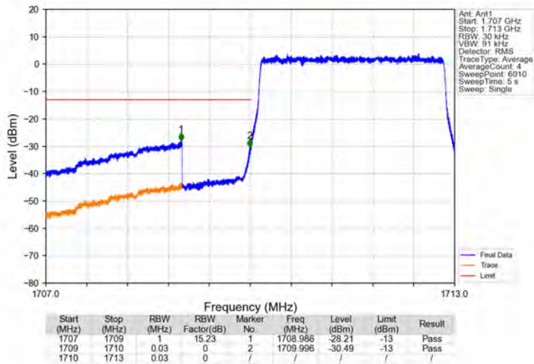
Band66_3MHz_16QAM_LCH_1711.5MHz_RB_15_0_NTNV
