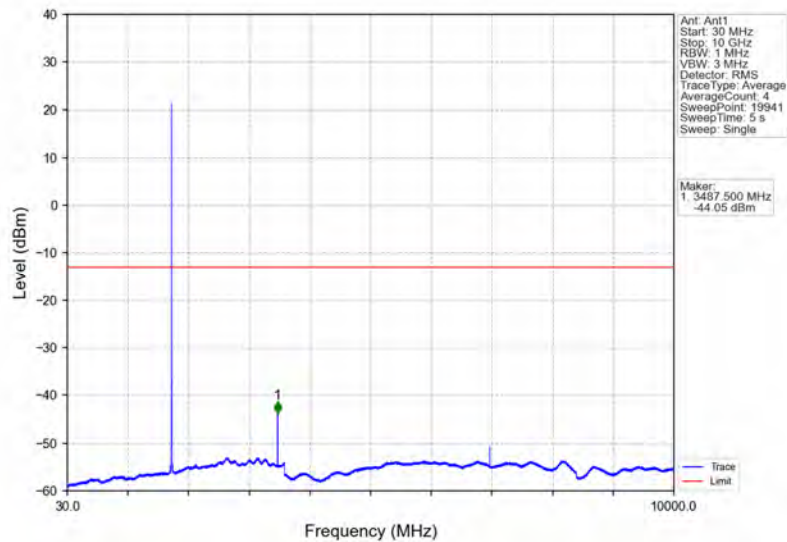
Band66_3MHz_16QAM_MCH_1745MHz_RB_1_0_NTNV
