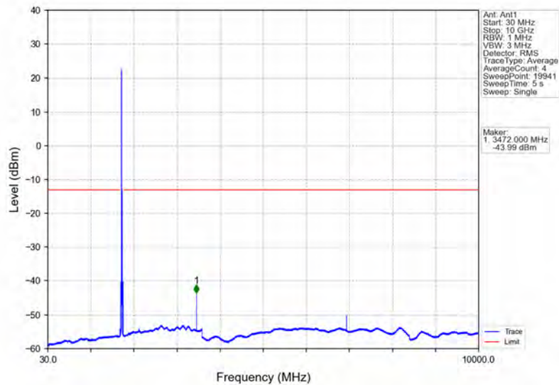
Band66_20MHz_16QAM_MCH_1745MHz_RB_1_0_NTNV
