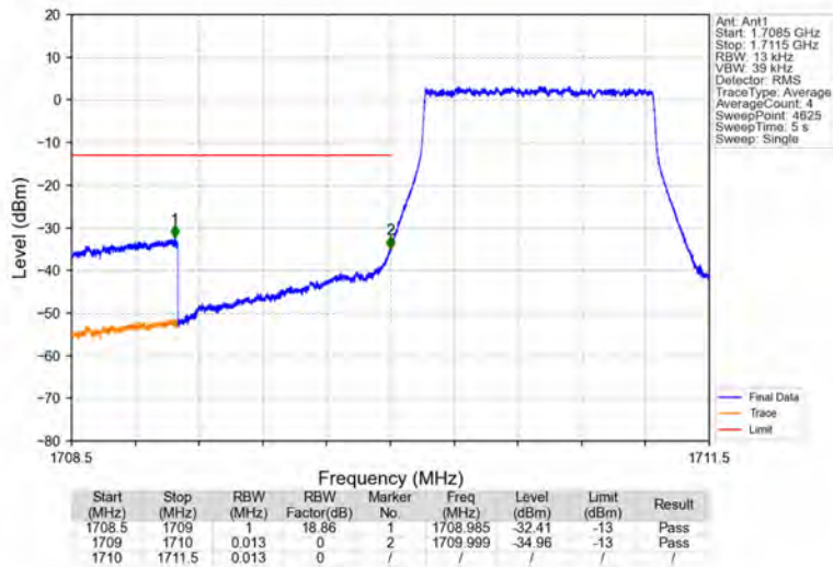
Band66_1.4MHz_16QAM_LCH_1710.7MHz_RB_6_0_NTNV
