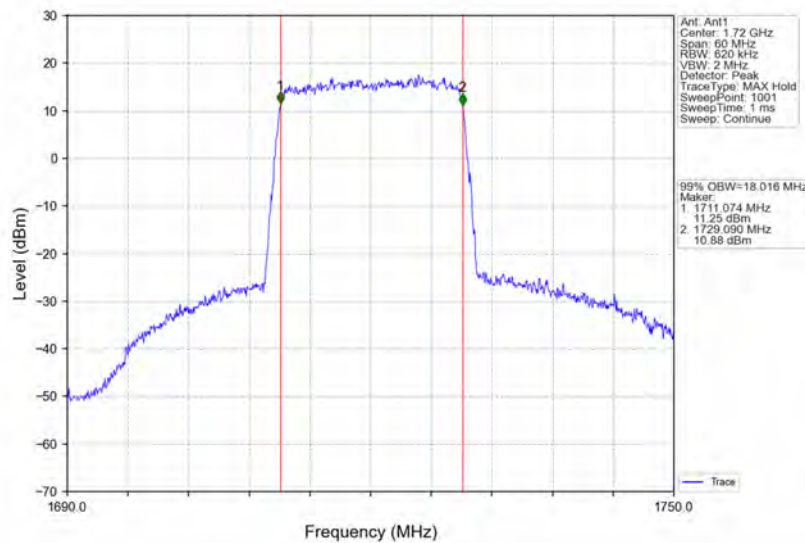
Band66_20MHz_64QAM_LCH_1720MHz_RB_100_0_NTNV
