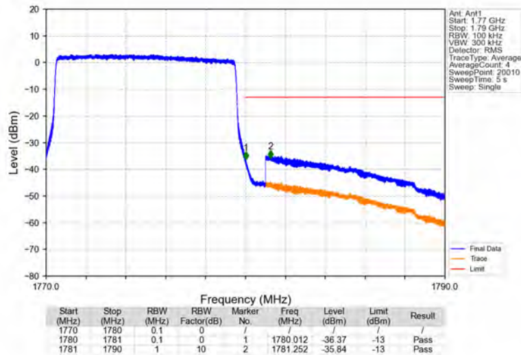
Band66_10MHz_16QAM_HCH_1775MHz_RB_50_0_NTNV
