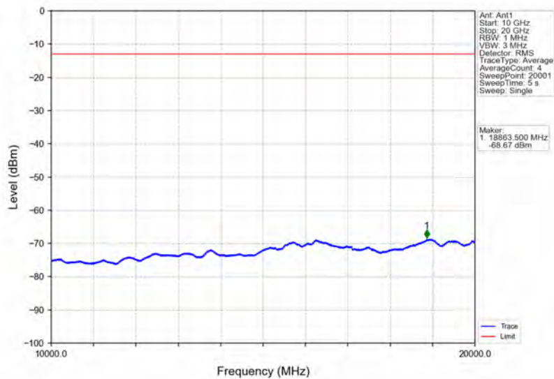
Band66_15MHz_64QAM_MCH_1745MHz_RB_1_0_NTNV
