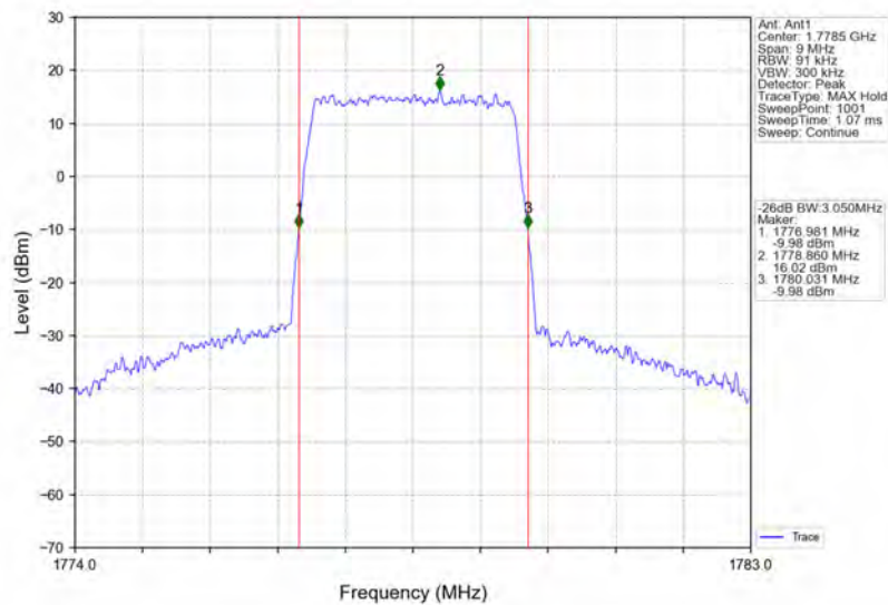
Band66_3MHz_64QAM_HCH_1778.5MHz_RB_15_0_NTNV
