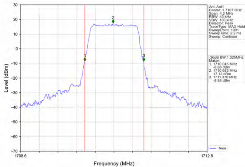
Band66_1.4MHz_16QAM_LCH_1710.7MHz_RB_6_0_NTNV
