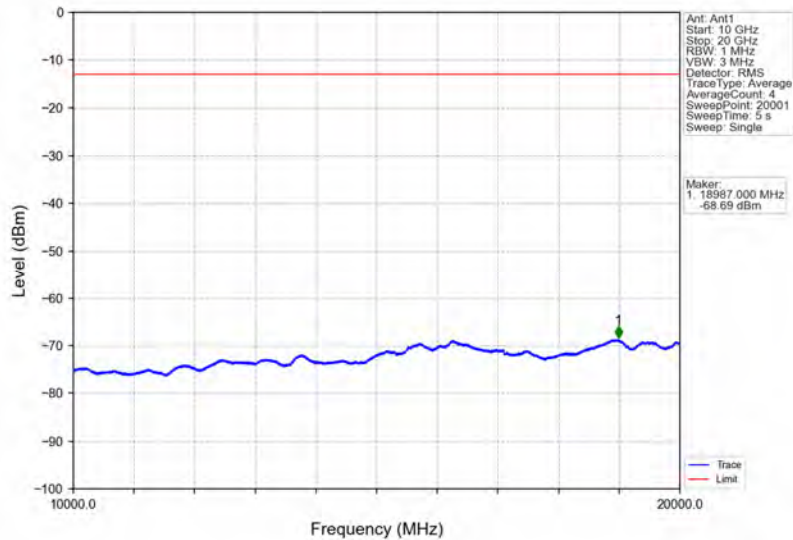
Band66_1.4MHz_64QAM_LCH_1710.7MHz_RB_6_0_NTNV
