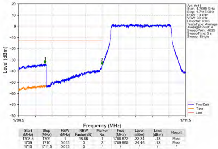
Band66_1.4MHz_64QAM_LCH_1710.7MHz_RB_6_0_NTNV
