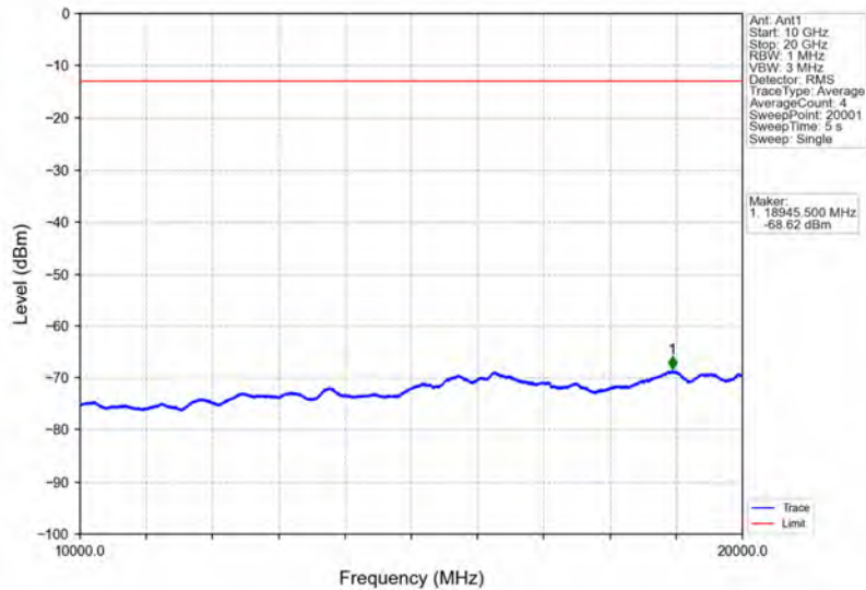
Band66_5MHz_QPSK_LCH_1712.5MHz_RB_25_0_NTNV
