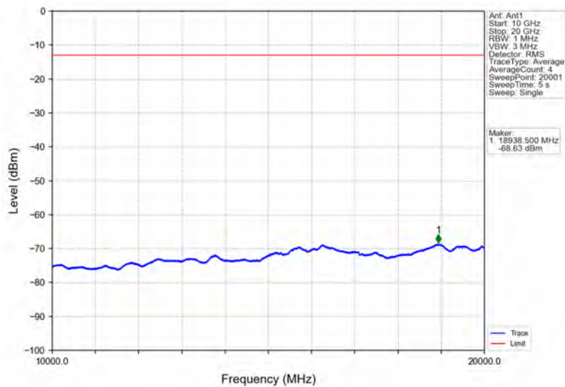
Band66_3MHz_16QAM_MCH_1745MHz_RB_1_0_NTNV
