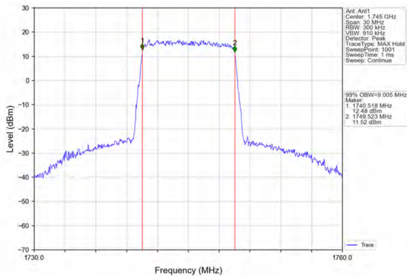
Band66_10MHz_16QAM_MCH_1745MHz_RB_50_0_NTNV
