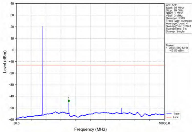
Band66_3MHz_64QAM_HCH_1778.5MHz_RB_1_0_NTNV
