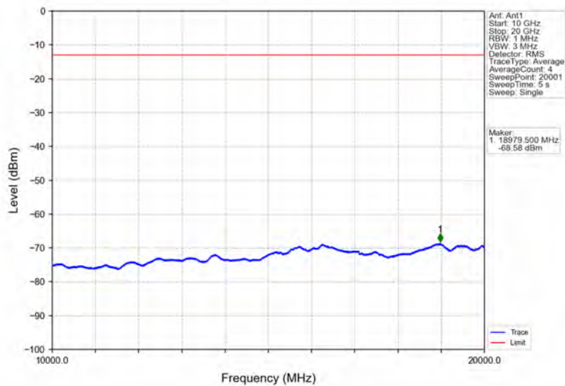
Band66_15MHz_QPSK_MCH_1745MHz_RB_1_0_NTNV
