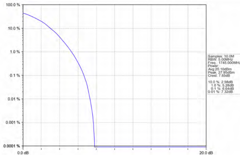
Band66_5MHz_64QAM_MCH_1745MHz_RB_25_0_NTNV
