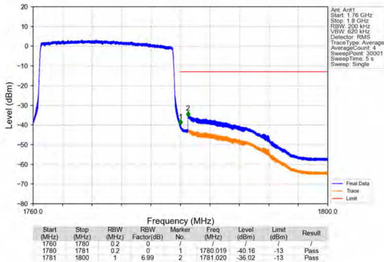
Band66_20MHz_16QAM_HCH_1770MHz_RB_100_0_NTNV
