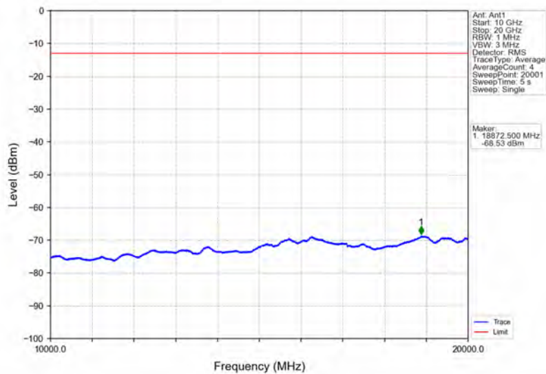
Band66_5MHz_QPSK_HCH_1777.5MHz_RB_1_0_NTNV
