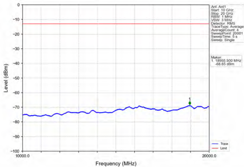
Band66_15MHz_16QAM_MCH_1745MHz_RB_1_0_NTNV
