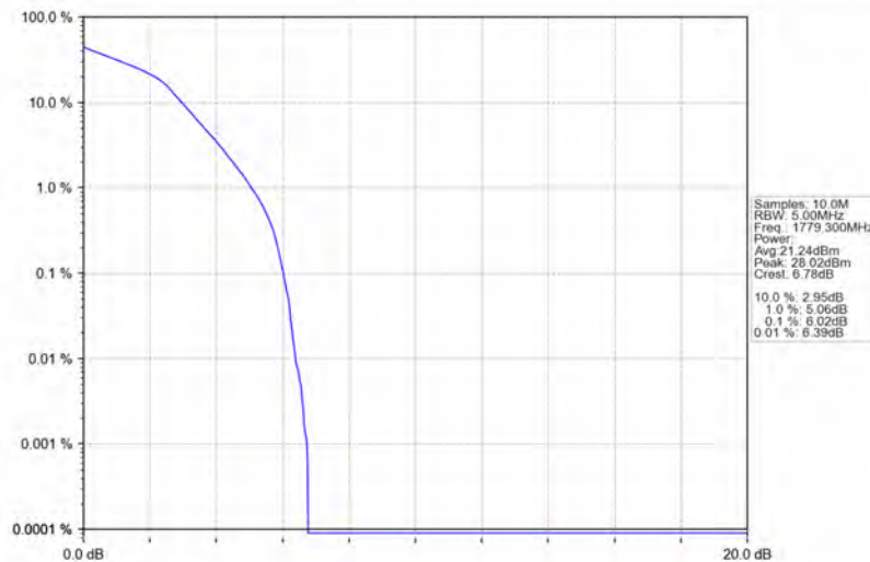
Band66_1.4MHz_16QAM_HCH_1779.3MHz_RB_6_0_NTNV
