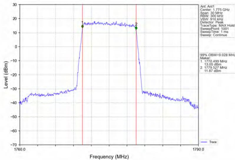
Band66_10MHz_QPSK_HCH_1775MHz_RB_50_0_NTNV
