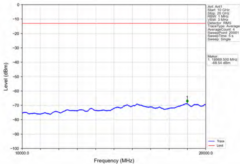
Band66_10MHz_QPSK_MCH_1745MHz_RB_1_0_NTNV
