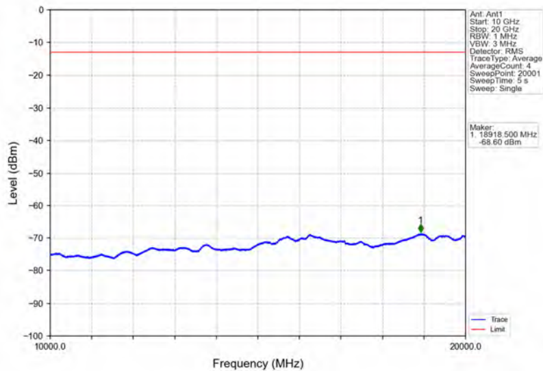
Band66_3MHz_QPSK_LCH_1711.5MHz_RB_15_0_NTNV
