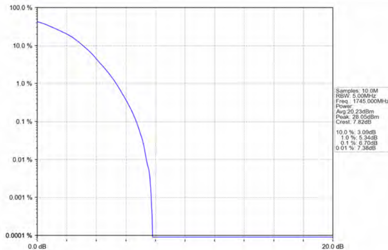
Band66_3MHz_64QAM_MCH_1745MHz_RB_15_0_NTNV
