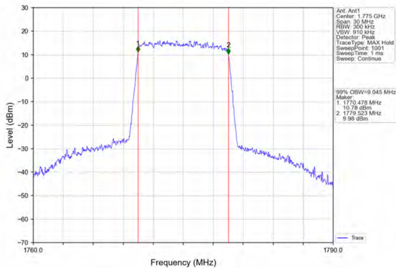
Band66_10MHz_64QAM_HCH_1775MHz_RB_50_0_NTNV
