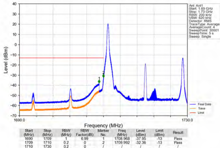
Band66_20MHz_64QAM_LCH_1720MHz_RB_1_0_NTNV
