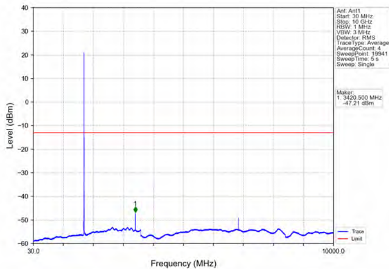
Band66_5MHz_16QAM_LCH_1712.5MHz_RB_1_0_NTNV
