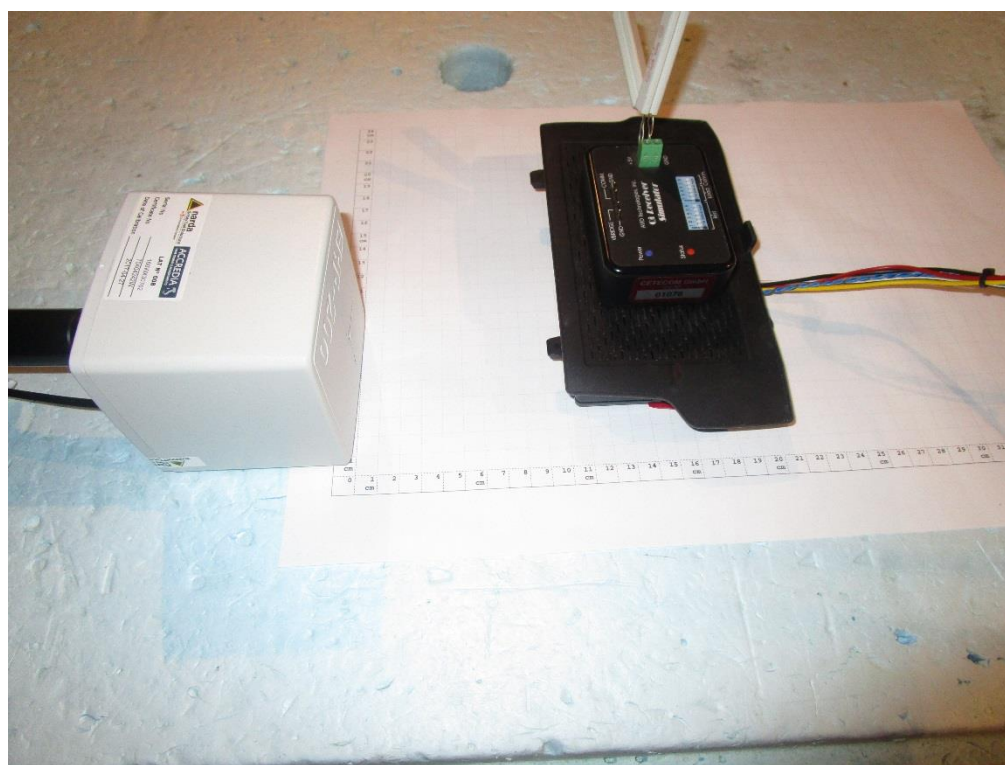
Photograph 2: Measurements in the anechoic chamber, 10cm distance between measurement probe and EUT, Position 1
