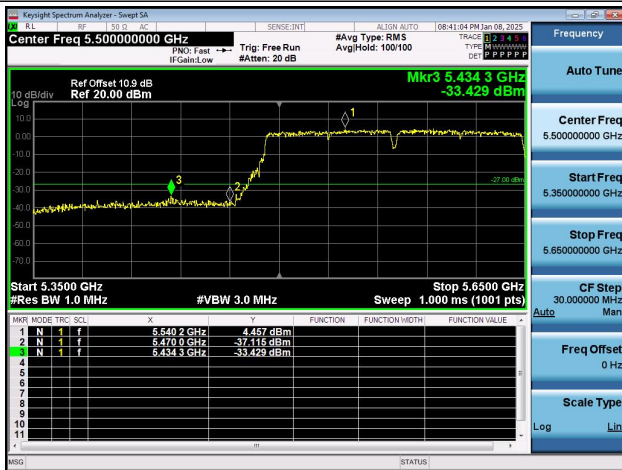
11AC160SISO-Ant2-5570-PASS
