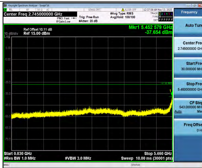
11N40SISO_Ant0_5510_5735~27000
