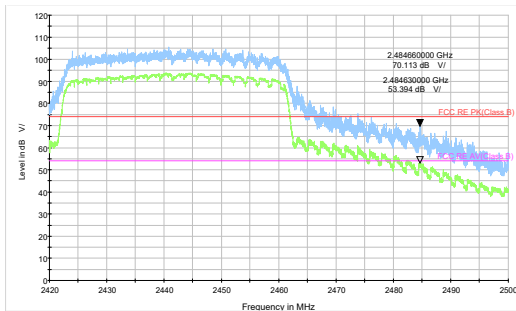
802.11ax HE40-Channel 7 Peak+ Average
