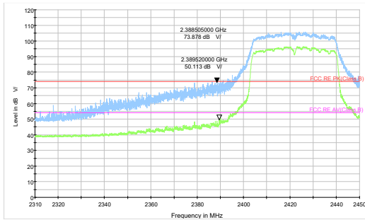
802.11n HT40-Channel 3 Peak+ Average
