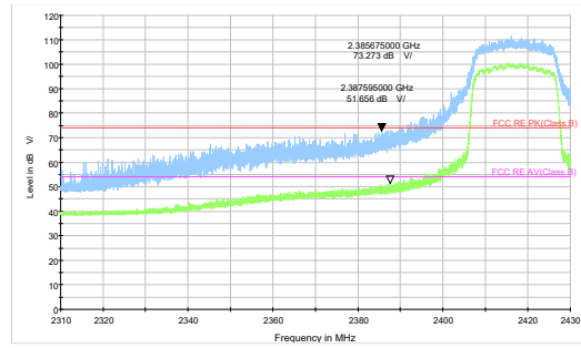
802.11ax HE20-Channel 2 Peak+ Average
