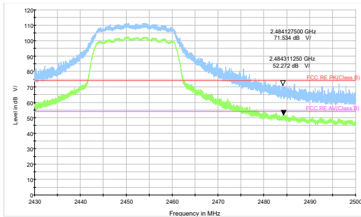
802.11n HT20-Channel 9 Peak+ Average
