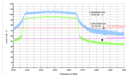
802.11ax HE40-Channel 8 Peak+ Average
