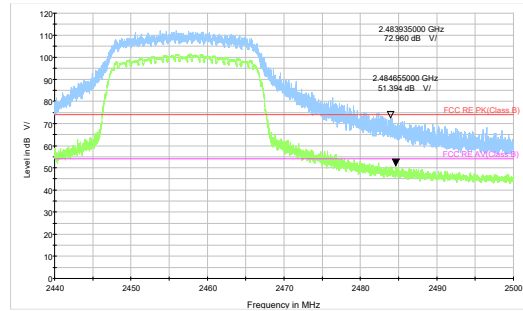
802.11ax HE20-Channel 10 Peak+ Average
