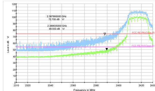
802.11g-Channel 2 Peak+ Average
