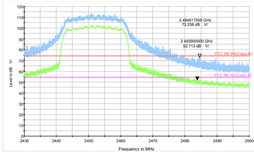
802.11ax HE20-Channel 9 Peak+ Average
