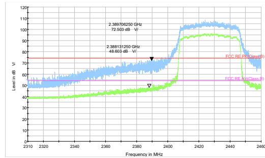
802.11ax HE40-Channel 4 Peak+ Average
