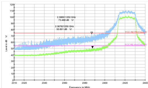
802.11g-Channel 3 Peak+ Average
