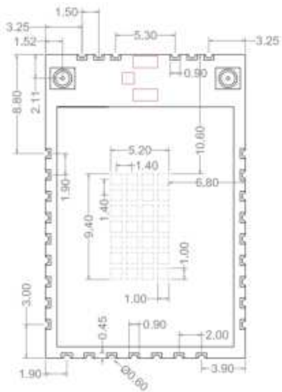
(TopView)(Bottom View)
