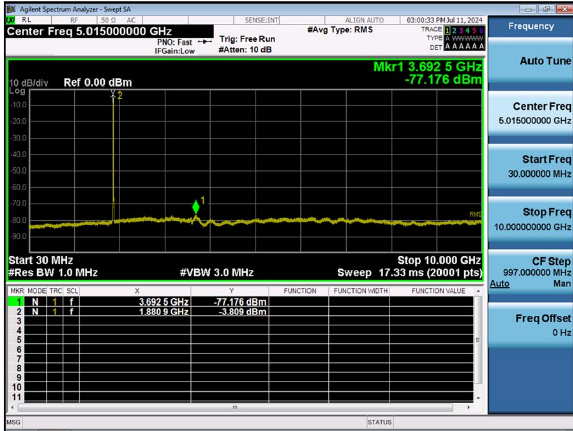
LTE B25(2)_5 M_Conducted Spurious(30 M-10 G)_Mid_QPSK_1RB
