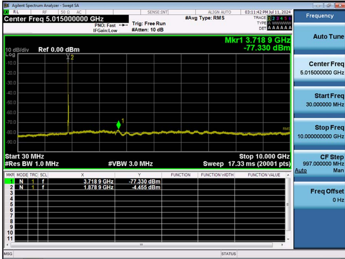
LTE B25(2)_10 M_Conducted Spurious(30 M-10 G)_Mid_QPSK_1RB
