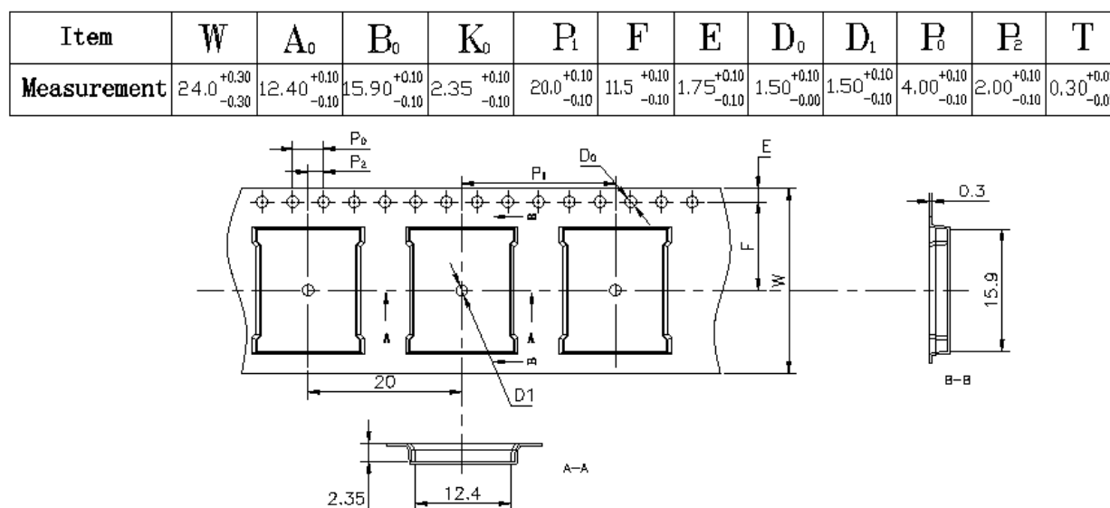
Figure 24. CYBT-343151-02 Tape Dimensions
