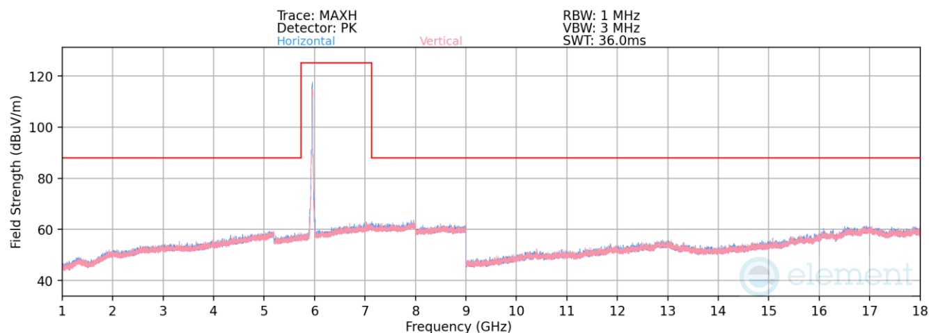
Plot 7-1693. Radiated Spurious Emissions above 1GHz SDM Diversity (802.11ax – Ch. 1 – RU242)
