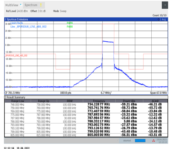
1-N14--15-5-L-6-CP-QPSK-Outer_Full-25@0-Ant1-PASS-see graph
