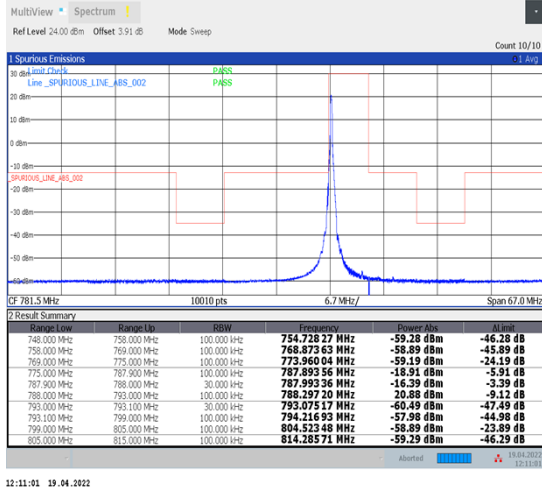
1-N14--15-5-L-1-DFT-PI2BPSK-Edge_1RB_Left-1@0-Ant1-PASS-see graph
