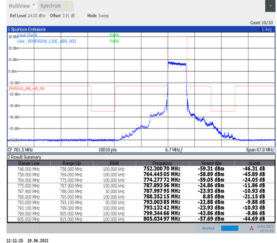
1-N14--15-5-L-3-DFT-PI2BPSK-Outer_Full-25@0-Ant1-PASS-see graph
