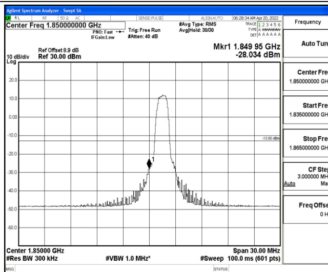
Band25-15MHz-16QAM-26115-6-0-Low--28.03-PASS
