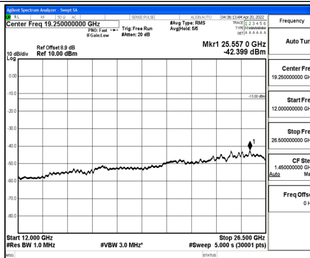
Band25-1.4MHz-16QAM-26047-1-0-Low-12000-26500--42.4-PASS
