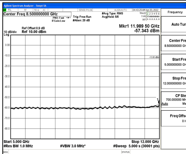
Band25-1.4MHz-16QAM-26683-1-0-High-5000-12000--57.34-PASS
