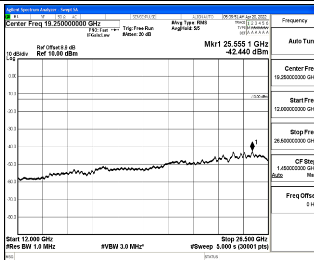
Band25-5MHz-16QAM-26365-1-0-Low-12000-26500--42.44-PASS
