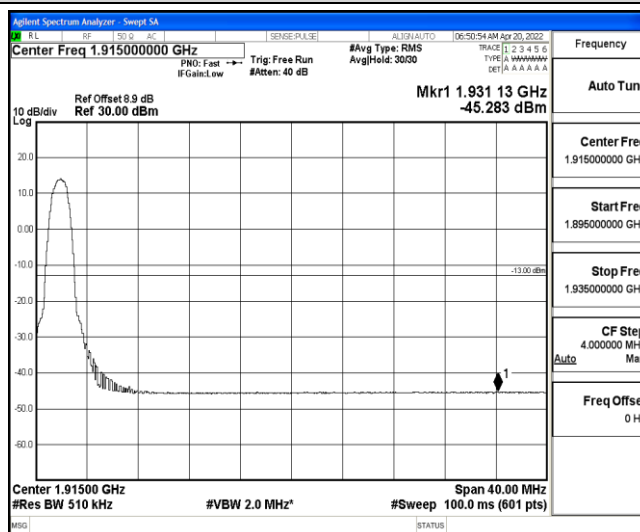
Band25-20MHz-16QAM-26590-6-0-Low--45.28-PASS
