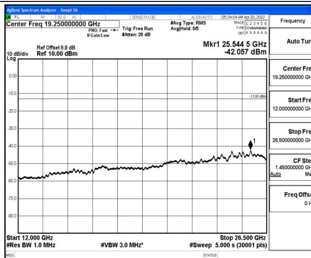
Band25-5MHz-QPSK-26065-1-0-Low-12000-26500--42.06-PASS
