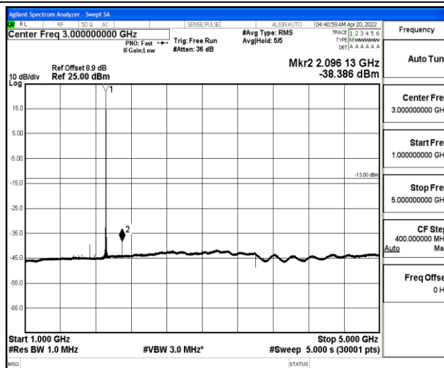
Band25-1.4MHz-QPSK-26683-1-0-High-1000-5000--38.39-PASS
