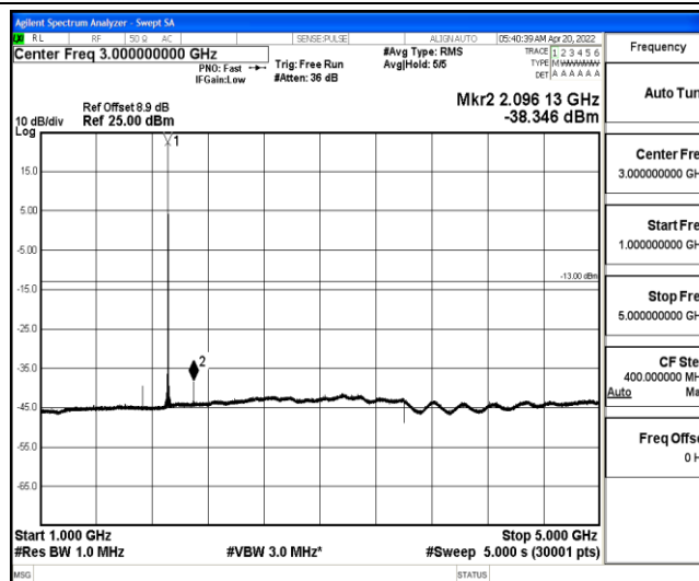
Band25-5MHz-QPSK-26665-1-0-High-1000-5000--38.35-PASS
