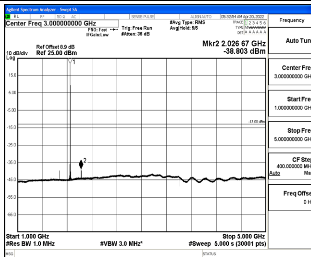
Band25-5MHz-QPSK-26065-1-0-Low-1000-5000--38.8-PASS
