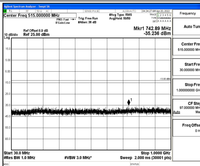
Band25-1.4MHz-16QAM-26047-1-0-Low-30-1000--35.24-PASS
