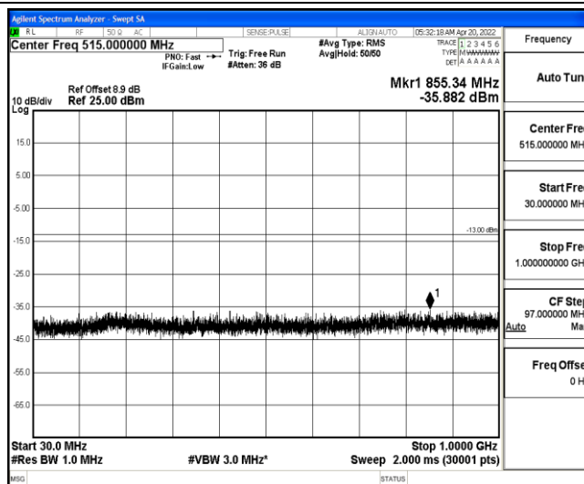
Band25-5MHz-QPSK-26065-1-0-Low-30-1000--35.88-PASS
