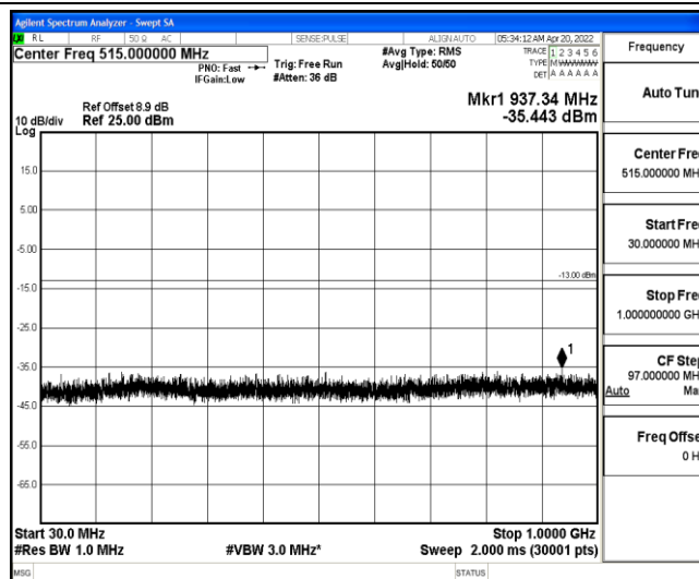
Band25-5MHz-16QAM-26065-1-0-Low-30-1000--35.44-PASS
