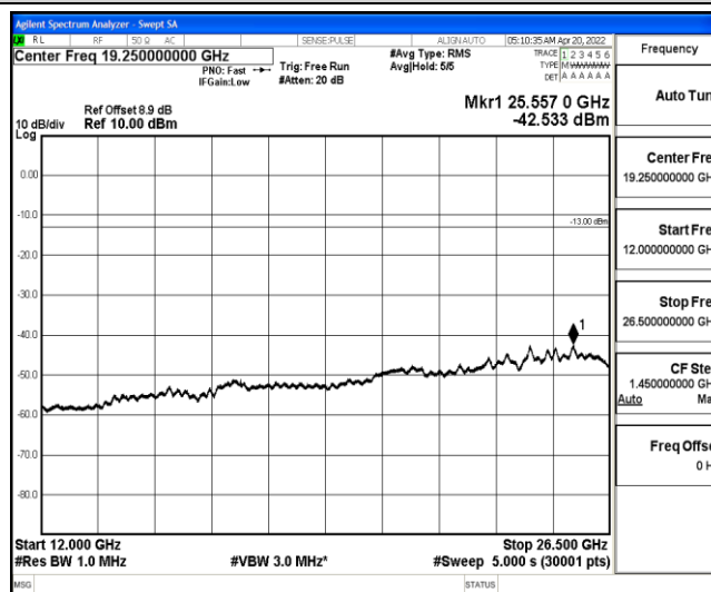
Band25-3MHz-16QAM-26675-1-0-High-12000-26500--42.53-PASS
