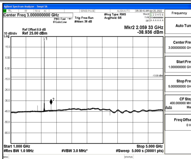
Band25-5MHz-16QAM-26365-1-0-Low-1000-5000--38.94-PASS
