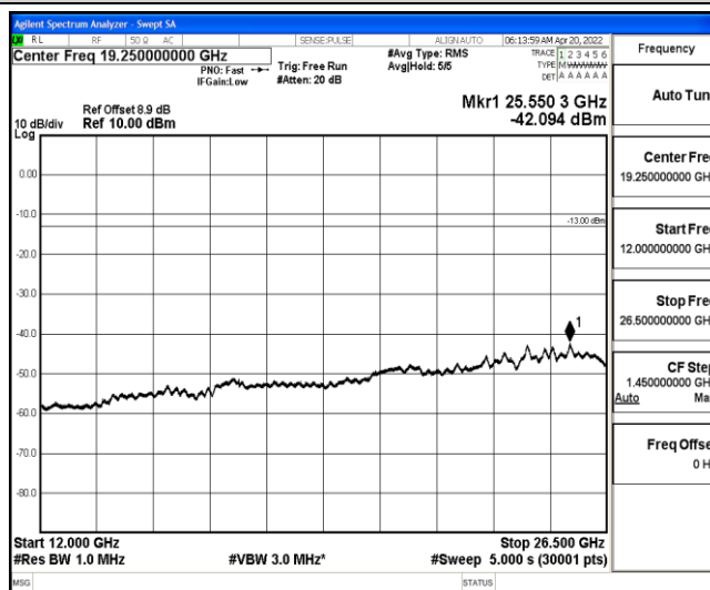
Band25-10MHz-QPSK-26640-1-0-High-12000-26500--42.09-PASS
