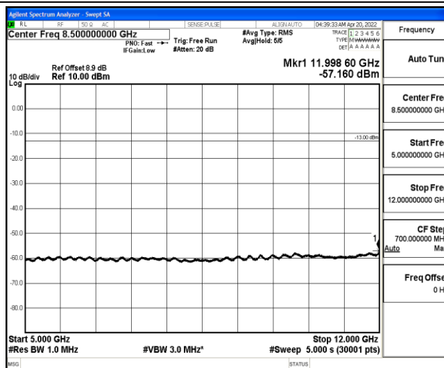
Band25-1.4MHz-16QAM-26365-1-0-Low-5000-12000--57.16-PASS
