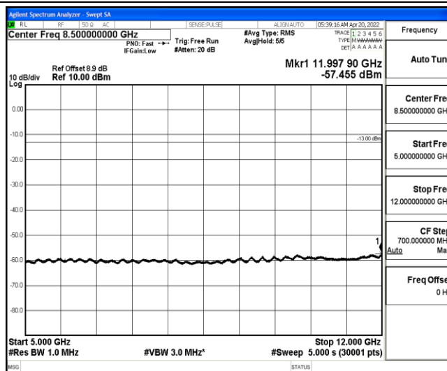
Band25-5MHz-16QAM-26365-1-0-Low-5000-12000--57.46-PASS
