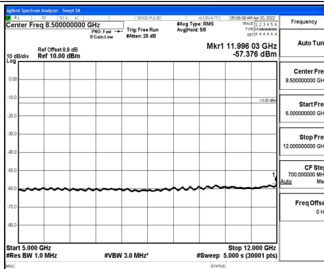
Band25-3MHz-16QAM-26365-1-0-Low-5000-12000--57.38-PASS
