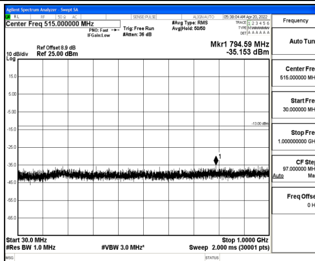
Band25-5MHz-16QAM-26365-1-0-Low-30-1000--35.15-PASS
