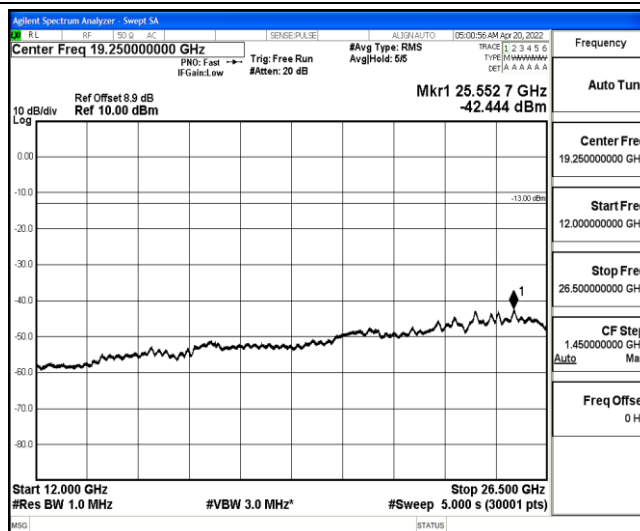
Band25-3MHz-QPSK-26055-1-0-Low-12000-26500--42.44-PASS
