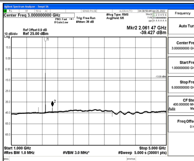
Band25-1.4MHz-16QAM-26365-1-0-Low-1000-5000--39.43-PASS
