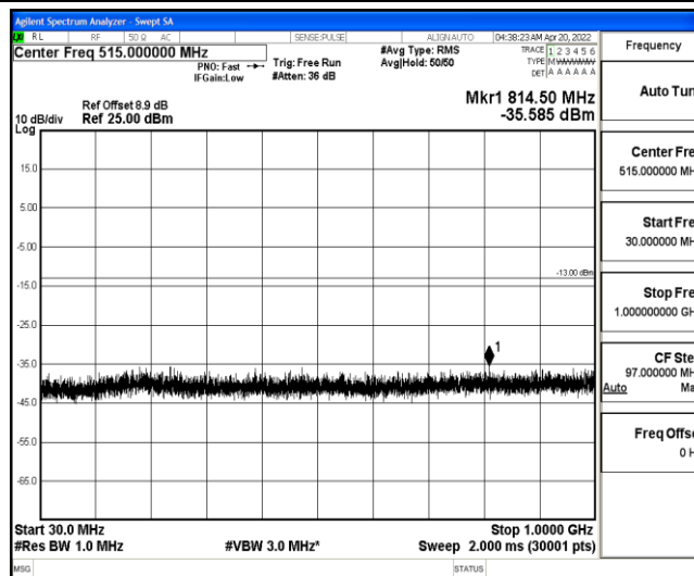
Band25-1.4MHz-16QAM-26365-1-0-Low-30-1000--35.59-PASS
