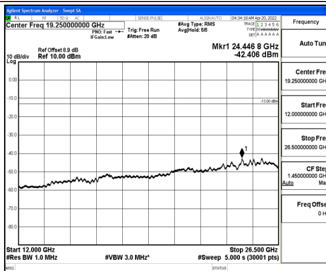
Band25-1.4MHz-QPSK-26047-1-0-Low-12000-26500--42.41-PASS
