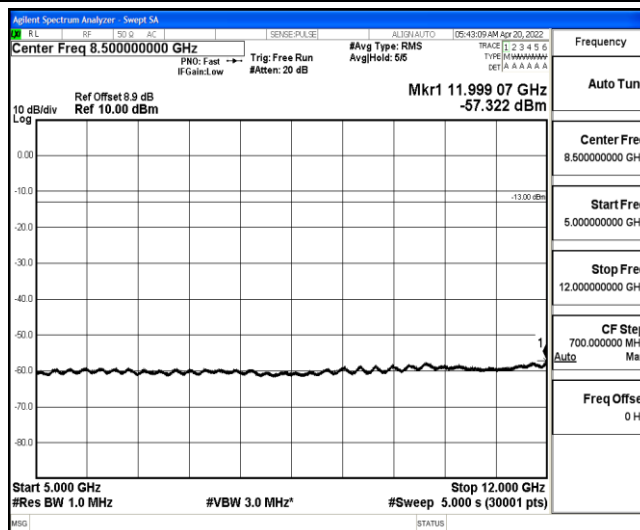
Band25-5MHz-16QAM-26665-1-0-High-5000-12000--57.32-PASS
