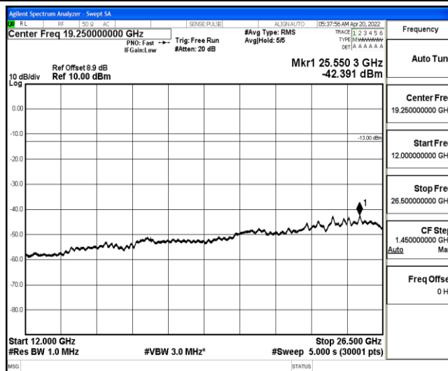
Band25-5MHz-QPSK-26365-1-0-Low-12000-26500--42.39-PASS
