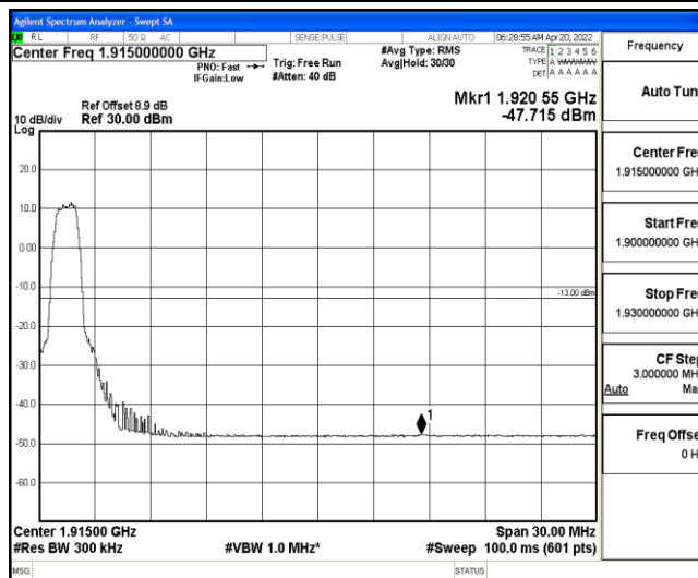
Band25-15MHz-16QAM-26615-6-0-Low--47.71-PASS
