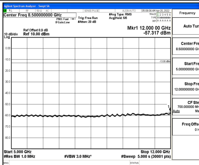
Band25-3MHz-QPSK-26675-1-0-High-5000-12000--57.32-PASS
