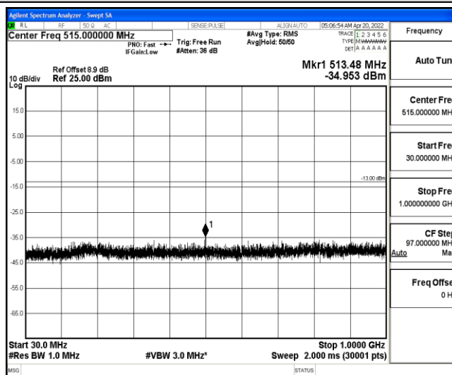
Band25-3MHz-QPSK-26675-1-0-High-30-1000--34.95-PASS
