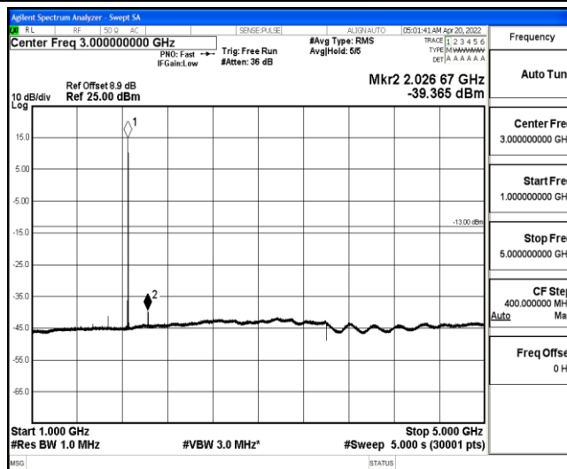
Band25-3MHz-16QAM-26055-1-0-Low-1000-5000--39.37-PASS
