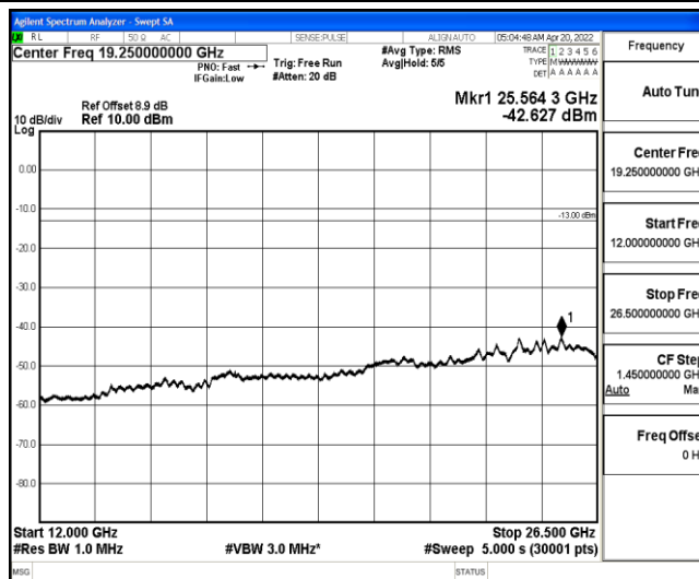
Band25-3MHz-QPSK-26365-1-0-Low-12000-26500--42.63-PASS
