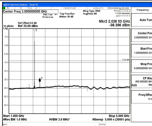
Band25-5MHz-16QAM-26065-1-0-Low-1000-5000--38.4-PASS
