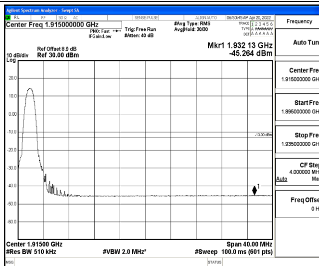
Band25-20MHz-QPSK-26590-6-0-Low--45.26-PASS
