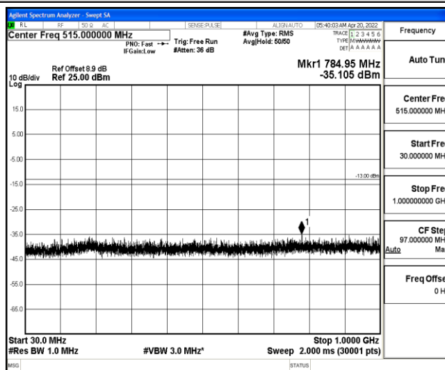
Band25-5MHz-QPSK-26665-1-0-High-30-1000--35.11-PASS
