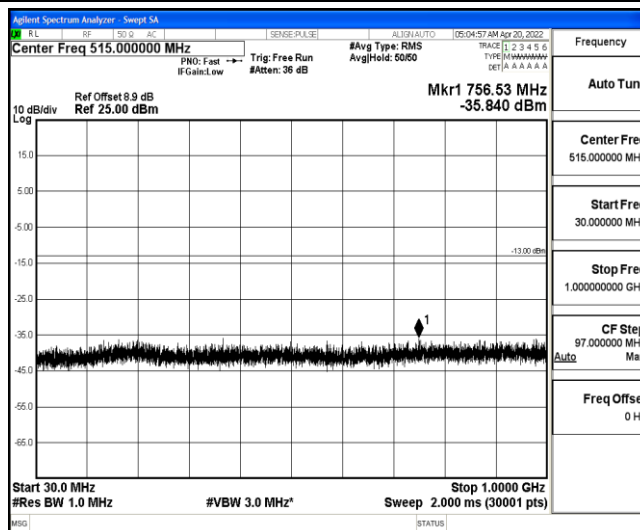
Band25-3MHz-16QAM-26365-1-0-Low-30-1000--35.84-PASS
