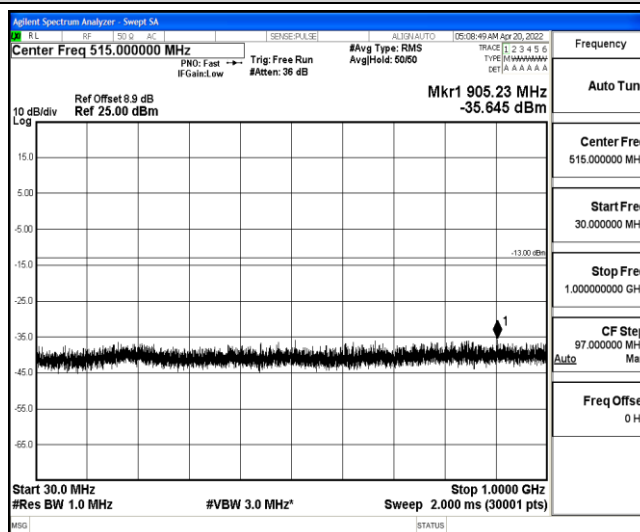
Band25-3MHz-16QAM-26675-1-0-High-30-1000--35.65-PASS
