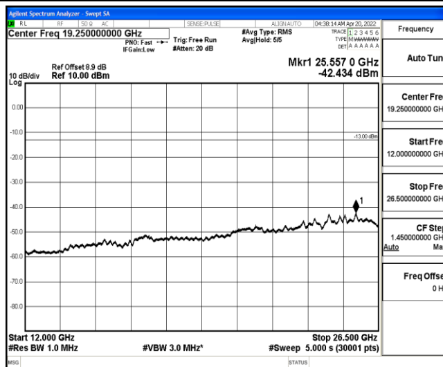
Band25-1.4MHz-QPSK-26365-1-0-Low-12000-26500--42.43-PASS
