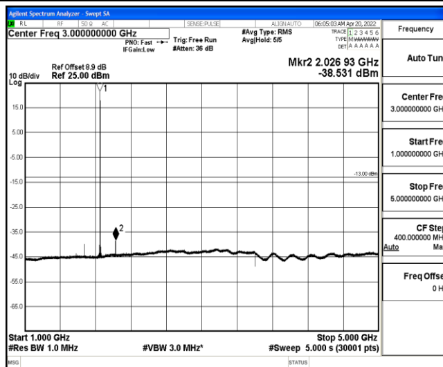
Band25-10MHz-QPSK-26090-1-0-Low-1000-5000--38.53-PASS
