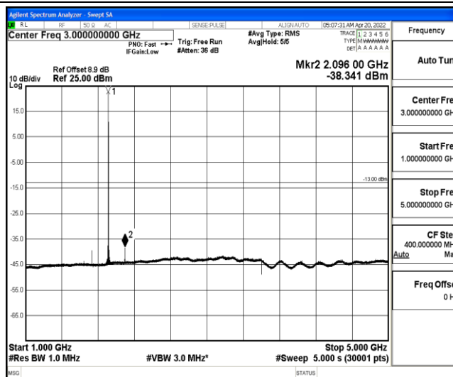
Band25-3MHz-QPSK-26675-1-0-High-1000-5000--38.34-PASS
