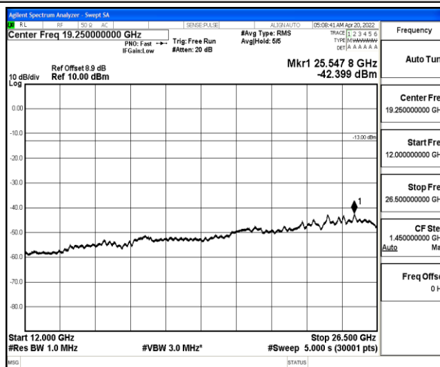
Band25-3MHz-QPSK-26675-1-0-High-12000-26500--42.4-PASS
