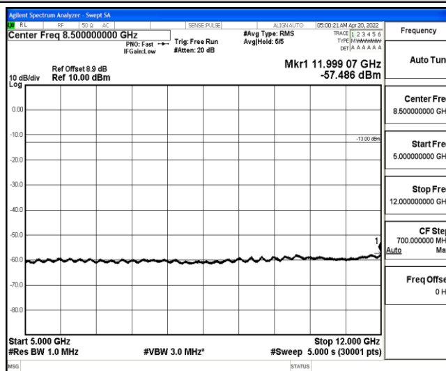
Band25-3MHz-QPSK-26055-1-0-Low-5000-12000--57.49-PASS
