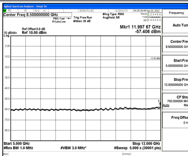
Band25-1.4MHz-16QAM-26047-1-0-Low-5000-12000--57.41-PASS
