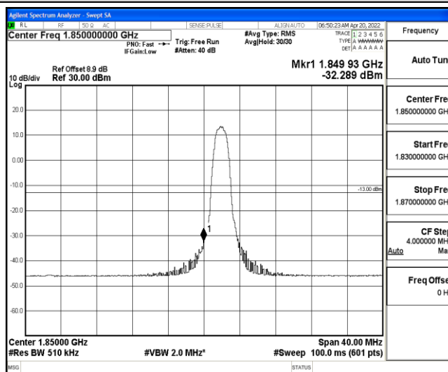
Band25-20MHz-QPSK-26140-6-0-Low--32.29-PASS
