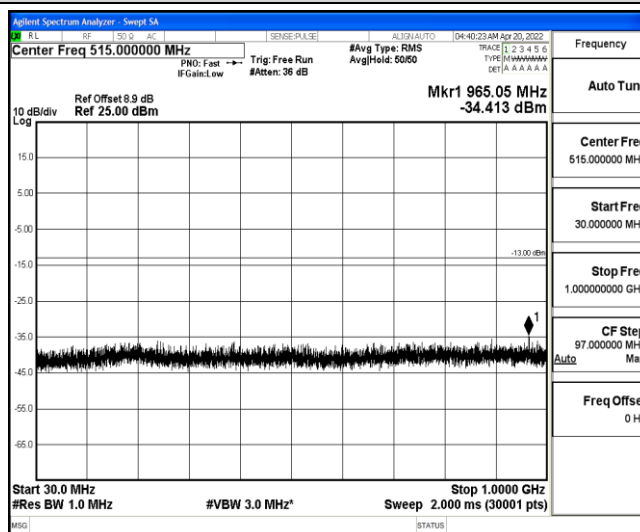
Band25-1.4MHz-QPSK-26683-1-0-High-30-1000--34.41-PASS
