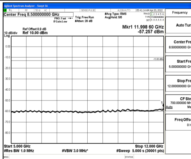
Band25-5MHz-QPSK-26665-1-0-High-5000-12000--57.26-PASS
