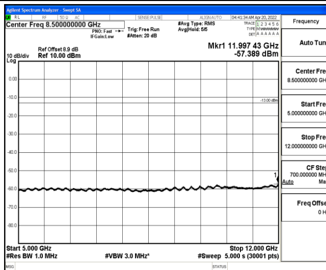
Band25-1.4MHz-QPSK-26683-1-0-High-5000-12000--57.39-PASS
