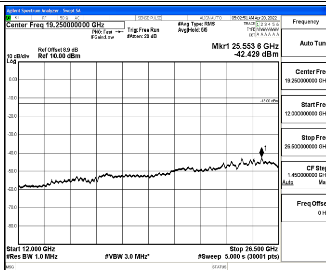
Band25-3MHz-16QAM-26055-1-0-Low-12000-26500--42.43-PASS
