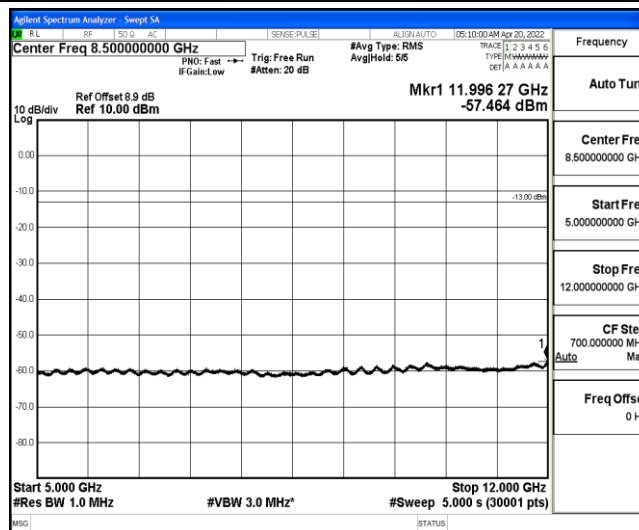
Band25-3MHz-16QAM-26675-1-0-High-5000-12000--57.46-PASS
