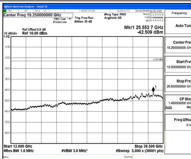
Band25-1.4MHz-QPSK-26683-1-0-High-12000-26500--42.51-PASS
