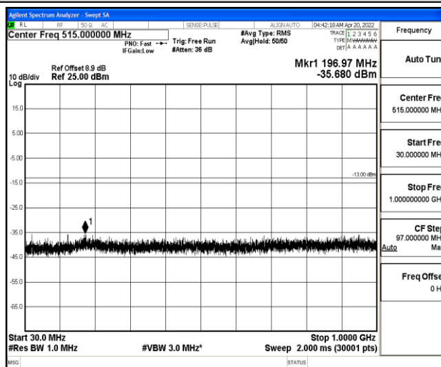
Band25-1.4MHz-16QAM-26683-1-0-High-30-1000--35.68-PASS
