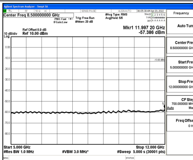
Band25-10MHz-QPSK-26090-1-0-Low-5000-12000--57.39-PASS
