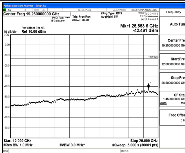
Band25-3MHz-16QAM-26365-1-0-Low-12000-26500--42.46-PASS
