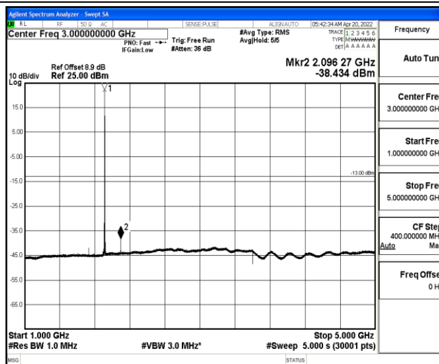
Band25-5MHz-16QAM-26665-1-0-High-1000-5000--38.43-PASS
