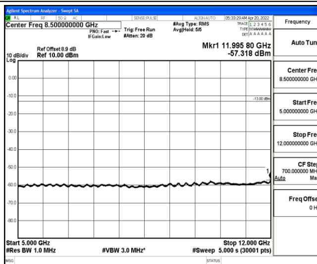
Band25-5MHz-QPSK-26065-1-0-Low-5000-12000--57.32-PASS
