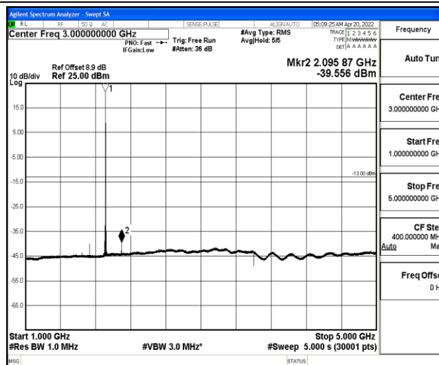
Band25-3MHz-16QAM-26675-1-0-High-1000-5000--39.56-PASS
