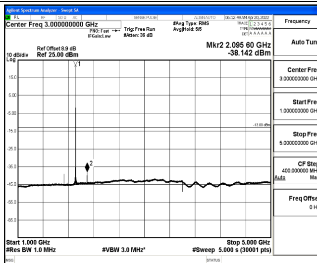
Band25-10MHz-QPSK-26640-1-0-High-1000-5000--38.14-PASS
