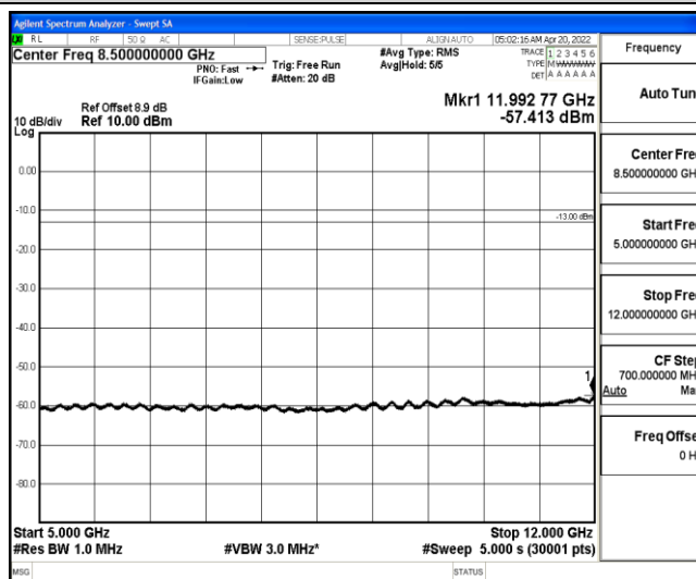
Band25-3MHz-16QAM-26055-1-0-Low-5000-12000--57.41-PASS
