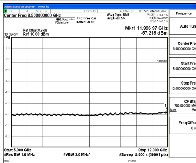
Band25-5MHz-16QAM-26065-1-0-Low-5000-12000--57.22-PASS
