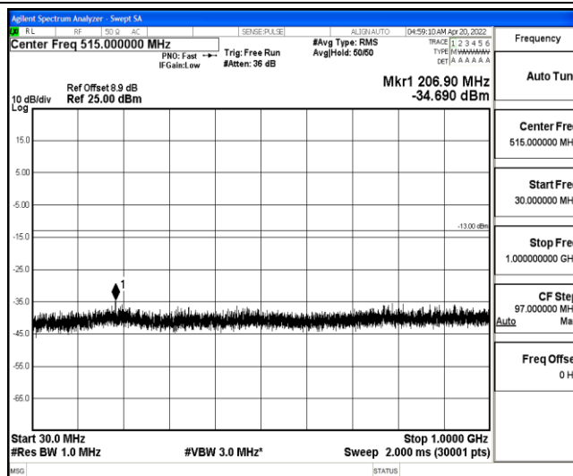
Band25-3MHz-QPSK-26055-1-0-Low-30-1000--34.69-PASS
