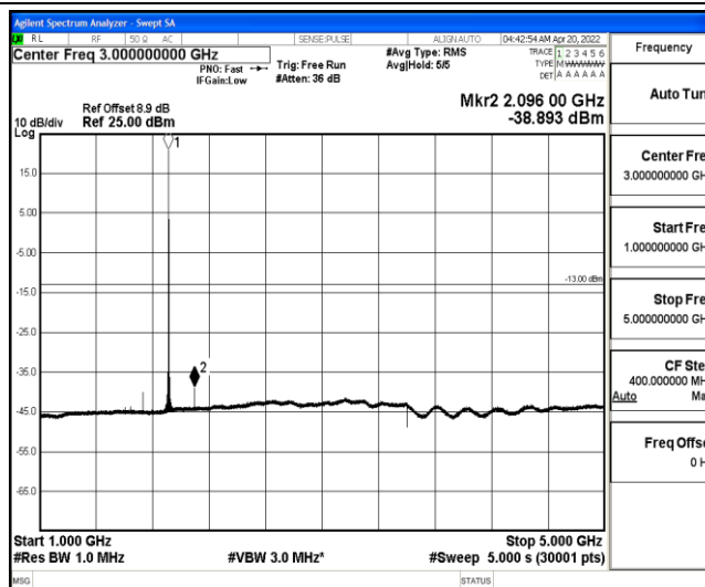
Band25-1.4MHz-16QAM-26683-1-0-High-1000-5000--38.89-PASS
