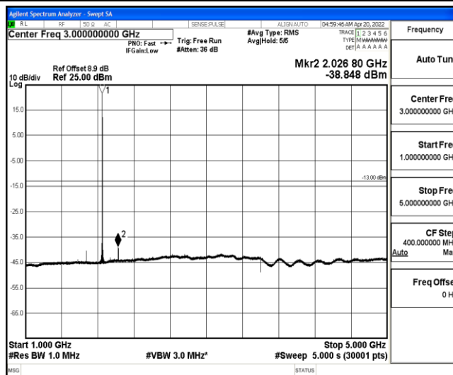
Band25-3MHz-QPSK-26055-1-0-Low-1000-5000--38.85-PASS
