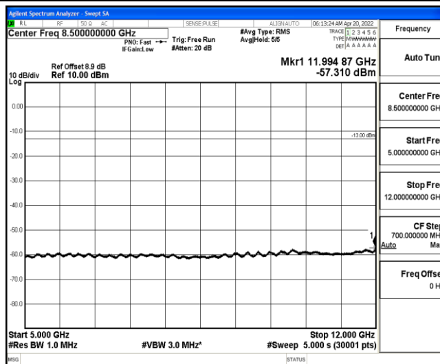
Band25-10MHz-QPSK-26640-1-0-High-5000-12000--57.31-PASS
