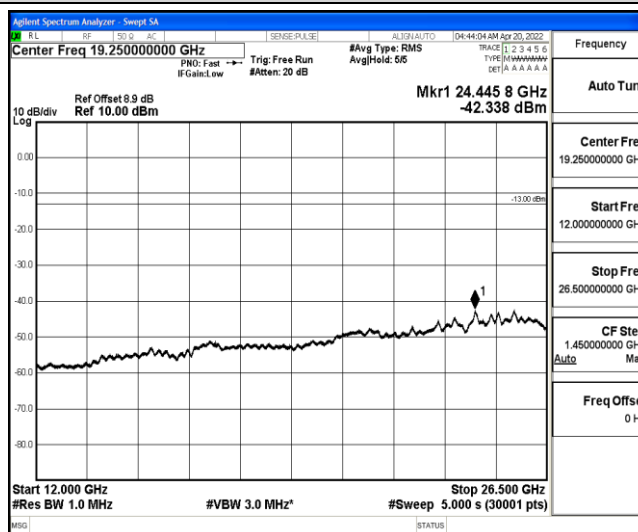
Band25-1.4MHz-16QAM-26683-1-0-High-12000-26500--42.34-PASS
