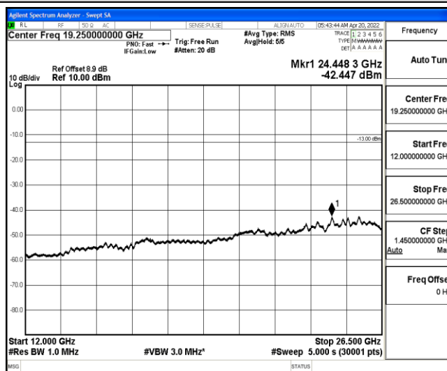
Band25-5MHz-16QAM-26665-1-0-High-12000-26500--42.45-PASS
