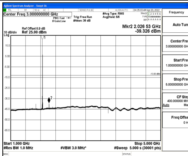
Band25-1.4MHz-16QAM-26047-1-0-Low-1000-5000--39.33-PASS
