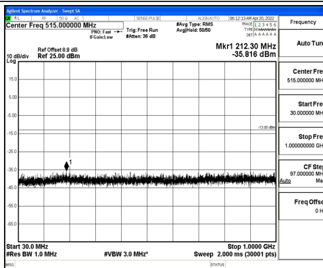
Band25-10MHz-QPSK-26640-1-0-High-30-1000--35.82-PASS
