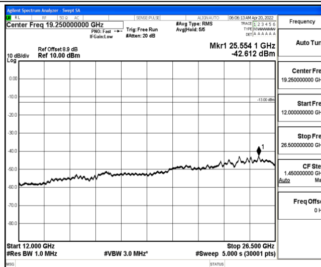
Band25-10MHz-QPSK-26090-1-0-Low-12000-26500--42.61-PASS
