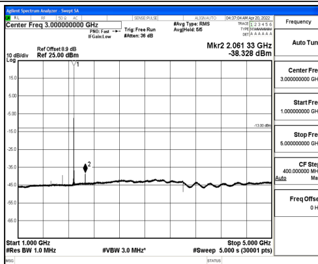
Band25-1.4MHz-QPSK-26365-1-0-Low-1000-5000--38.33-PASS
