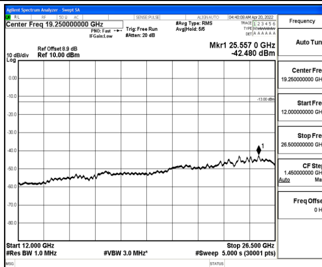
Band25-1.4MHz-16QAM-26365-1-0-Low-12000-26500--42.48-PASS
