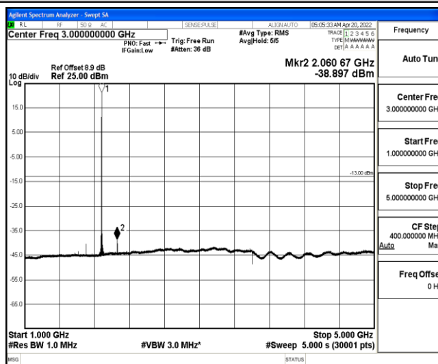
Band25-3MHz-16QAM-26365-1-0-Low-1000-5000--38.9-PASS
