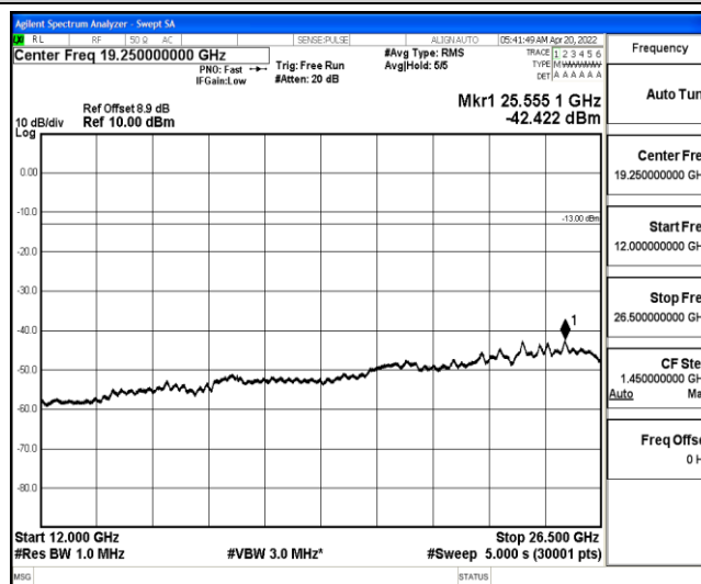
Band25-5MHz-QPSK-26665-1-0-High-12000-26500--42.42-PASS
