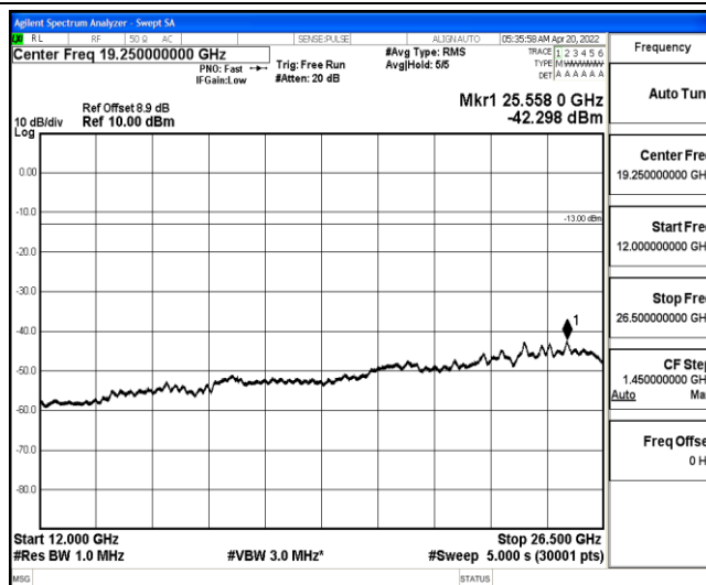
Band25-5MHz-16QAM-26065-1-0-Low-12000-26500--42.3-PASS
