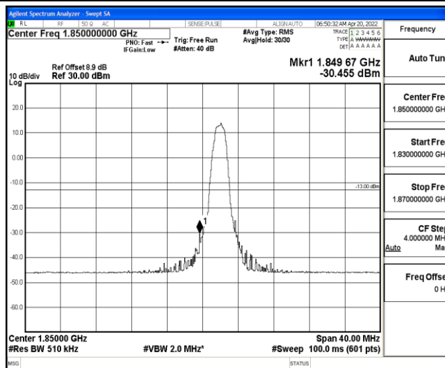
Band25-20MHz-16QAM-26140-6-0-Low--30.45-PASS
