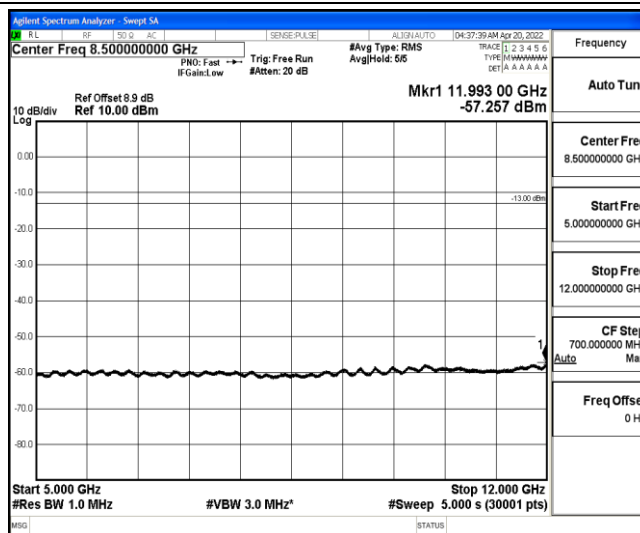
Band25-1.4MHz-QPSK-26365-1-0-Low-5000-12000--57.26-PASS
