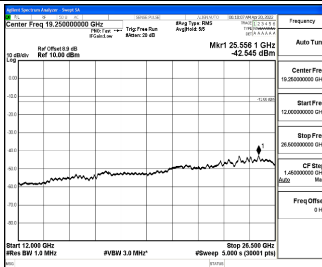
Band25-10MHz-QPSK-26365-1-0-Low-12000-26500--42.55-PASS
