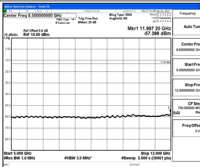
Band25-5MHz-QPSK-26365-1-0-Low-5000-12000--57.39-PASS
