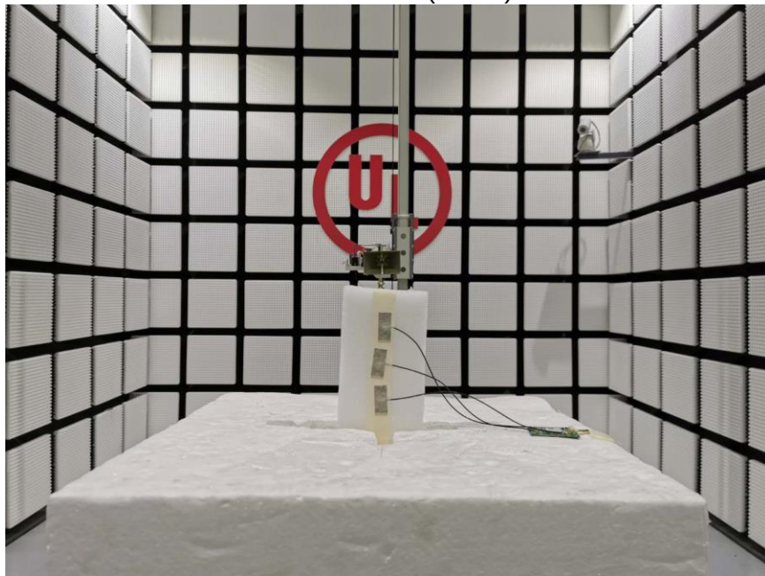
MEASUREMENT POSITION (Z axis) -ANT WCT5H-20
