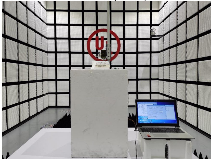
MEASUREMENT POSITION (TESTED) -ANT WCT5H-20
