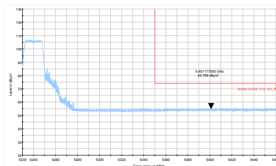
SISO 802.11a-Channel 48: Average
