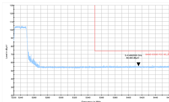
MIMO 802.11ac VHT20 -Channel 48: Average
