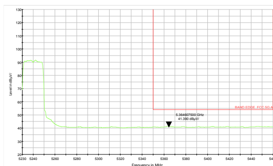
MIMO 802.11ac VHT20 -Channel 48: Average
