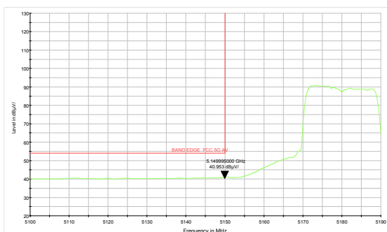
MIMO 802.11ac VHT20-Channel 36: Average
