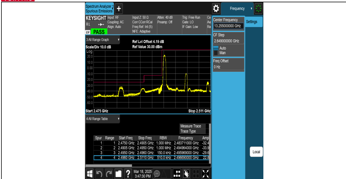
Band41-15MHz-16QAM-39725-27RB#0-PASS
