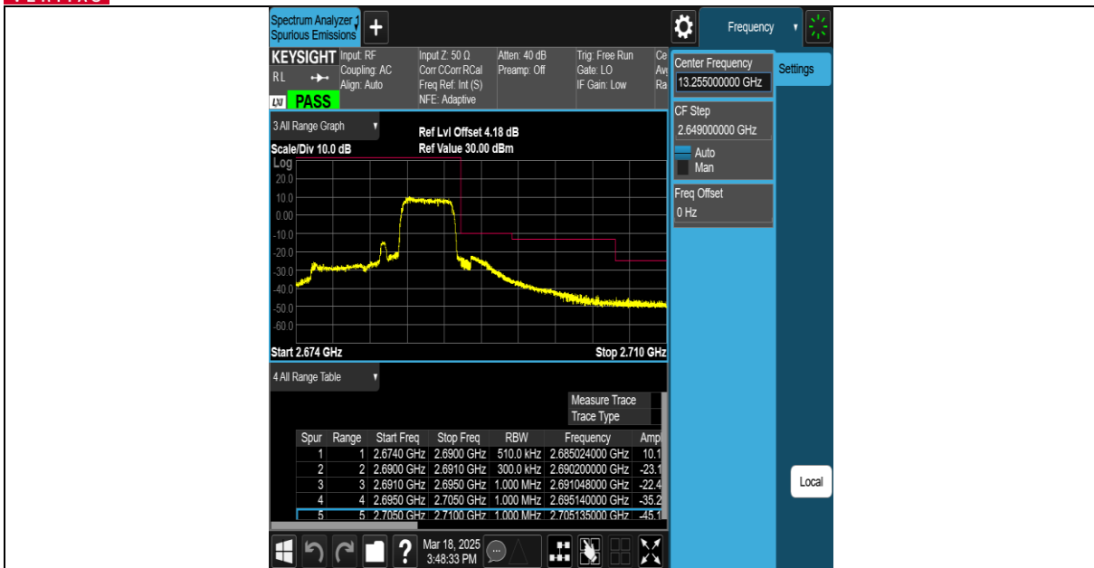
Band41-15MHz-16QAM-41515-1RB#74-PASS
