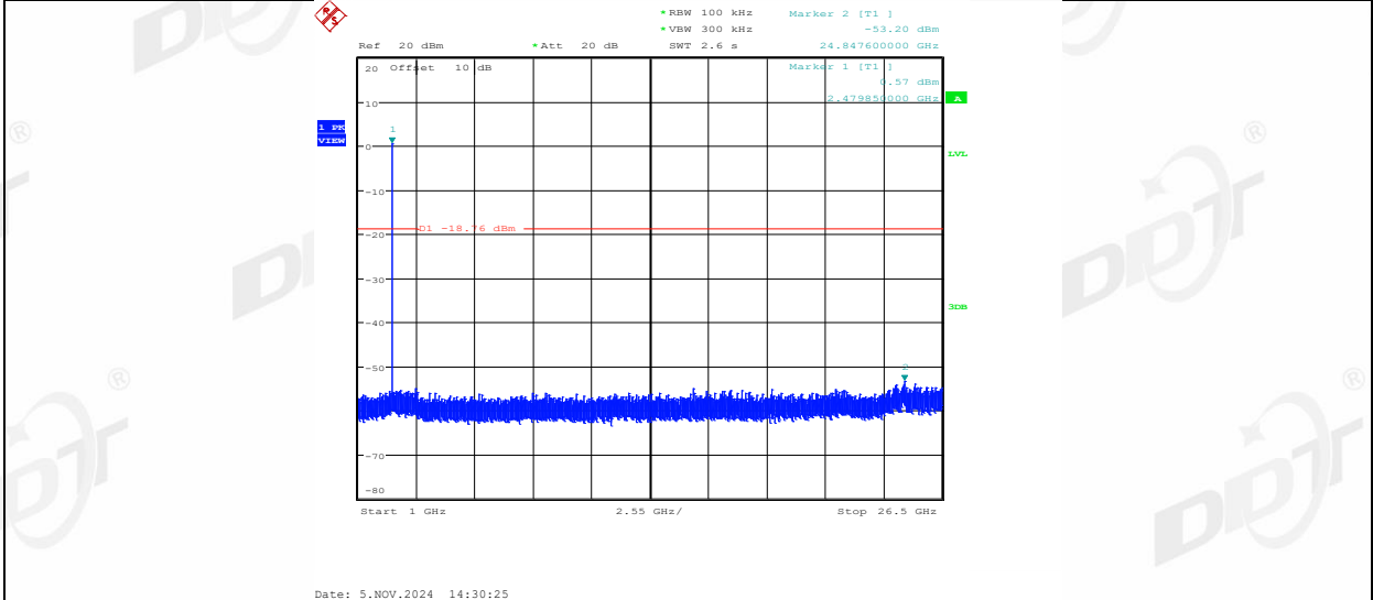
2DH5_Ant1_2402_0~Reference
