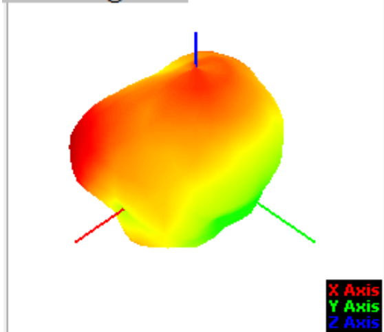
2340.00MHz@T45P45
