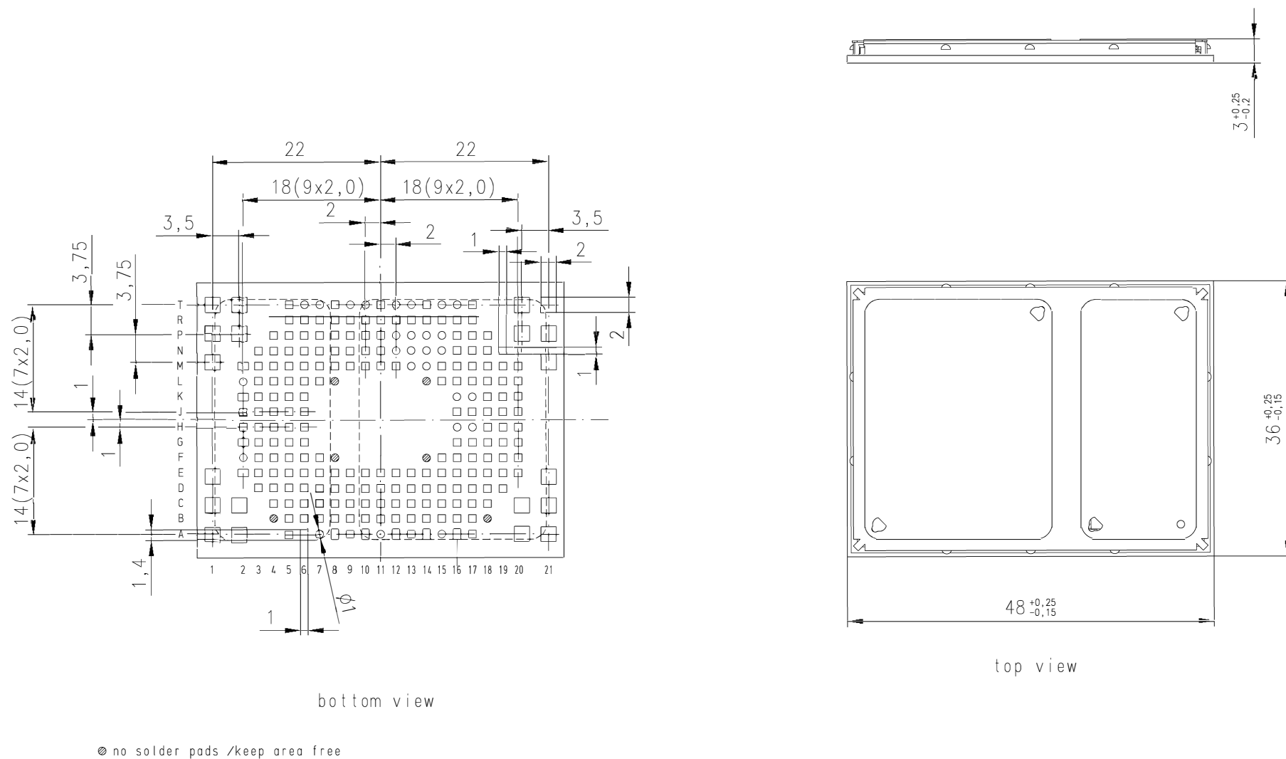
Figure 15: Dimensions of ALAS66A (all dimensions in mm)
