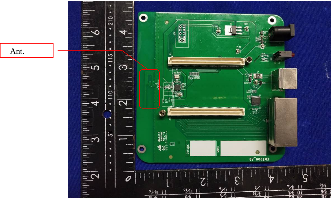
Solder Board-Component View 1
