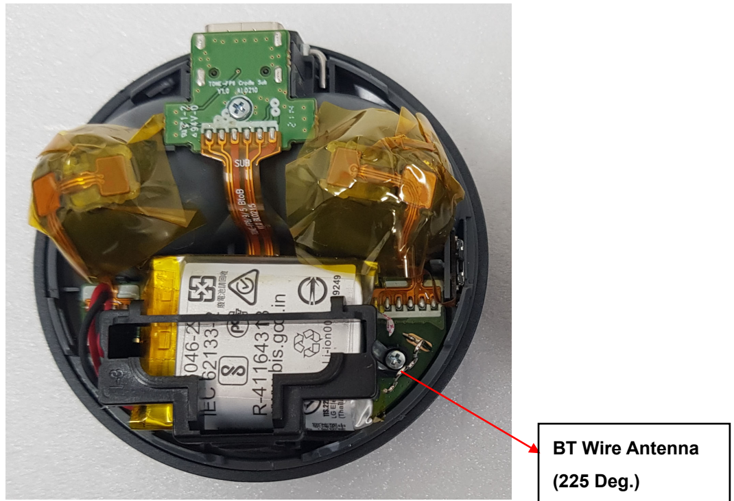
Figure F-1 Antenna Location (Rear Side View)
