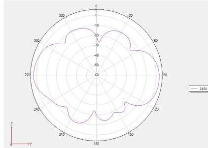
Phi =90 freq=2450MHz
