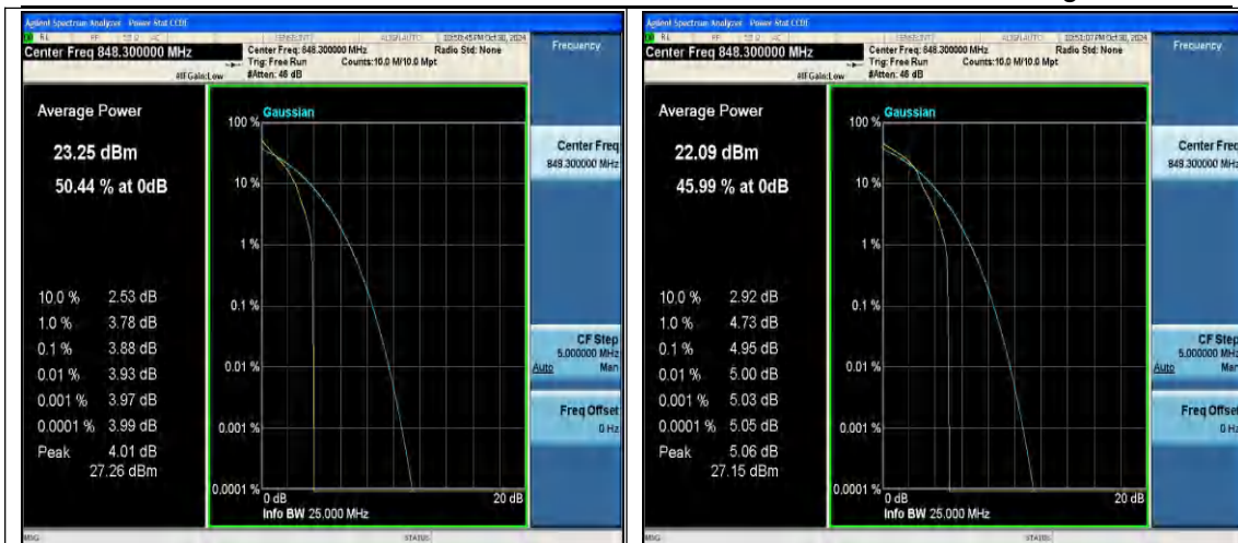
26(824-849)-1.4MHz-QPSK-27033-1RB#0-PASS
