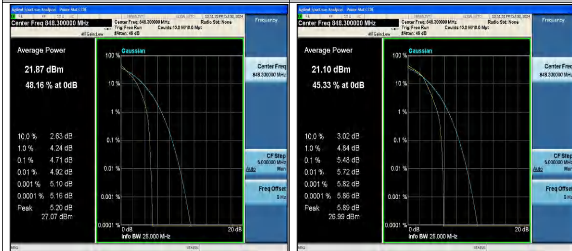
26(824-849)-1.4MHz-QPSK-27033-6RB#0-PASS
