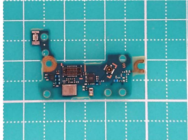
Internal Sub-PWB (Rear-side)
