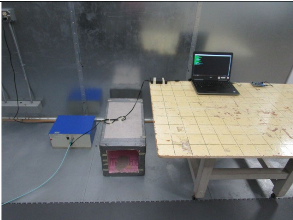
AC Line Conducted Emissions
