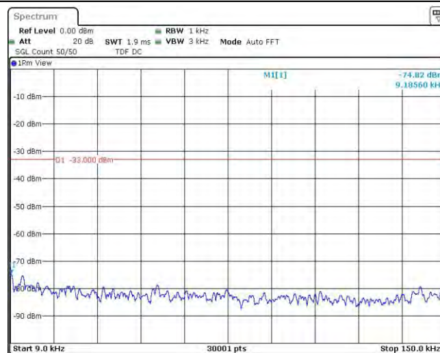
Band5-4132-3-10000~18000MHz
