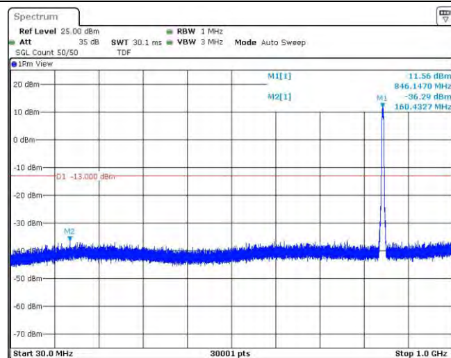
Band5-4233-3-30~1000MHz
