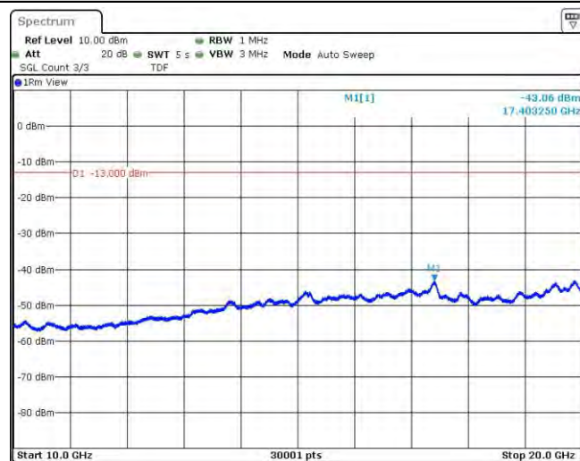
Band4-1513-1-10000~20000MHz
