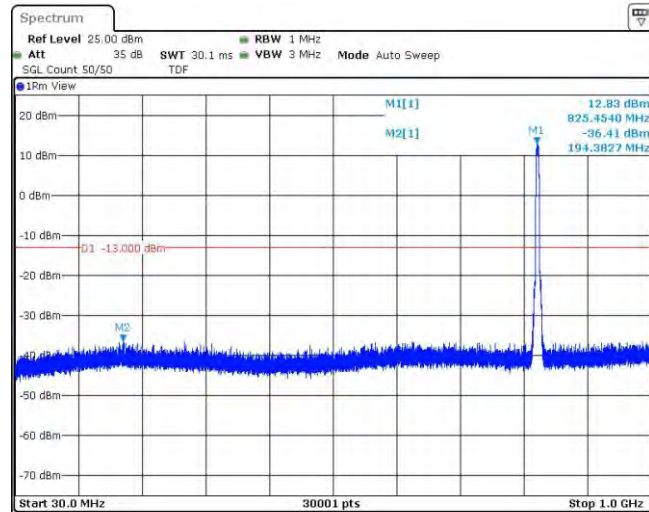
Band5-4132-1-1000~3000MHz
