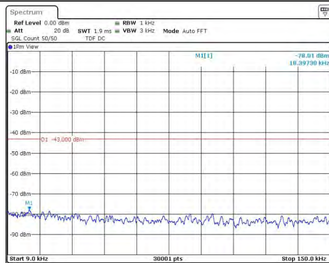
Band4-1413-3-0.009~0.15MHz
