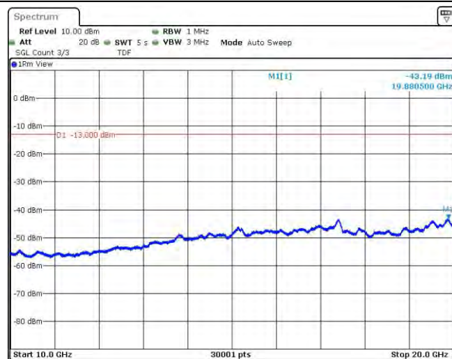
Band2-9400-3-10000~20000MHz
