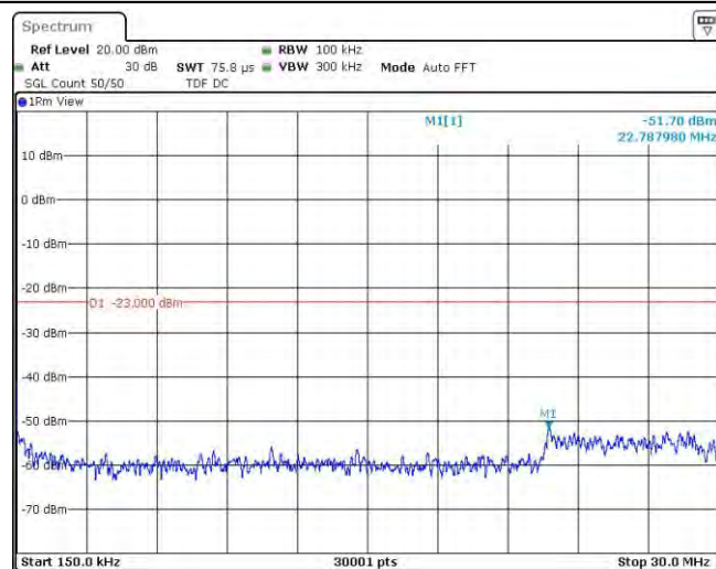
Band4-1513-2-0.15~30MHz
