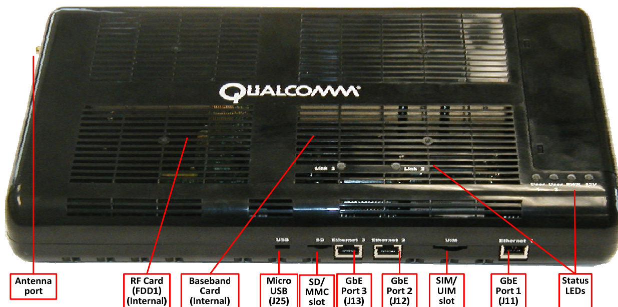
Figure 2.1 MTP9900 LAA external ports
