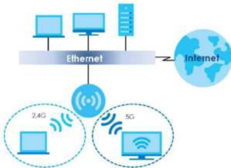
Figure 6 Dual-Radio Application
