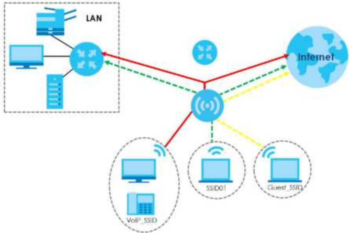
Figure 5 Multiple BSSs
