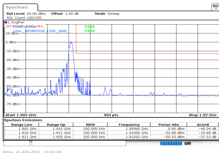
n2_5MHz_15kHz_1907.5MHz_DFT-s-OFDM QPSK_RB1@24
