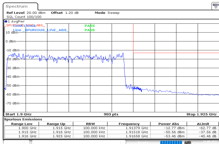
n25_15MHz_15kHz_1907.5MHz_DFT-s-OFDM QPSK_RB75@0
