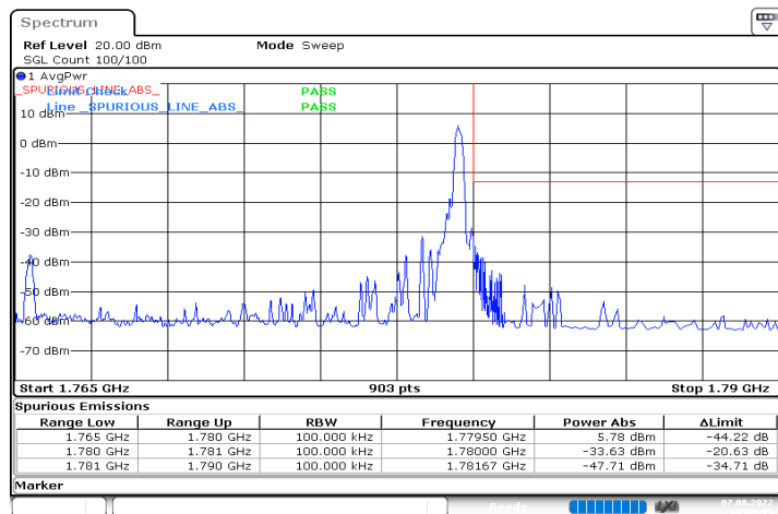
DC_12A_n66A_10MHz|15MHz_15kHz_707.5MHz|1772.5MHz_ DFT-s-OFDM QPSK_RB0|RB1@78
