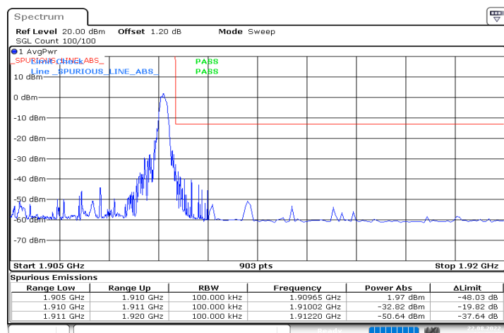
n2_5MHz_15kHz_1907.5MHz_DFT-s-OFDM QPSK_RB1@24
