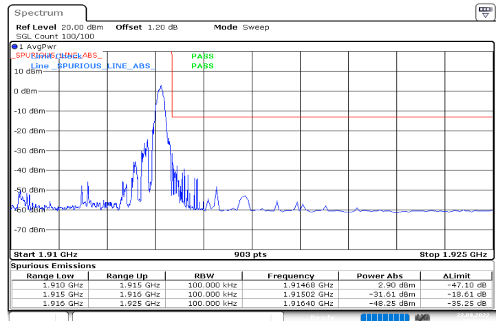
n25_5MHz_15kHz_1912.5MHz_DFT-s-OFDM QPSK_RB1@24
