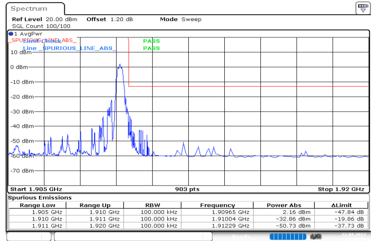
n2_5MHz_15kHz_1907.5MHz_DFT-s-OFDM QPSK_RB1@24
