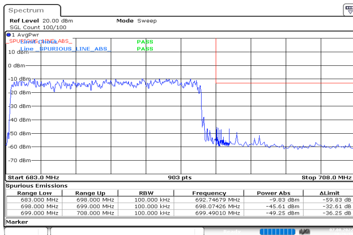
DC_2A_n71A_10MHz|15MHz_15kHz_1880MHz|690.5MHz_D FT-s-OFDM QPSK_RB0|RB75@0
