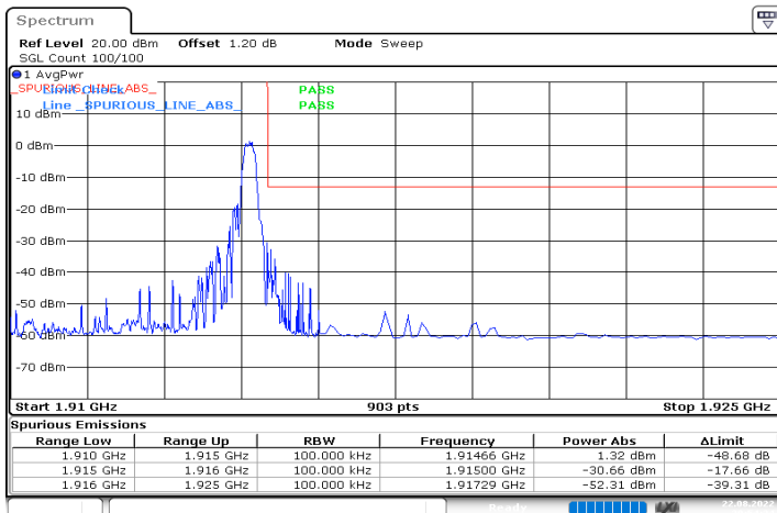
n25_5MHz_15kHz_1912.5MHz_DFT-s-OFDM QPSK_RB1@24
