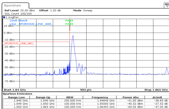
n25_15MHz_15kHz_1857.5MHz_DFT-s-OFDM QPSK_RB1@0
