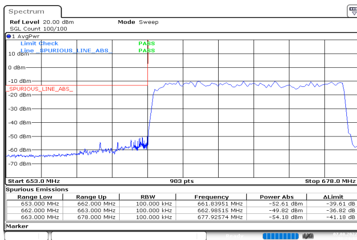
DC_2A_n71A_10MHz|15MHz_15kHz_1880MHz|670.5MHz_D FT-s-OFDM QPSK_RB0|RB75@0
