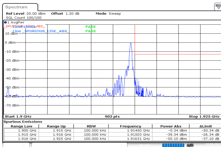
n25_15MHz_15kHz_1907.5MHz_DFT-s-OFDM QPSK_RB1@78
