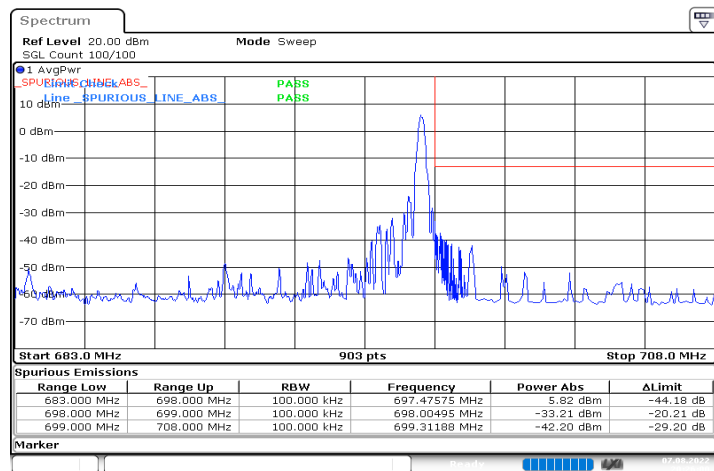
DC_2A_n71A_10MHz|15MHz_15kHz_1880MHz|690.5MHz_D FT-s-OFDM QPSK_RB0|RB1@78
