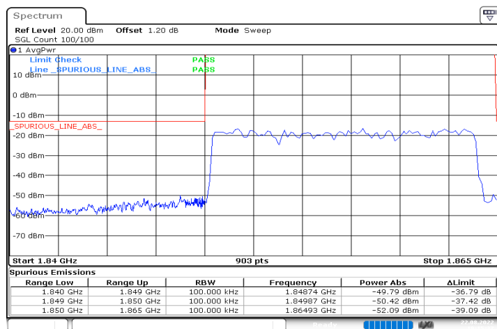
n25_15MHz_15kHz_1857.5MHz_DFT-s-OFDM QPSK_RB75@0
