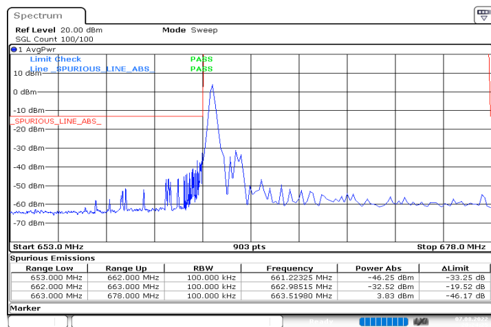
DC_2A_n71A_10MHz|15MHz_15kHz_1880MHz|670.5MHz_D FT-s-OFDM QPSK_RB0|RB1@0
