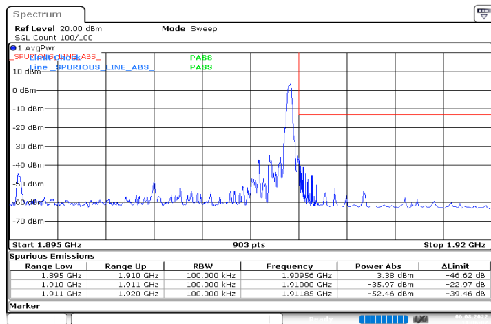
DC_12A_n2A_10MHz|15MHz_15kHz_707.5MHz|1902.5MHz_ DFT-s-OFDM QPSK_RB0|RB1@78
