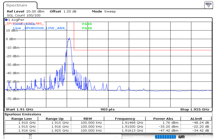
n25_5MHz_15kHz_1912.5MHz_DFT-s-OFDM QPSK_RB1@24
