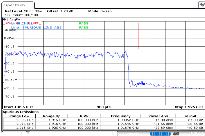
n25_20MHz_15kHz_1905MHz_DFT-s-OFDM QPSK_RB100@0
