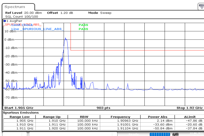
n2_5MHz_15kHz_1907.5MHz_DFT-s-OFDM QPSK_RB1@24
