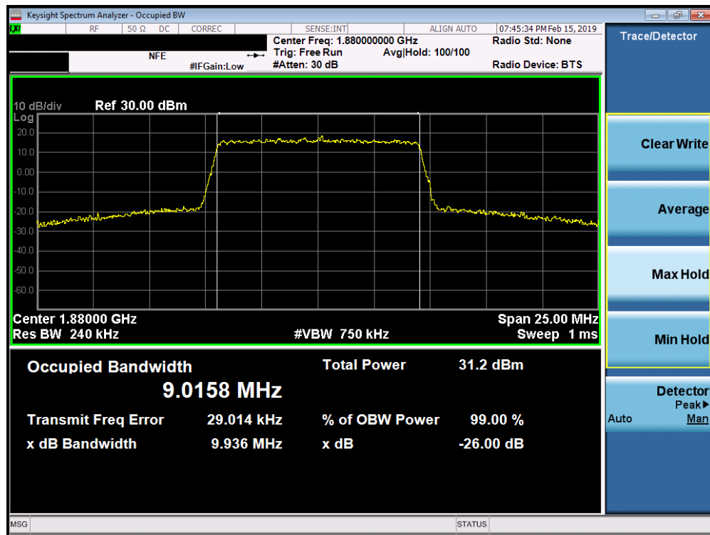
Plot 7-46. Occupied Bandwidth Plot (Band 25/2 - 10.0MHz 16-QAM - Full RB Configuration)
