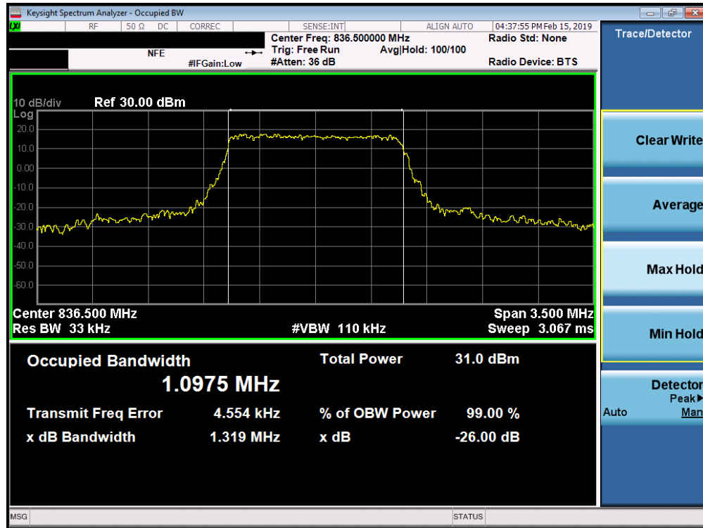
Plot 7-17. Occupied Bandwidth Plot (Band 26/5 - 1.4MHz QPSK - Full RB Configuration)
