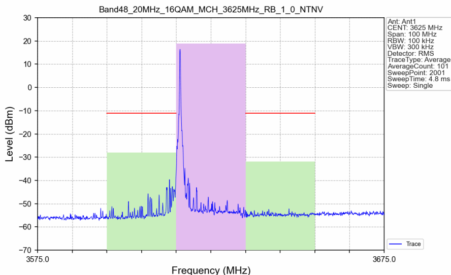
Band48_20MHz_16QAM_MCH_3625MHz_RB_1_0_NTNV
