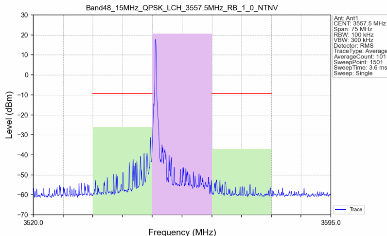
Band48_15MHz_QPSK_LCH_3557.5MHz_RB_1_0_NTNV
