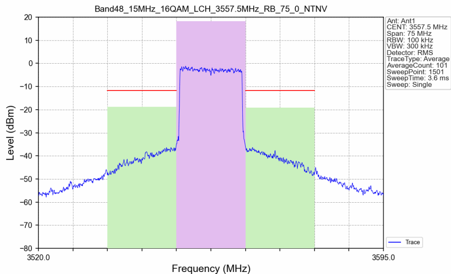
Band48_15MHz_16QAM_LCH_3557.5MHz_RB_75_0_NTNV
