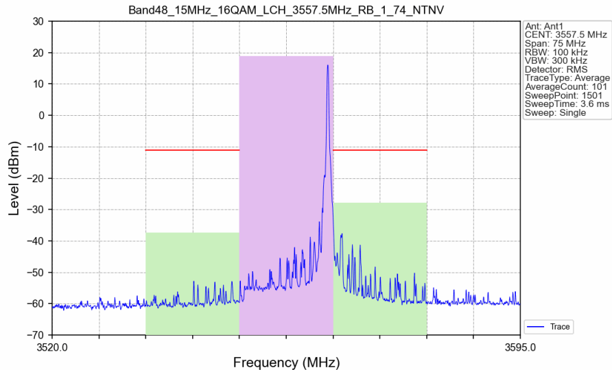
Band48_15MHz_16QAM_LCH_3557.5MHz_RB_1_74_NTNV
