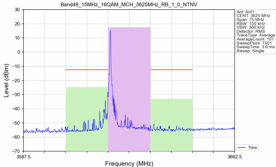
Band48_15MHz_16QAM_MCH_3625MHz_RB_1_0_NTNV
