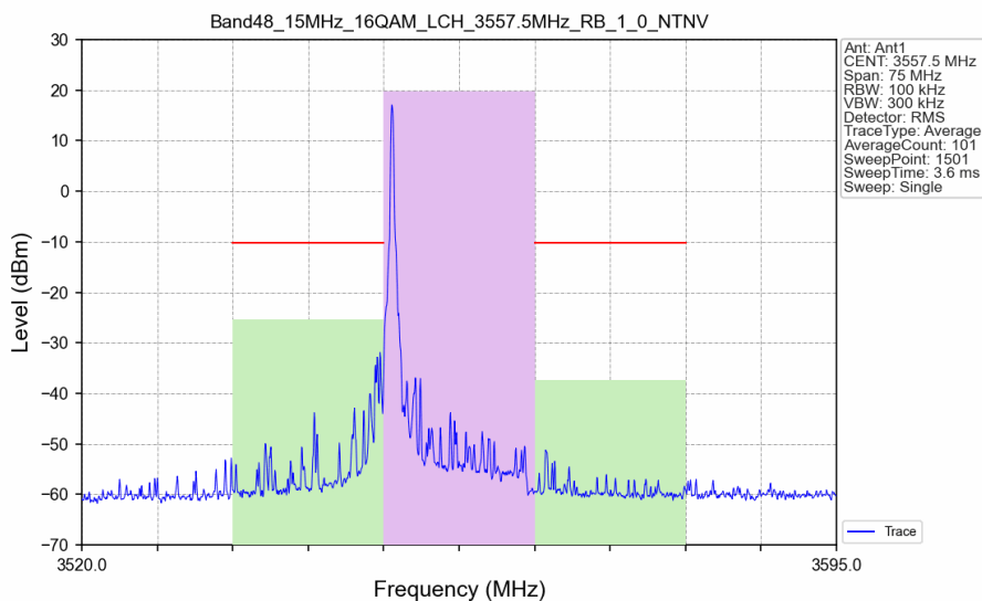
Band48_15MHz_16QAM_LCH_3557.5MHz_RB_1_0_NTNV
