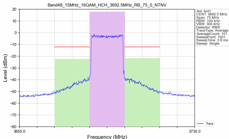
Band48_15MHz_16QAM_HCH_3692.5MHz_RB_75_0_NTNV
