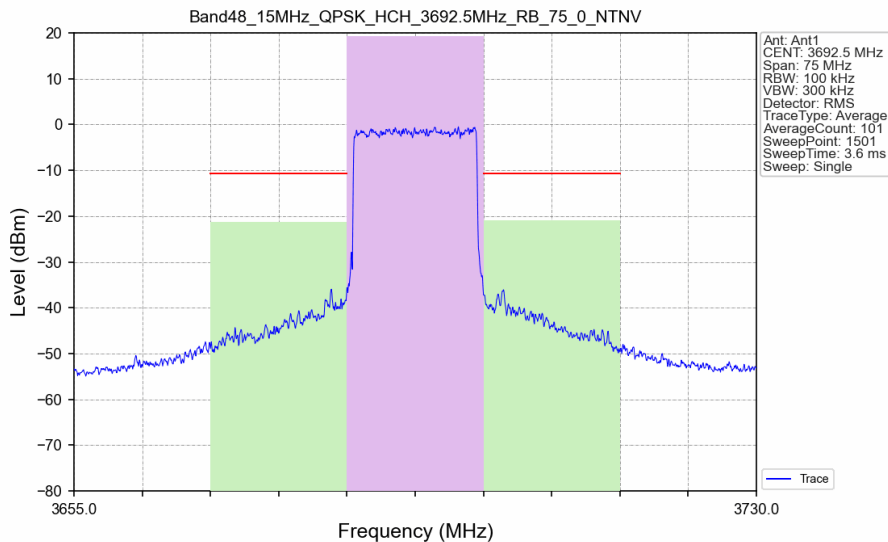
Band48_15MHz_QPSK_HCH_3692.5MHz_RB_75_0_NTNV
