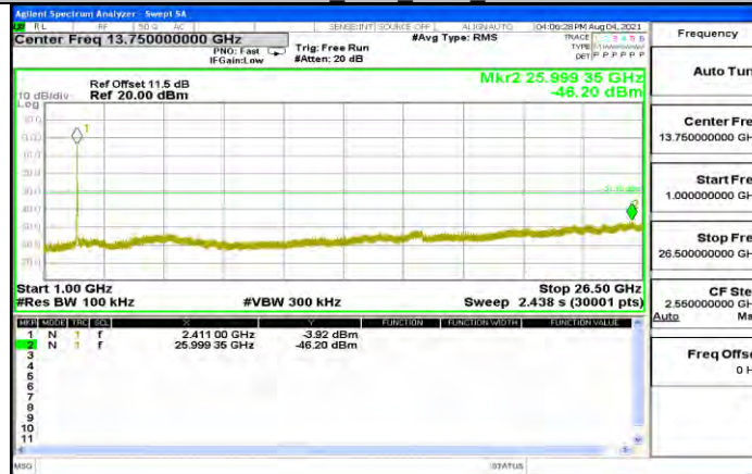
11N20SISO_Ant1_2412_1000~26500
