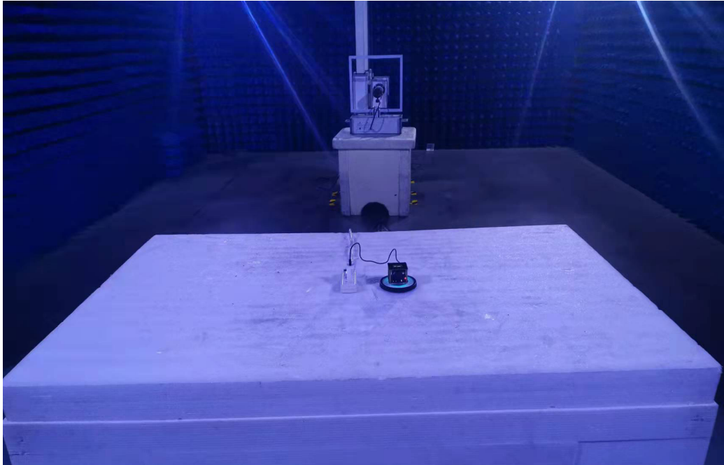
Photo of Radiated Emission Measurement (Below 1GHz)
