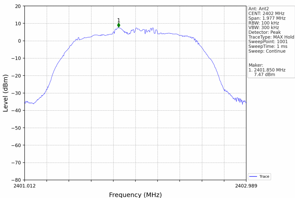
Pi/4DQPSK_2DH5_LCH_2402MHz_Ant2_NTNV
