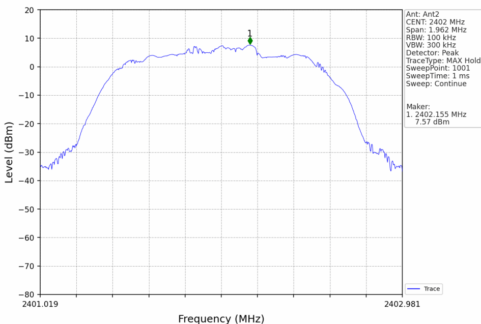
8DPSK_3DH5_LCH_2402MHz_Ant2_NTNV
