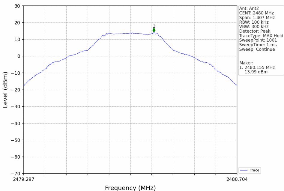
GFSK_DH5_HCH_2480MHz_Ant2_NTNV
